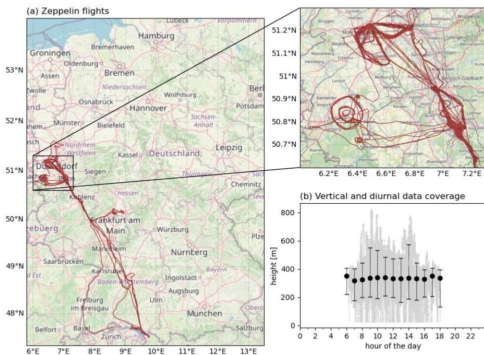
Figure 1: (a). The Zepplin flight tracks over Germany (© OpenStreetMap contributors 2021. Distributed under the Open Data Commons Open Database License (ODbL) v1.0.) and (b). their vertical and diurnal coverage in UTC.
