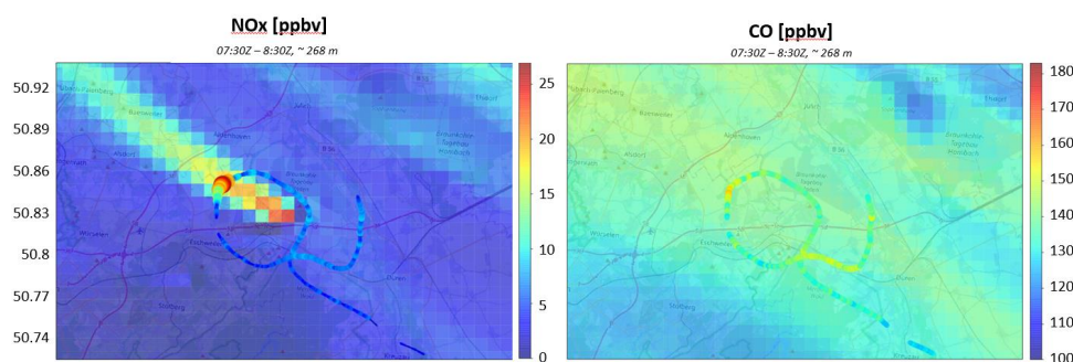
355 Figure 7: Evolution of industrial plume emissions of NO x and CO based on the EURAD-IM model overlaid by the field-derived Zeppelin observations.
