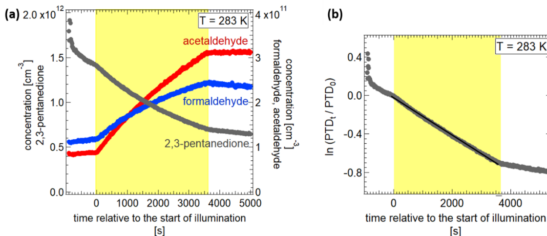
315 Figure 5: a) Concentrations of 2,3-pentanedione, acetaldehyde and formaldehyde during the experiment. b) Logarithmic depiction of the 2,3-pentanedione (PTD) concentration to calculate the photolysis frequency.
