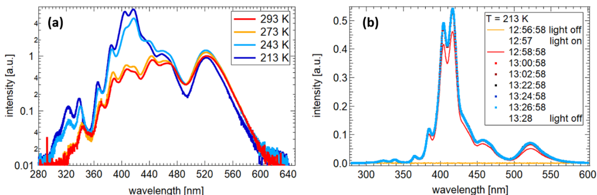
230 Figure 3: a) Spectra taken with the UV-Vis spectrometer at the bottom of the chamber at 4 different temperatures. The electrical settings for the LEDs for each temperature are different. In addition to the emission changes of the LEDs due to the temperature variation, this leads to different spectral distributions for each temperature. b) Spectra taken with the UV-Vis spectrometer at the bottom of the chamber over a time period of 30 min.
