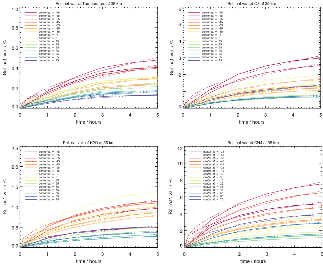
Figure 3. Natural variability as function of time separation for temperature, O 3 , CH 4 , and H 2 O in BASCOE model (solid lines) and proposed parametrization (dashed lines).
