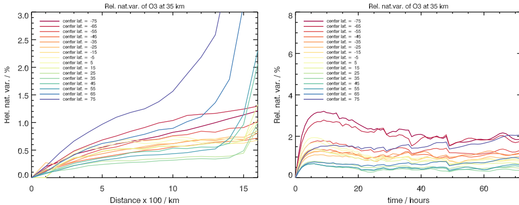
Figure 1. Left panel : natural variability of O_3 at 35 km altitude as function of horizontal distance in BASCOE model. Right panel : natural variability of O_3 at 35 km altitude as function of time separation in BASCOE model.
