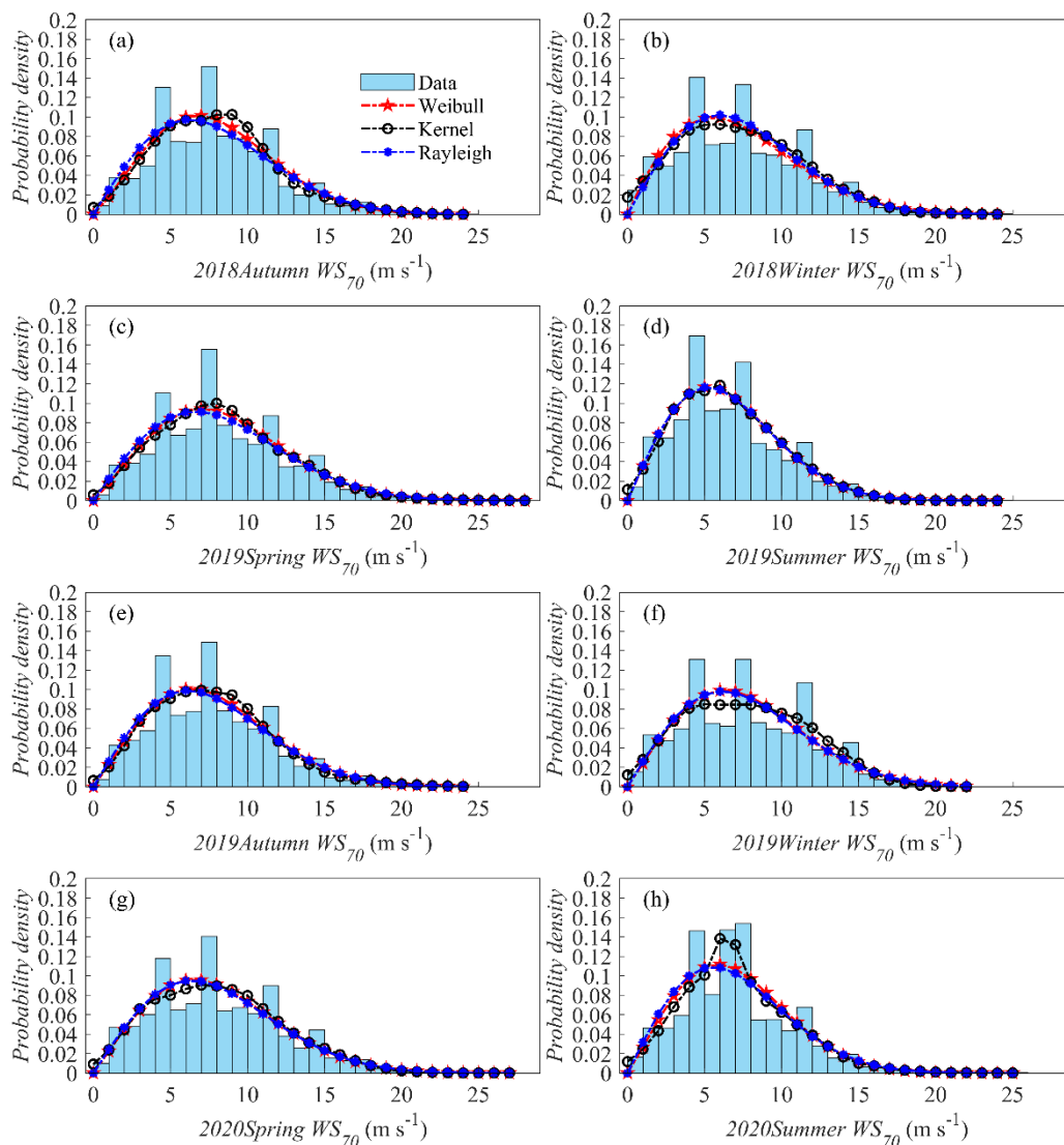
465 Figure 4: Frequency density histogram of wind speed at 70-m height from autumn 2018 to summer 2020; the probability density curve obtained by fitting the Weibull, kernel, and Rayleigh distribution functions to the original data. (a), (b), (c), (d), (e), (f), and (h) represent each season, respectively.
