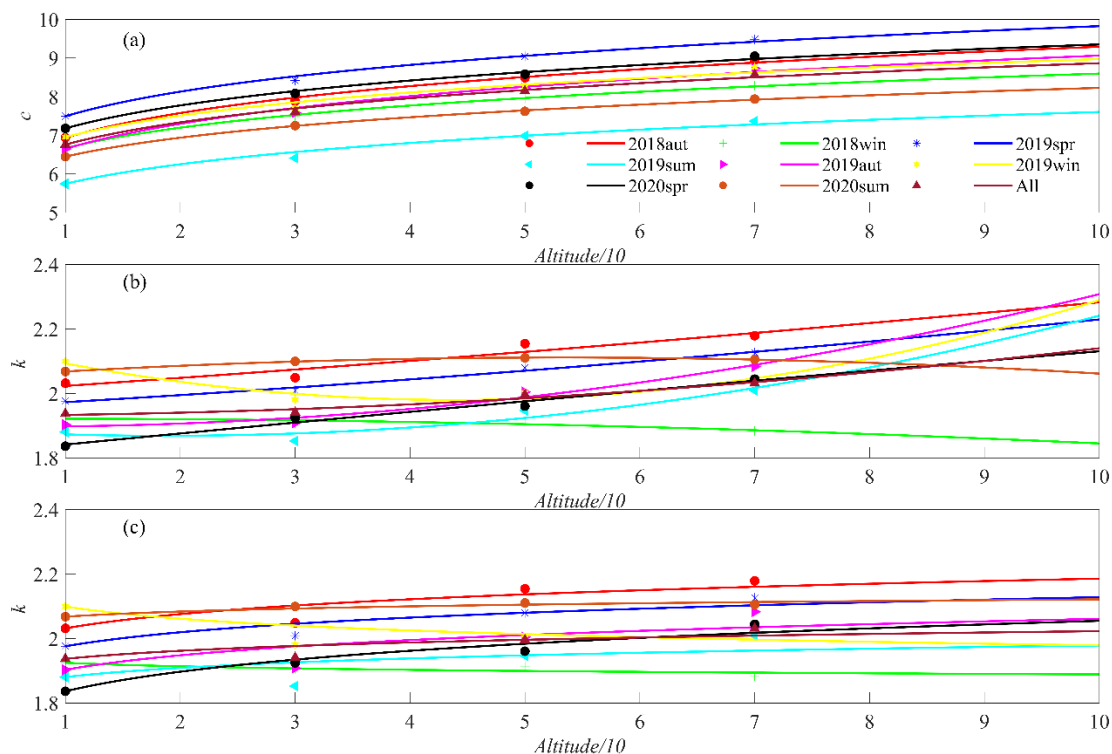
Figure 6: (a) The characteristic variation of scale factor c with height based on equation (2.12). The characteristic variation of shape factor k with height based on (b) equation (2.13) and (c) equation (2.14).
