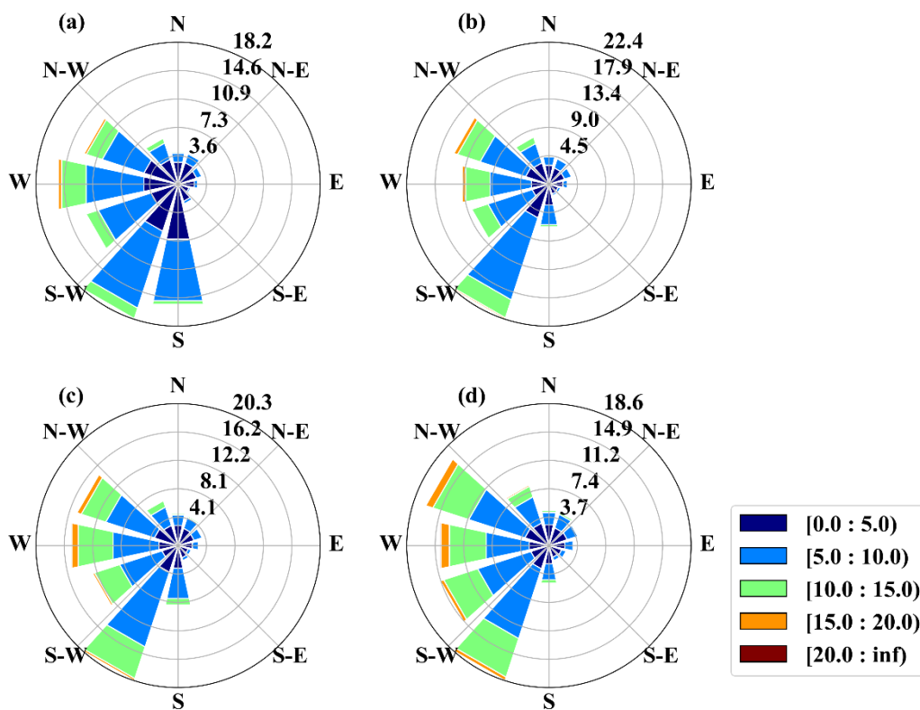
460 Figure 3: The distribution of the high-altitude wind speed and direction rose diagram of the wind measurement tower of the Ningyuanbailiutu wind farm from September 2018 to August 2020. (a), (b), (c), and (d) represent 10 m, 30 m, 50 m, and 70 m in altitude, respectively.
