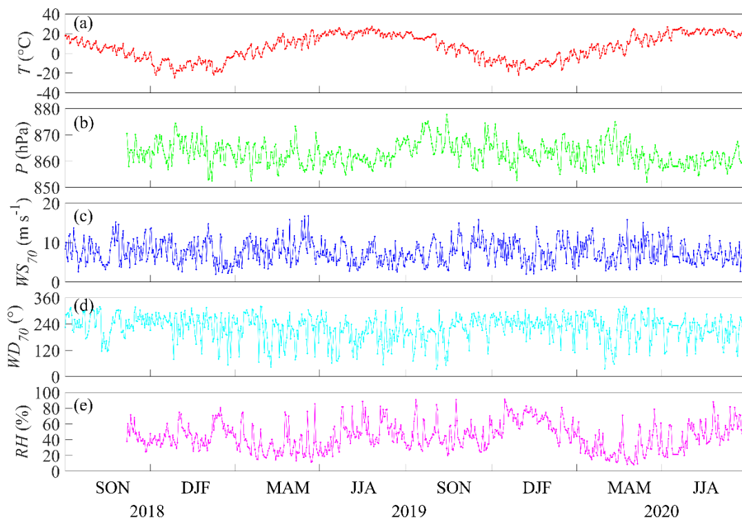
455 Figure 2: (a), (b), (c), (d), and (e) represent daily average temperature ( ^{\circ}\text{C} ), daily average pressure (hPa), 70-m daily average wind speed (m/s), 70-m daily average wind direction ( ^{\circ} ), and the average daily relative humidity (%), respectively.
