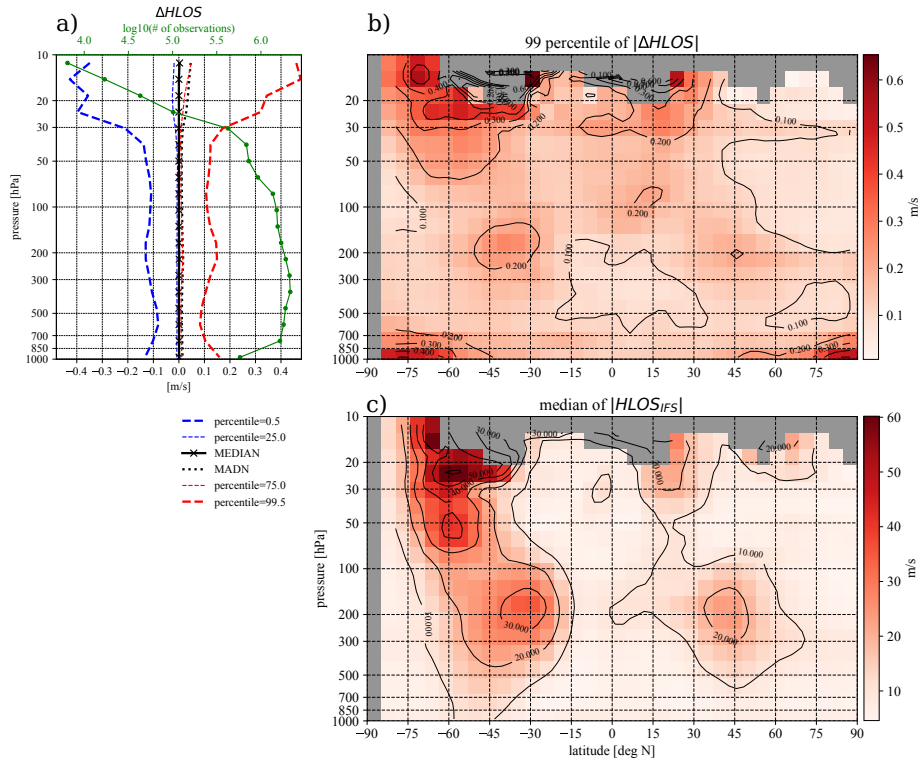
Figure 7. The \Delta HLOS statistics related to the dataset presented in Fig. 3-5 and computed by Eq. 3. (a) The spatial and temporal statistics are displayed as a function of pressure showing the median, madn and several percentiles. (solid green) The number of available data at specific pressure layers. (b) 99th percentile of |\Delta HLOS| and (c) the median of the |HLOS|_{IFS} from the operational L2B output files.
