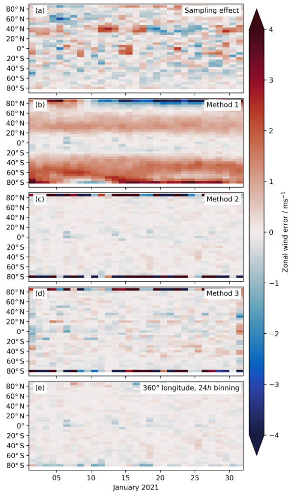
535 Figure 9: Absolute errors in the daily zonal mean zonal wind calculation for January 2021. Panel (a) shows errors originating in the Aeolus sampling, panels (b-d) the errors when using the three conversion methods, respectively, and panel (e) the errors for Method 3, but with a slightly different collocation/binning algorithm. The sampling bias shown in Panel (a) has been removed from the error estimates in panels (b-e).
