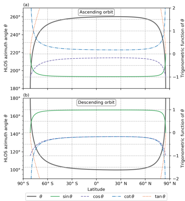
500 Figure 3: Aeolus azimuth angle and its trigonometric functions with respect to latitude for ascending (a) and descending (b) orbits.
