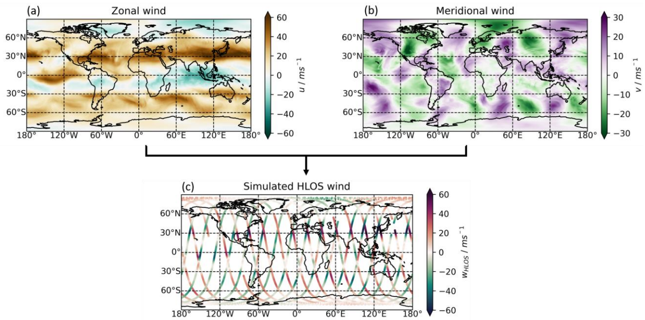
510 Figure 5: Simulation of Aeolus HLOS wind from ERA5 model data. Panels (a) and (b) show the zonal and meridional wind fields from ERA5 on 15 January 2021, 12 UTC for an altitude of 15 km. Panel (c) shows the simulated Aeolus HLOS wind along track on 15 January 2021. This simulated Aeolus HLOS wind is constructed through trilinear interpolation of hourly ERA5 zonal and meridional wind fields onto the exact times and locations of real Aeolus observations, followed by a conversion into simulated Aeolus HLOS wind following Eq. (3).
