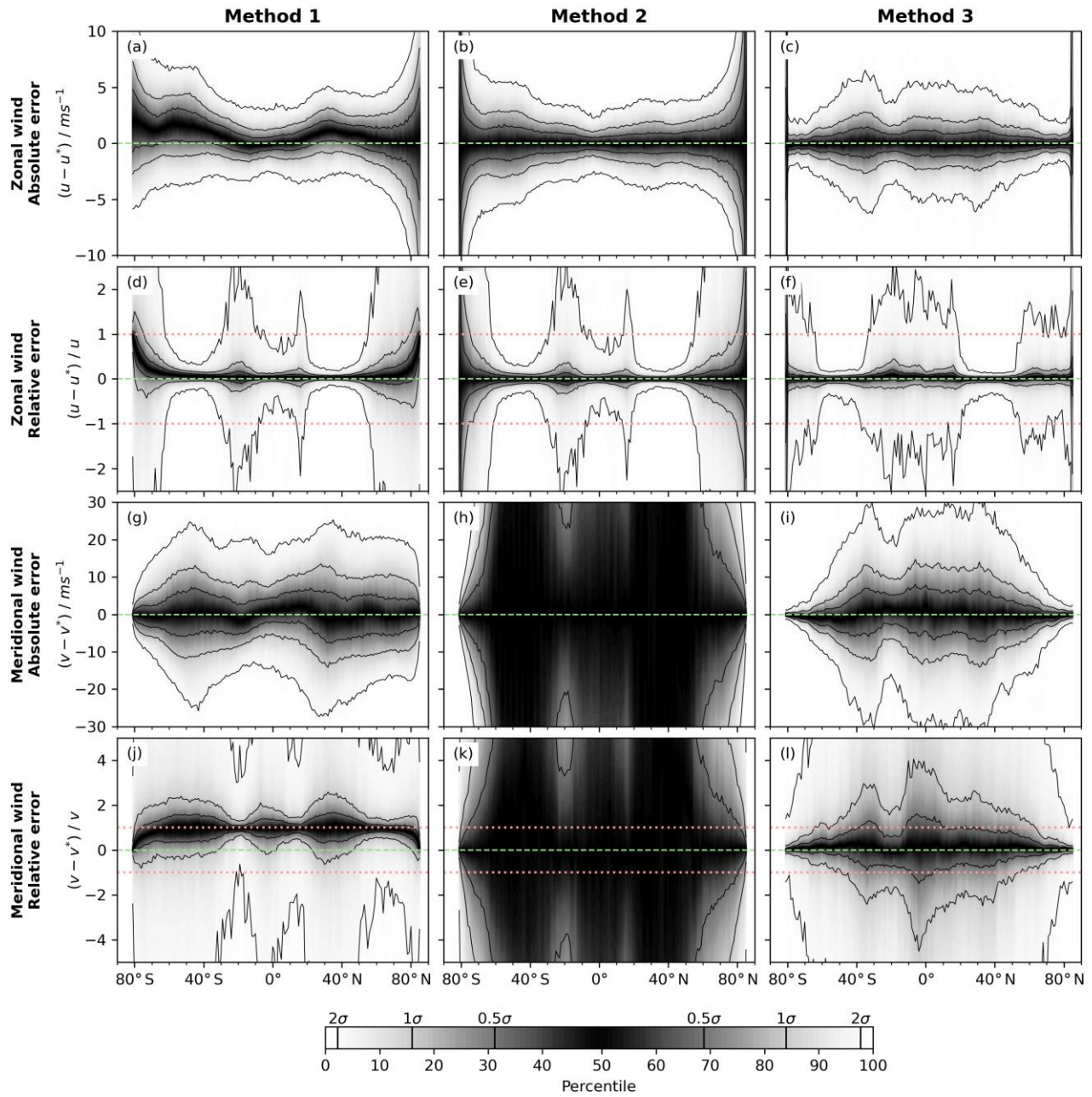
Figure 7: Statistical distribution of absolute and relative errors for the different methods versus latitude (x-axes). Data from the whole month of January 2021 is used here. The green dashed lines indicate zero absolute and relative wind errors, the red dotted lines in the relative error plots indicate errors of 100%.
