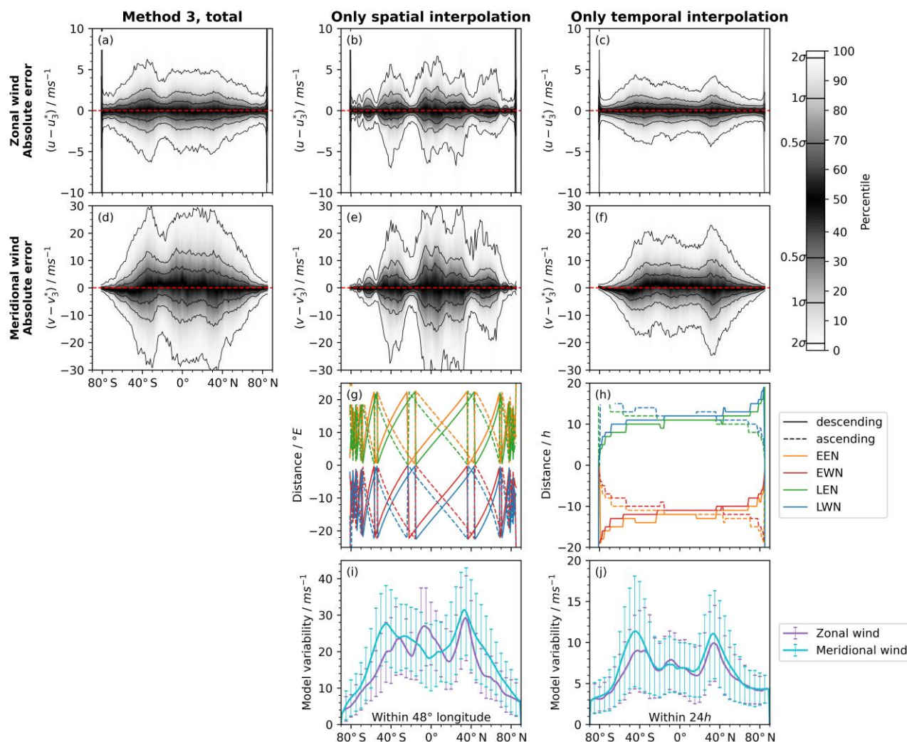
460 Figure 8: Influence of spatial and temporal interpolation on the total error statistics of Method 3. Panels a & d are a copy of Figure 7 c & i. The first two rows show the error statistics for zonal and meridional wind. In the third row, the spatial (g) and temporal (h) distance to the four nearest neighbours used for interpolation is plotted. The bottom row depicts the mean difference between maximal and minimal wind speed within 48° longitude (i) and 24 h (j) derived from ERA5 data. Data from the whole month of January is used for this variability analysis.
