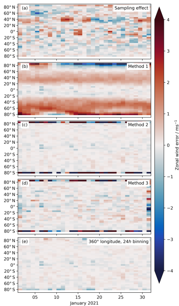
470 Figure 9: Absolute errors in the daily zonal mean zonal wind calculation for January 2021. Panel (a) shows errors originating in the Aeolus sampling, panels (b-d) the errors when using the three conversion methods, respectively, and panel (e) the errors for Method 3, but with a slightly different colocation/binning algorithm. The sampling bias shown in Panel (a) has been removed from the error estimates in panels (b-e).
