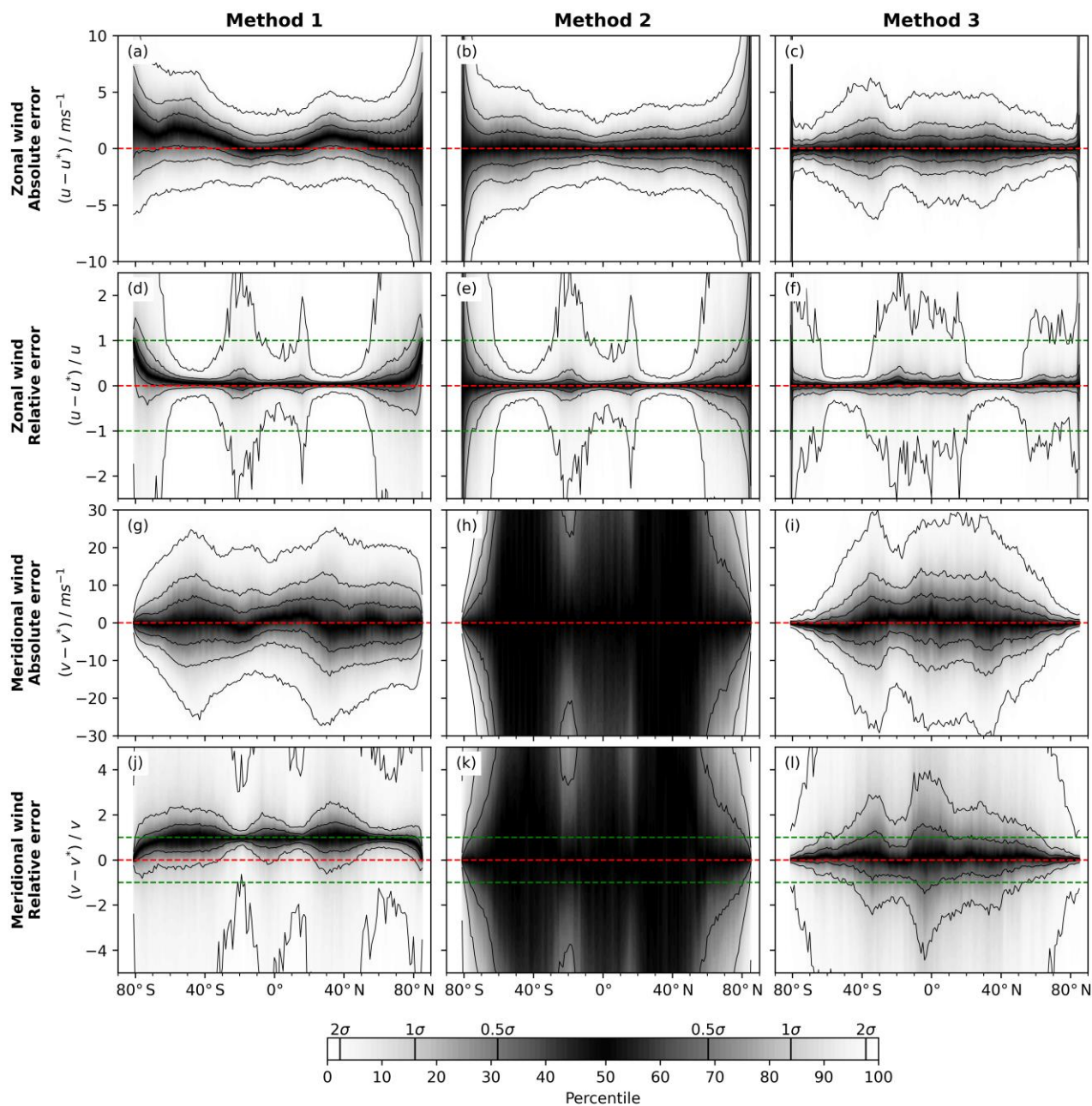
455 Figure 7: Statistical distribution of absolute and relative errors for the different methods versus latitude (x-axes). Data from the whole month of January 2021 is used here.
