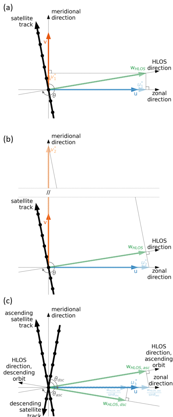
430 Figure 2: Geometric concepts of the three methods to convert Aeolus w_{HLOS} to zonal and meridional wind, which are introduced in this paper. Panel (a) shows the projection of w_{HLOS} onto zonal and meridional axes (Method 1), panel (b) the assumption of zero zonal or meridional wind (Method 2) and panel (c) the combination of ascending and descending measurements (Method 3).
