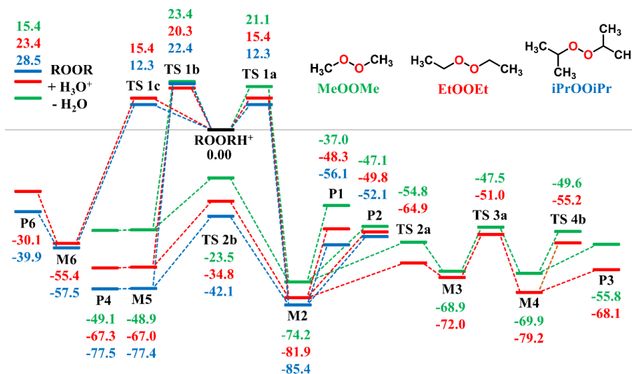
250 Figure S6. Potential energy surface calculated at the RHF-RCCSD(T)-F12a/VDZ-F12// \omega B97XD/aug-cc-pVTZ level of theory, for decomposition of Me-OO-Me (green), Et-OO-Et (red) and iPr-OO-iPr following protonation in the gas phase. Molecular structures for stationary points are shown in Scheme 2. Values given are relative zero-point corrected energies in kcal m mol -1 .
