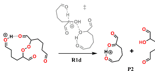
410 Figure S12. Initial decomposition step R1d, found for ROOR and ROOH derived from cyclohexene ozonolysis.
