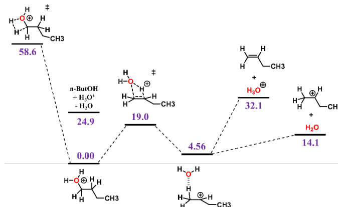
425 Figure S15. Potential energy surface calculated at the RHF-RCCSD(T)-F12a/VDZ-F12 // \omega B97XD/aug-cc-pVTZ level of theory for reaction following protonation in the gas phase, for n-butanol. Molecular structures carrying the double-dagger symbol ‡ are transition states. Values given in purple are relative zero-point corrected energies in kcal . mol -1 .
