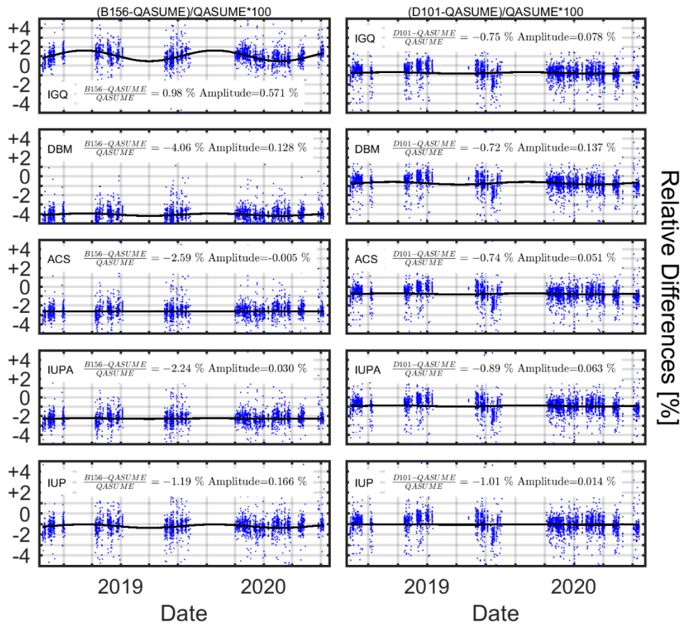
Figure 7: Comparison of TCO from Brewer 156 (left panels) and Dobson 101 (right panel) with TCO from traceable QASUME TCO retrieval for five different cross sections.
