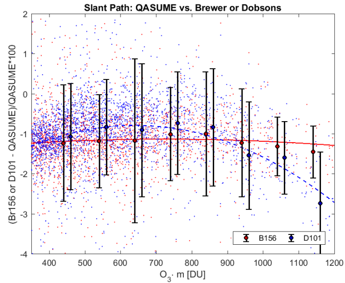
650 Figure 8: Differences of Brewer 156 and Dobson 101 retrieved with IUP cross section compared with QASUME TCO depending on the ozone slant path. The comparison with Brewer shows neglectable straylight effects.
