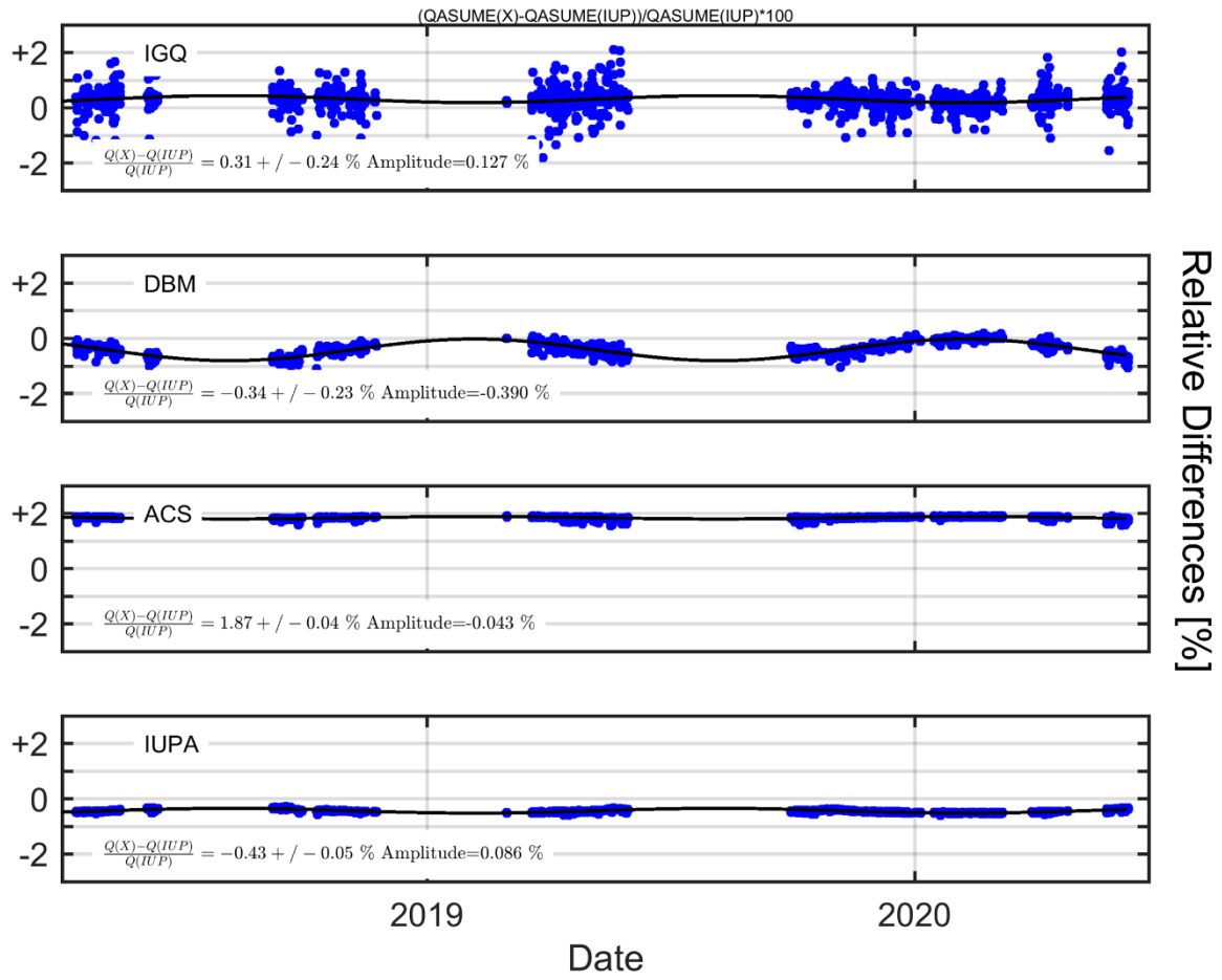
Figure 2: Differences (in %) of systematic offset, point to point variability (+/-) and seasonal variation (amplitude) of TCO retrieval of different cross sections compared with the IUP standard cross section.
