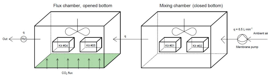
Figure 3. Scheme of the Dynamic SS-TF Chamber designed and built at IC3 for continuous CO 2 flux measurements.
