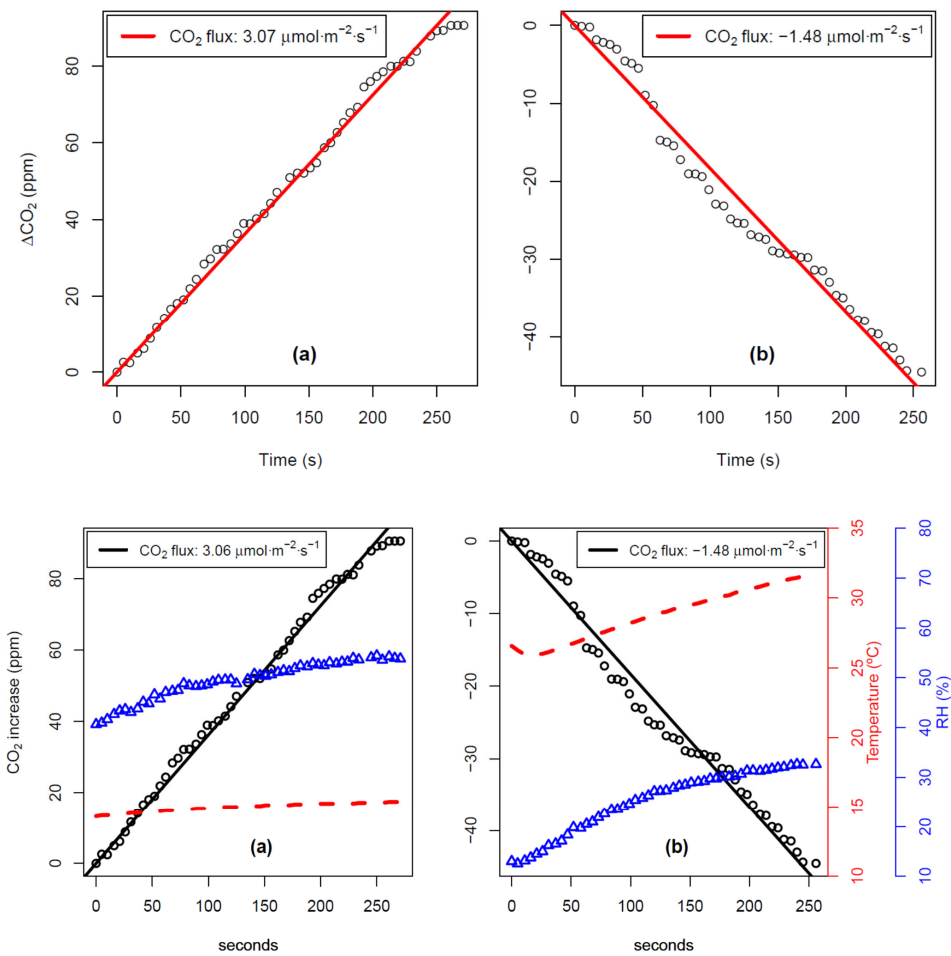
Figure 67. Example of two cases where the linear accumulation method was applied within an NSS-NTF chamber to calculate positive (a) and negative (b) CO 2 fluxes with Kit #03.
