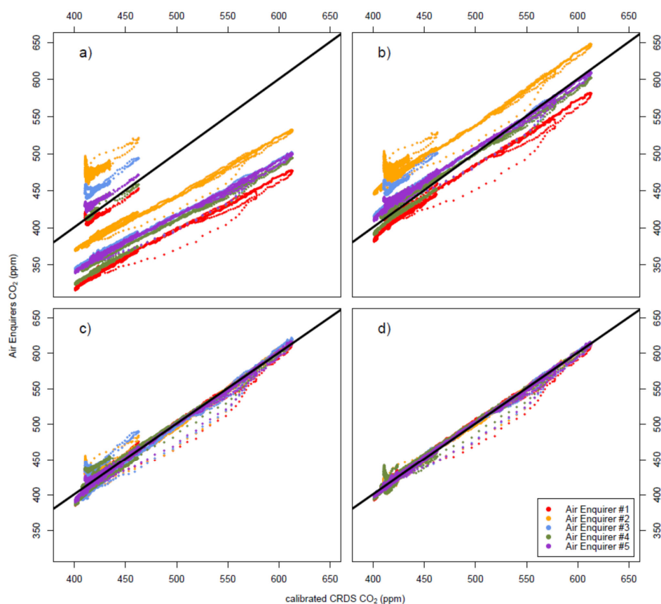
Figure 5. CO 2 concentrations in air measured by each of the Air Enquirer AE sensors during the experiment carried out at the CRAM and IC3 stations before (a) and after (b) correction and calibration was applied, vs CRDS data using sensor with raw data (a), sensor data theoretically corrected by P and RH (b), sensor data corrected by P and RH and calibrated with the CRDS (c) and sensor data corrected by P and RH and calibrated using a multiparametric lineal model (d)
