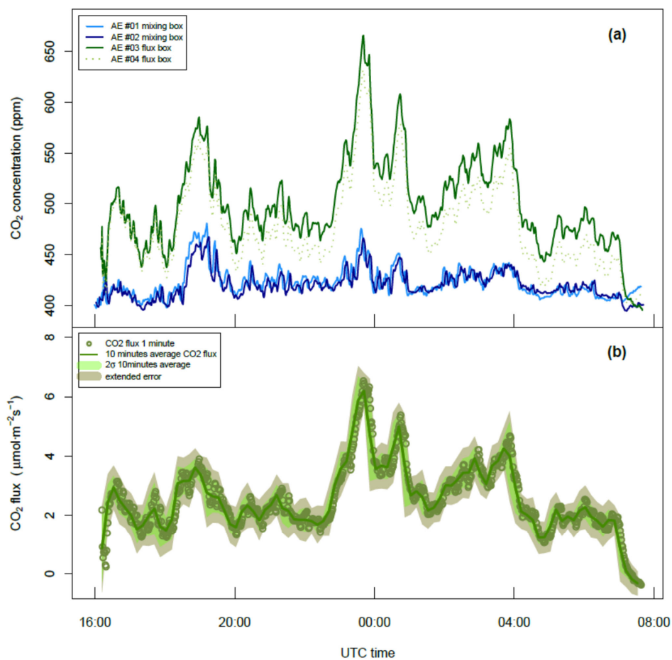
Figure 56. Time series of 10-min average CO 2 concentrations (upper panel) measured within the SS-TF chamber at the CRAM soilgrassland between 1st and 2nd of June 2016, and calculated f_{CO_2} (lower panel). The 2σ range for 10 minutes average variability and the extended error (adding 2 times the RSE of the multiparametric fit) are also plot.
