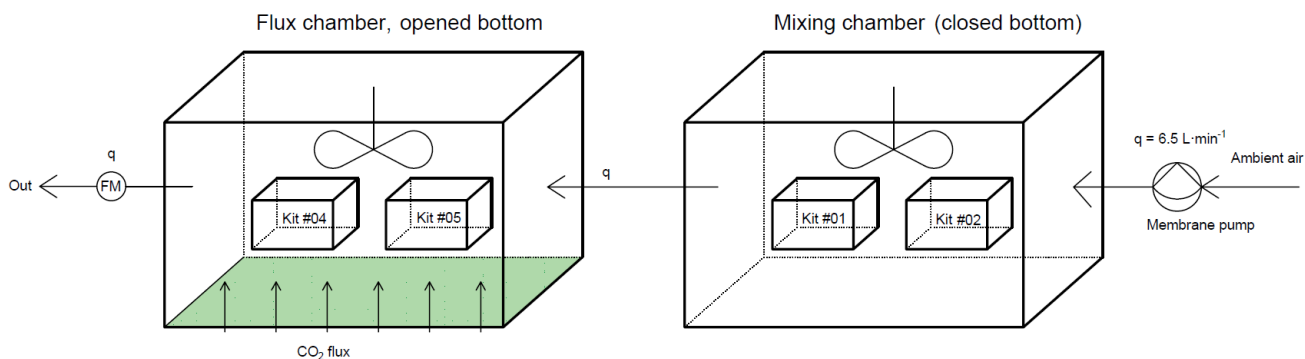
465 Figure 3. Scheme of the Dynamic SS-TF Chamber designed and built at IC3 for continuous CO 2 flux measurements.
