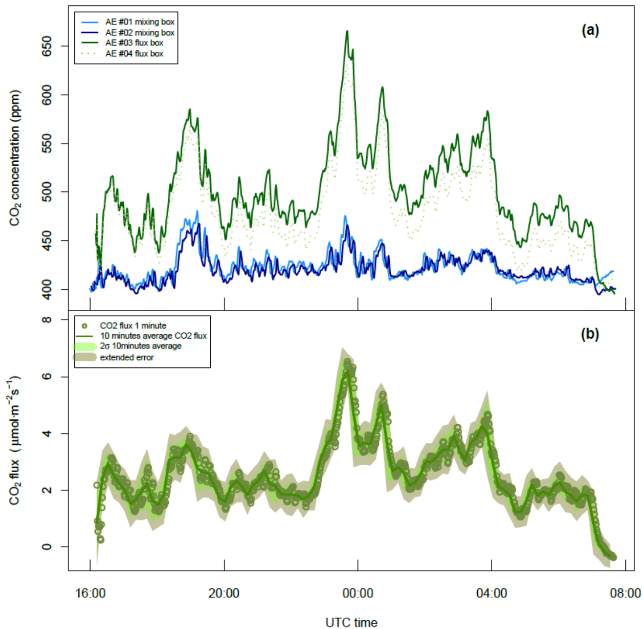
Figure 6. Time series of 10-min average CO 2 concentrations (upper panel) measured within the SS-TF chamber at the CRAM grassland between 1st and 2nd of June 2016, and calculated f_{CO_2} (lower panel). The 2 \sigma range for 10 minutes average variability and the extended error (adding 2 times the RSE of the multiparametric fit) are also plot.
