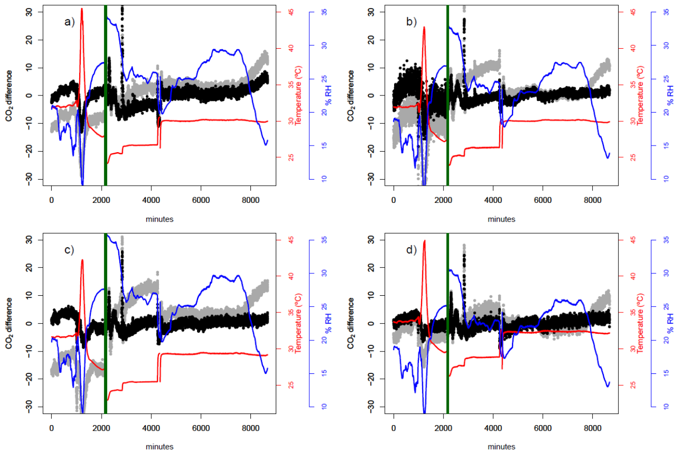
470 Figure 4. Timeseries of differences between CRDS CO 2 value and CO 2 AE kits value after simple calibration (grey) and after multiparametric fitting (black) for AE kit #1 (a), kit #2 (b), kit #3 (c) and kit #5 (d). Temperature values (red) and RH values (blue) are also plotted. Values before vertical green line correspond to the calibration at IC3, and after it to the calibration at CRAM.
