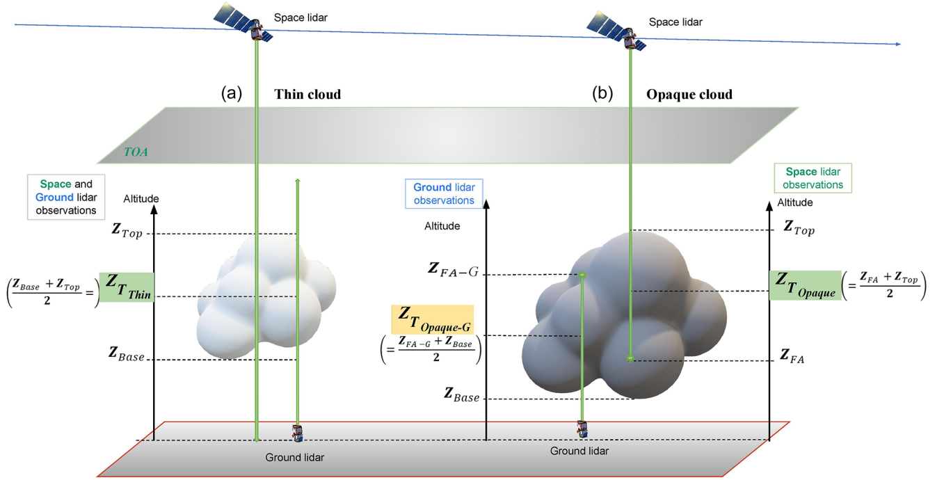
Figure 1. Schematic of cloud altitudes seen from space lidar and from a ground-based lidar in an atmospheric column containing thin cloud only (a) and opaque cloud only (b). The altitudes used to retrieve the surface LW CRE from CALIPSO–GOCCP are reported in green.
