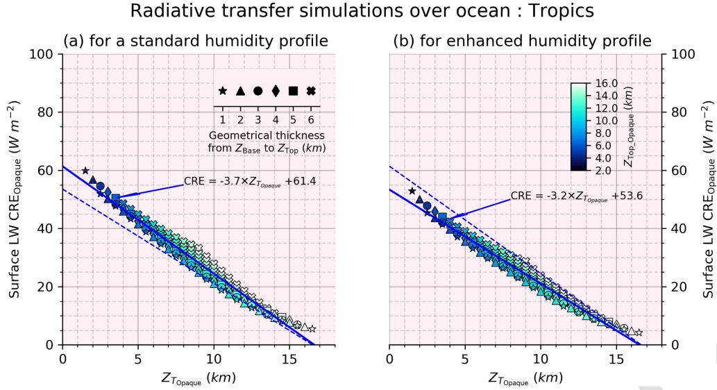
Figure 4. Same as Fig. 3a for (a) a standard humidity profile and (b) an enhanced humidity profile, both in the tropics: [30^{\circ}\text{S}–30^{\circ}\text{N}] .
