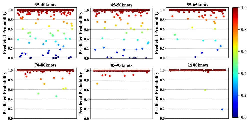
295 Figure 7. Predicted probability for each of TC images with varied intensity levels in the testing L image dataset via TG-1 model
