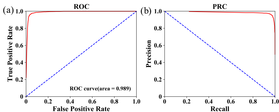
Figure 15. ROC and PRC curves of the TG-1 model for NWPO images during testing process
