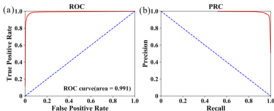
Figure 6. ROC and PRC curves of TG-1 model for L images during testing process
