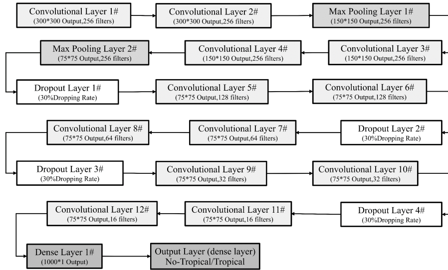
Figure 3. Detailed structure of the proposed DCNN model
