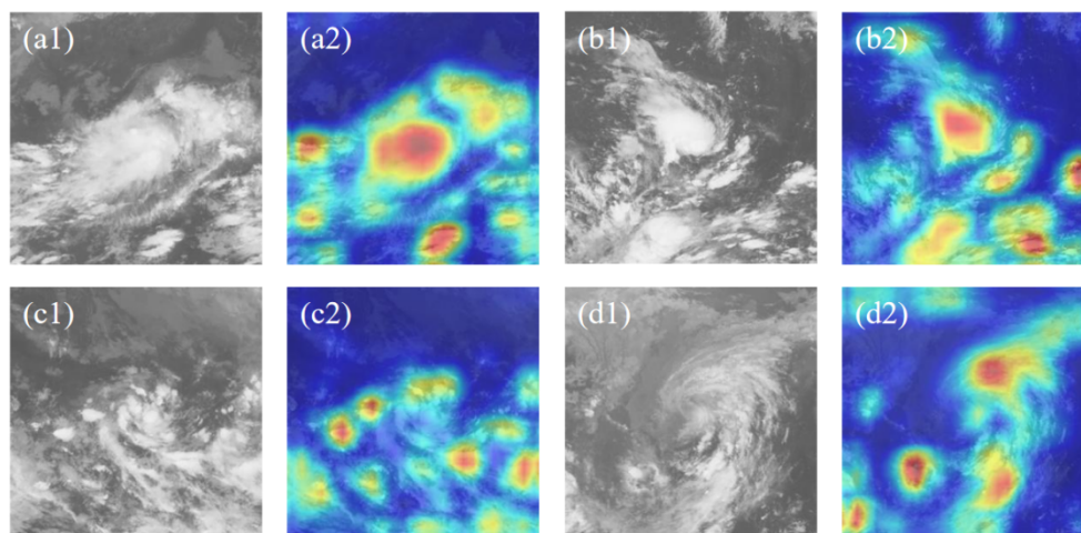
Figure 11. Heat maps of some non-TC images but misjudged as TC images compared with associated L images
