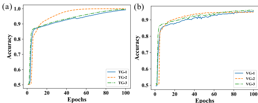
Figure 14. Evolutional curves of the prediction accuracy of the proposed DCNN model for NWPO images: (a) training process; (b) validation process
