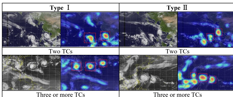
Figure 21. Heat Maps of some successfully identified TC images compared with associated NWPO images that involve multiple TCs
