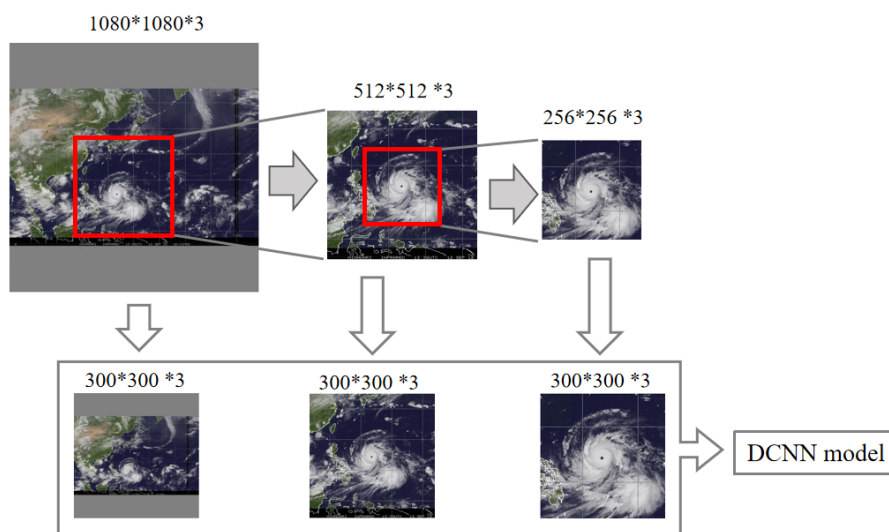
Figure 13. Flowchart for the realization of image pyramid of a TC image
