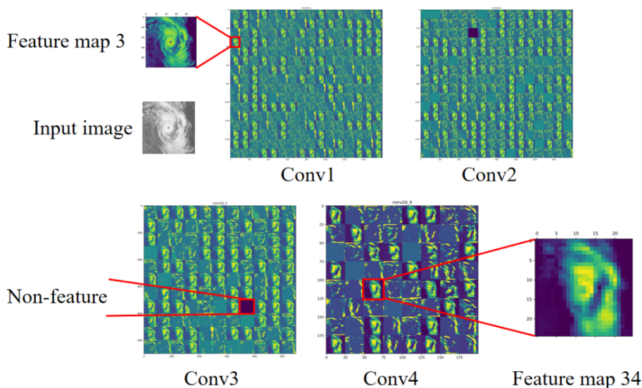
Figure 4. Visualization of outputs from the convolution kernels involved in the first 4 convolutional layers of a DCNN model
