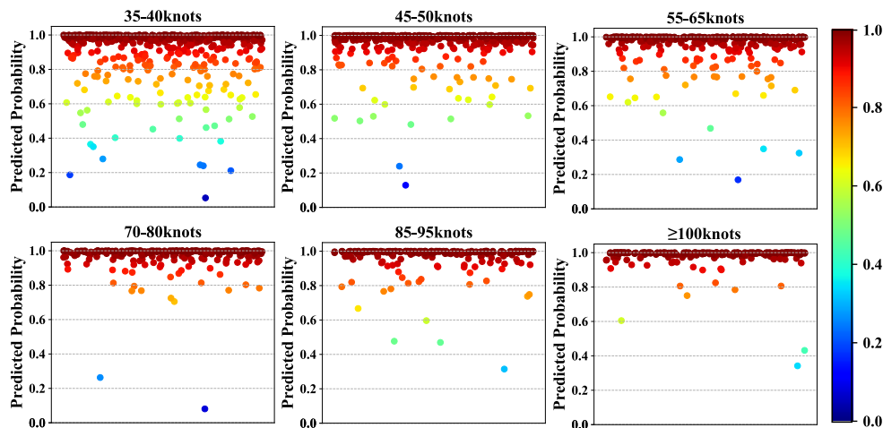
Figure 17. Prediction probability for NWPO images involving a single TC stratified by TC intensity
