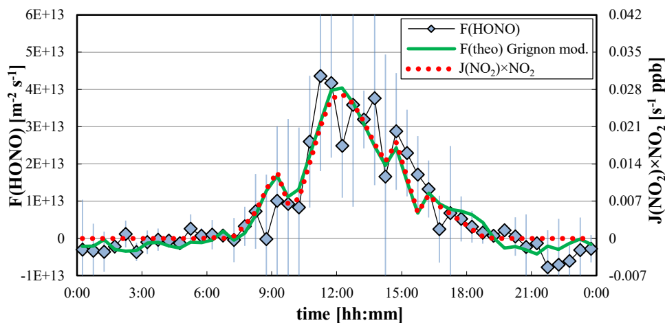
475 Figure 6: Average diurnal day of the HONO fluxes of the last four days of the campaign in comparison to a modified parameterization from former gradient measurements in Grignon/France (Laufs et al., 2017), see section 5.4. Error bars represent the standard deviation of the HONO fluxes of the four days. In addition, the scaled product J(NO_2) \cdot [NO_2] is also shown.
