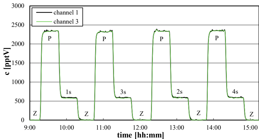
380 Figure 4: HONO mixing ratios during test measurements using a pure HONO source and variable valve switching times (30 s data). “Z”: zero; “P”: parallel ambient measurements; “xs”: valve switching experiments with constant periods for up-, down and deadband measurements (each with 1, 2, 3, 4 s using the sequence: up, deadband, down and deadband; dilution each by a factor of four).
