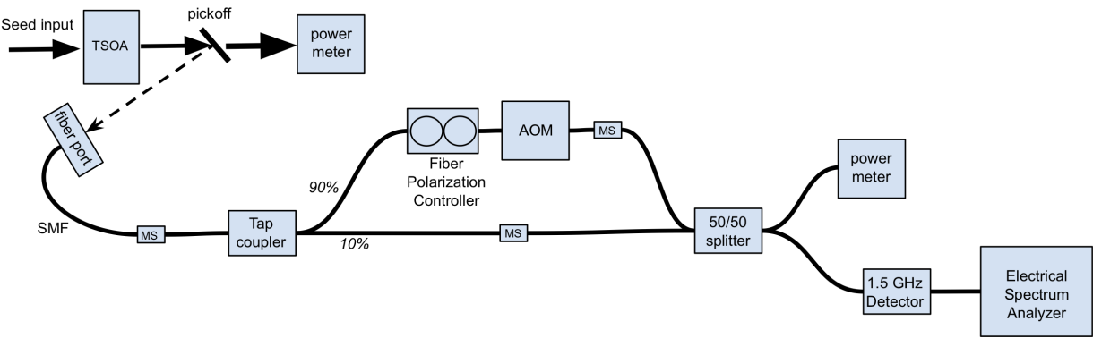
Figure A1. Test setup to measure the linewidth and spectral purity. AOM: Acousto-Optic Modulator, MS: Mating sleeve, SMF: single-mode fiber, TSOA: Tapered Semiconductor Optical Amplifier
