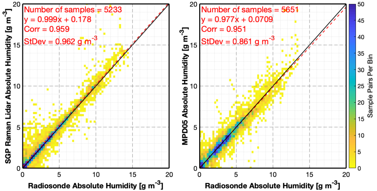
Figure 3. Frequency histograms showing the correlation between the SGP Raman Lidar (left) and Gen 4 MPD05 (right) with 77 collocated radiosondes between 19 Apr to 1 May 2019. The colors indicate the number of sample pairs per bin, 0.1x0.1 g m -3 bin sizes. The correlation between Raman lidar and radiosondes is expected to be near 1 as the lidar is calibrated from the same sondes while the MPD retrievals are run independent of the radiosonde information.
