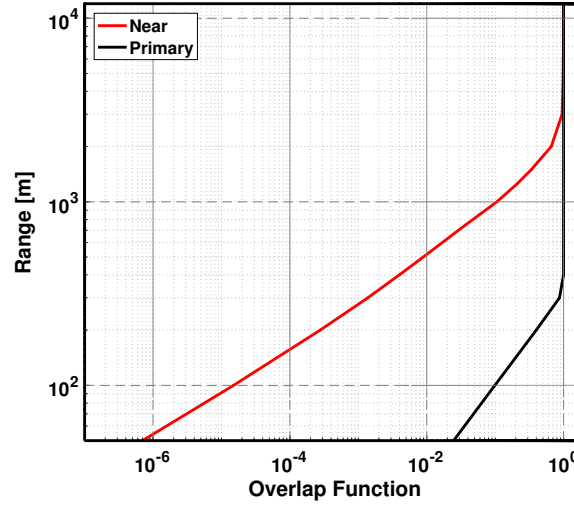
Figure B1. Overlap function for the primary and near/WFOV receivers.
