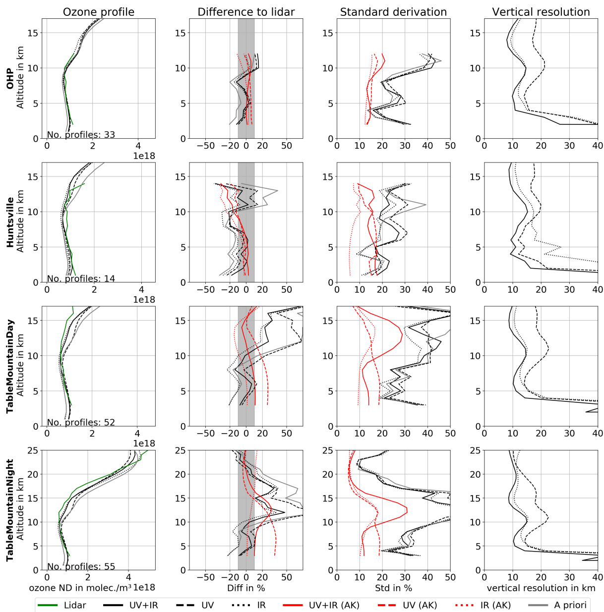
Figure 4. Ozone profile comparison between UV+IR, UV-only, and IR-only retrievals and tropospheric ozone lidar measurements from three different sites. Table Mountain provides in addition daytime (matching S5P/CrIS overpasses) profiles. Nighttime profiles can reach a height of up to 28 km and are used for comparison up to 25 km. In the panel showing the difference, the grey shaded area marks the \pm 10\% range.
