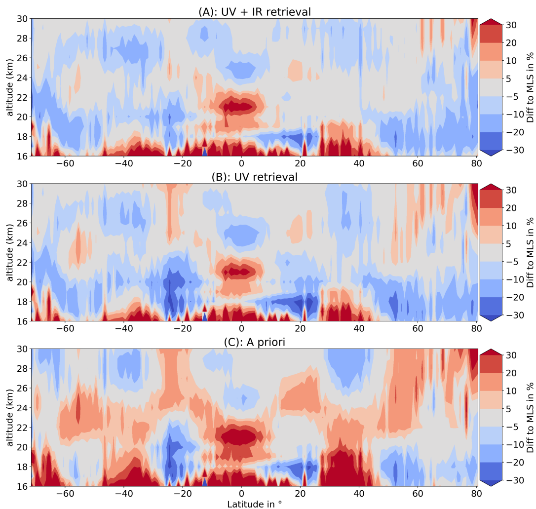
Figure 12. Zonal mean differences in percent between combined TOPAS ozone profiles (A), UV-only TOPAS profiles (B) as well as the climatological (a priori) (C) and MLS data on 1 October 2018.
