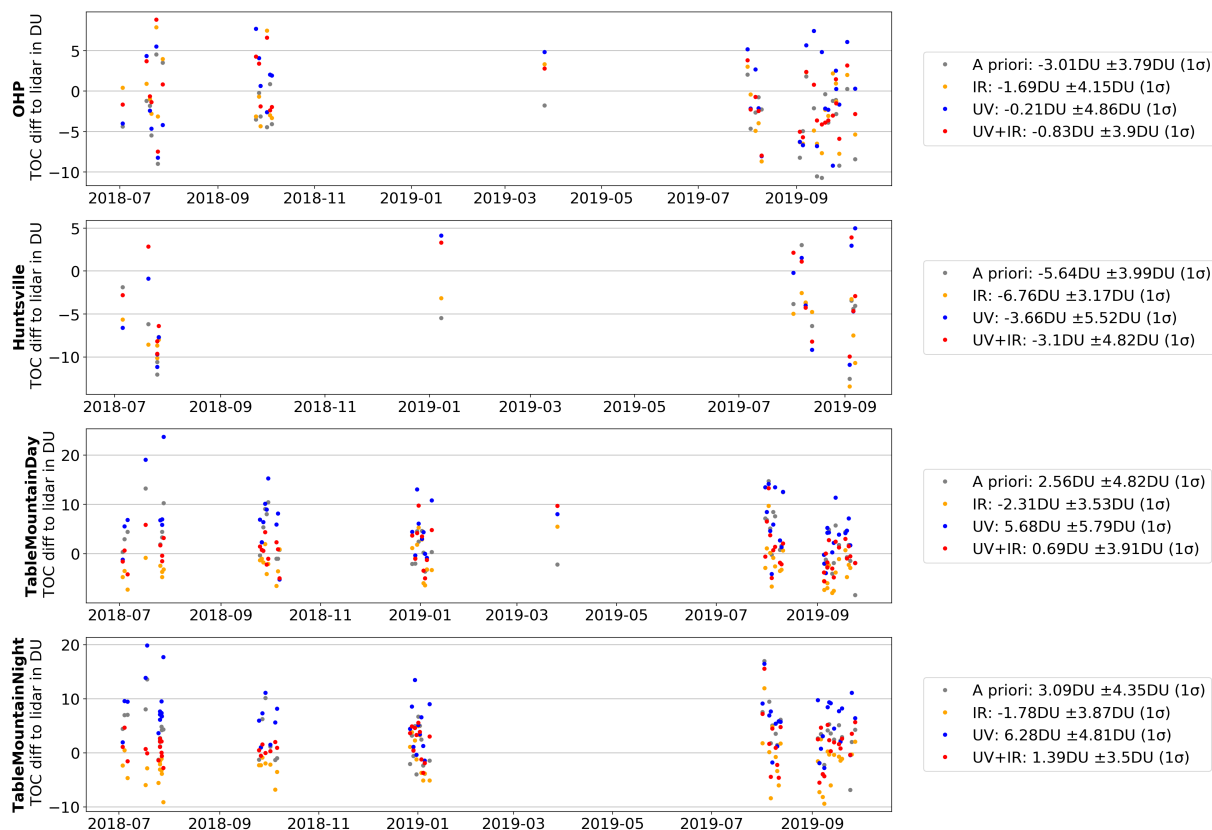
Figure 5. Absolute differences in the tropospheric ozone content (TOC) with respect to the tropospheric lidar data. TOCs are calculated by integrating ozone profiles from the lowermost retrieval level altitude up to the tropopause. The height of the tropopause is obtained from the ERA5 reanalysis data using the 2 PV definition. In the legend the mean absolute differences and the standard deviations are given.
