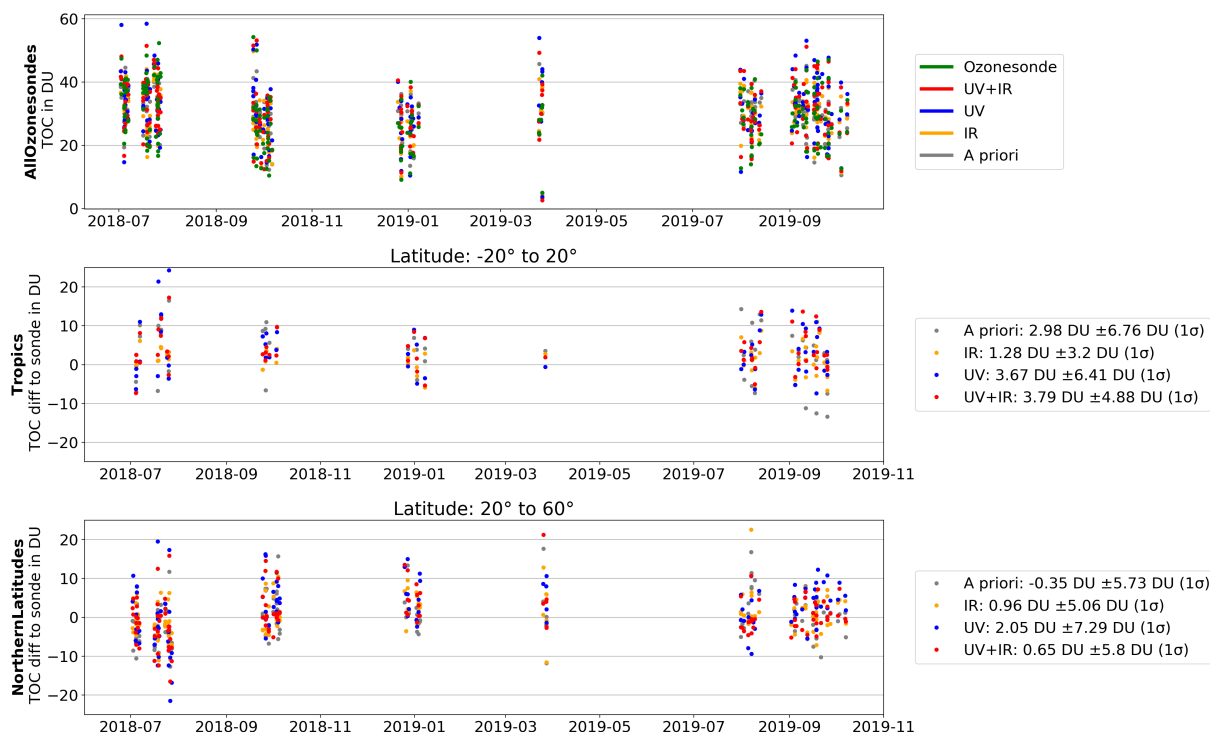
Figure 9. Comparison of tropospheric ozone content (TOC). Upper panel: TOC from TOPAS retrievals and ozonesondes. Middle panel: Absolute differences in TOC with respect to the ozonesonde data in the tropics (20°S – 20°N). Lower panel: same as the middle panel but for the northern latitudes (20°N – 60°N). TOCs are calculated by integrating ozone profiles from the lowermost retrieval level altitude up to the tropopause. The height of the tropopause is obtained from the ERA5 reanalysis data using the 2 PVU definition. In the legend (to the right), the mean absolute differences and the standard deviations are given.
