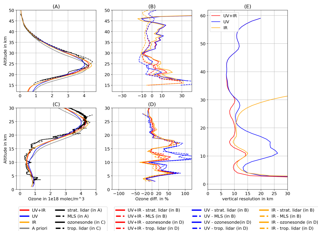
Figure 2. Comparison between UV+IR, UV-only, and IR-only ozone profile retrievals and collocated stratospheric lidar and MLS measurements (A and B) and collocated tropospheric lidar and ozonesonde profiles (C and D). The TROPOMI and CrIS data were obtained at 34.2° latitude and -117.9° longitude on 27 September 2018 at 21:20:11. All measurements, the MLS ozone profile, the ozonesonde and tropospheric/stratospheric lidar sounding from Table Mountain Facility, are within 100 km distance of TROPOMI/CrIS. The time difference for is 25 minutes for MLS and between 6 and 8 hours (nighttime profile) for the lidars and ozonesonde. The vertical resolution of the 3 TOPAS retrievals is given in (E).
