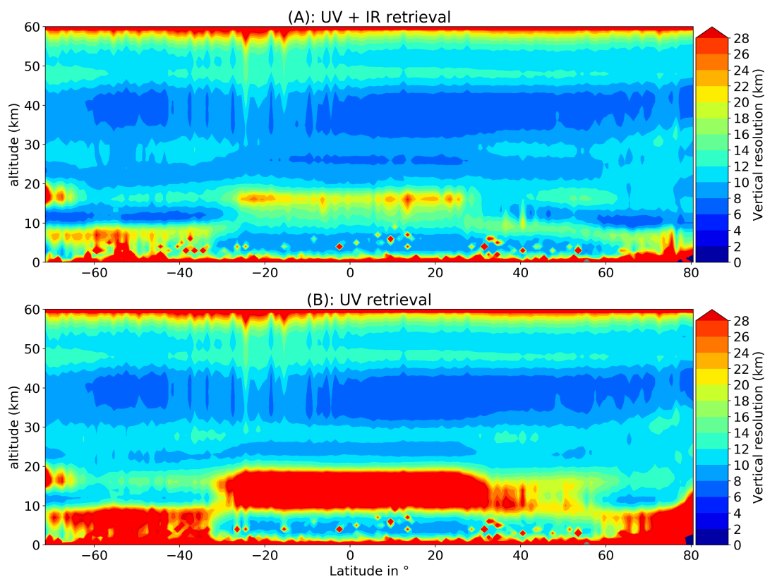
Figure 11. Zonally averaged vertical resolution for one day of TOPAS retrieval data (1 October 2018). The vertical resolution is given by the inverse main diagonal of the AK matrix. Upper panel (A): vertical resolution for the combined retrieval. Lower panel (B): vertical resolution from the UV-only retrieval.
