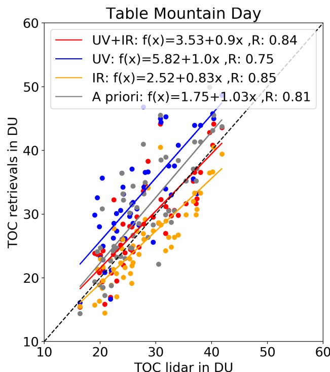
Figure 6. TOC scatter plot of TOPAS retrievals with respect to Table Mountain tropospheric lidar data (daylight measurements). The one-to-one line is given by the black dashed line. The linear regression curves are plotted with different colours and their equations are given in the legend.
