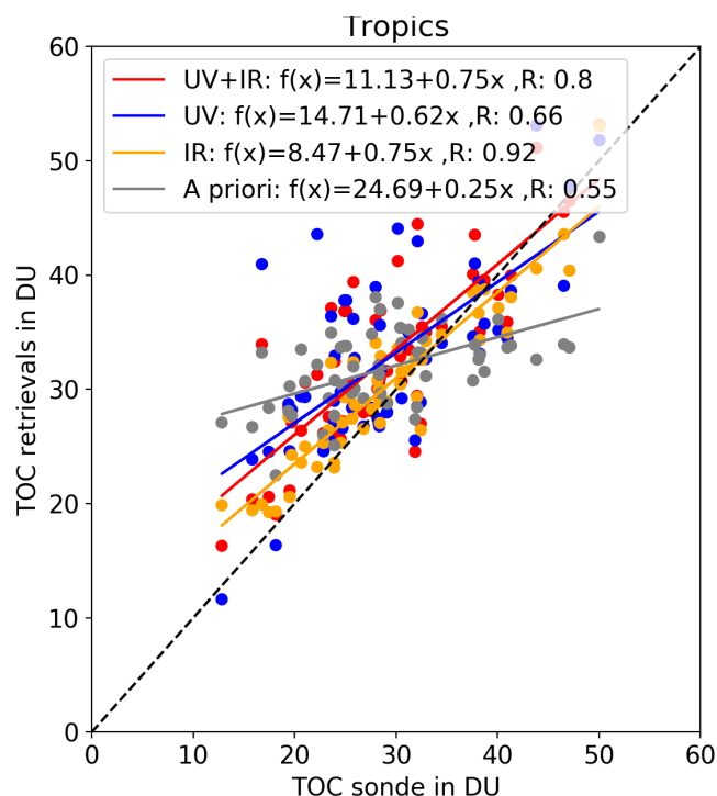
Figure 10. Scatter plot of TOCs from TOPAS retrievals with respect to ozonesonde data in the tropics. The one-to-one line is given as a black dashed line. The linear regression curves are plotted with different colours and their equations are given in the legend.
