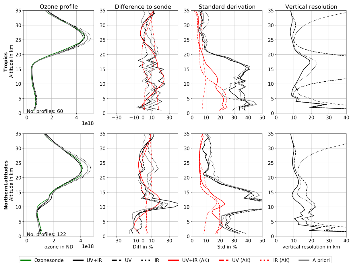
Figure 7. Ozone profile comparisons between UV+IR, UV-only and IR-only retrievals and ozonesonde measurements for northern and tropical latitudes.
