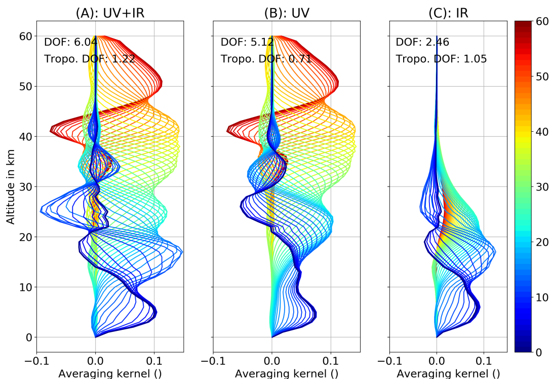
Figure 3. Rows of the averaging kernel matrix for the three retrievals shown in Fig. 2. Each line represents the sensitivity of the ozone profile retrieval at a certain altitude level from 0 km (blue) to 60 km (red). DOF is given by the sum of the AK matrix main diagonal. The tropopause is defined by 2 PVU from ERA5 reanalysis.
