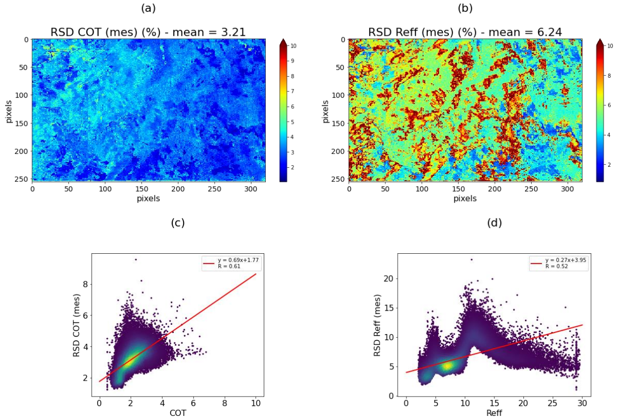
Figure 5: Uncertainties (RSD) in % of COT (a) and R_{eff} (b) originating from the measurement errors for the case study of CALIOSIRIS. COT uncertainties as a function of COT (c). R_{eff} uncertainties as a function of R_{eff} (d).
