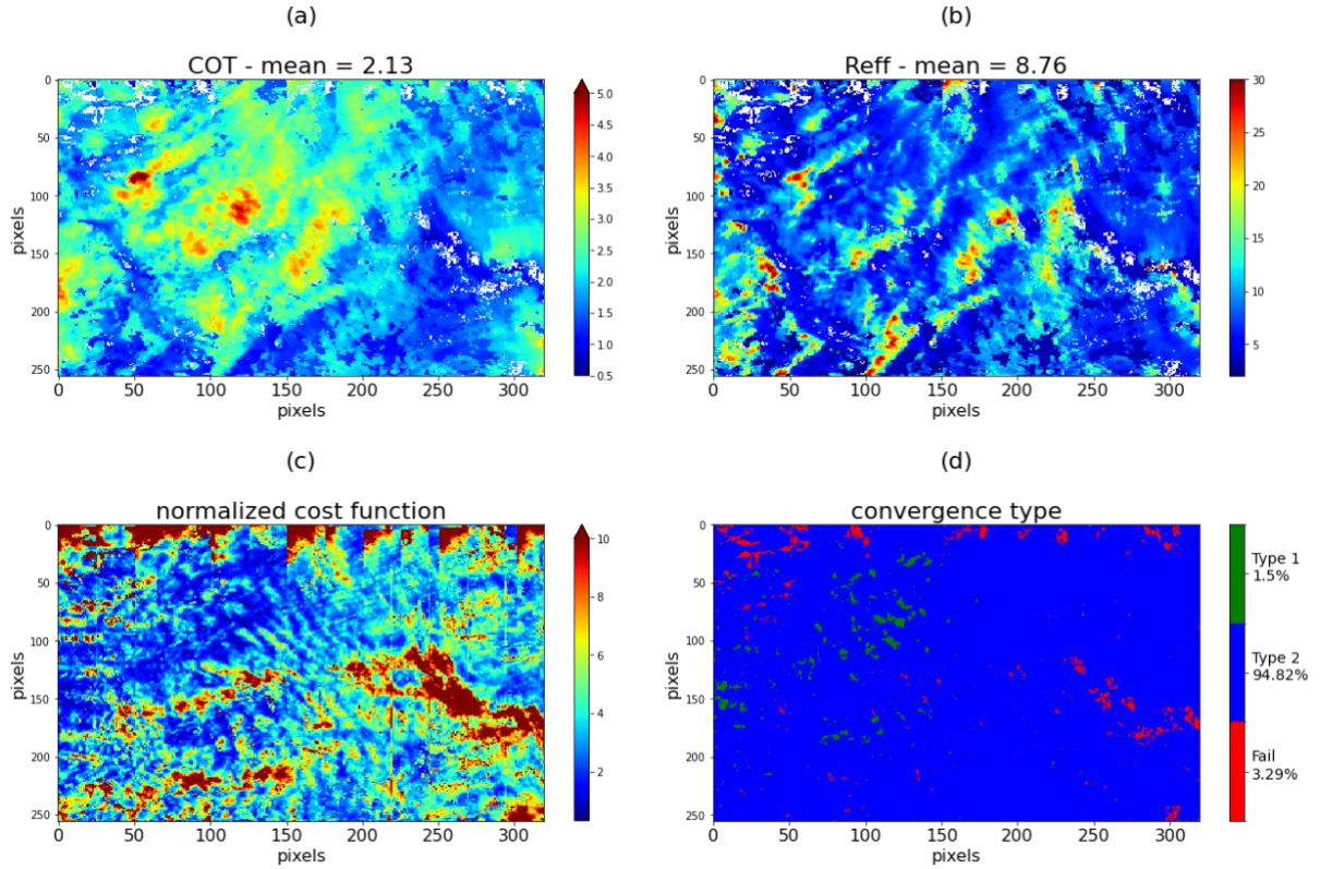
Figure 4: COT (a) and R_{eff} (b) retrieved using a multi-angular bispectral method from a liquid cloud case observed during the CALIOSIRIS airborne campaign on 24 October 2014 at 11:02 (local time). Pixels associated to failed retrievals are represented by white pixels. (c) Normalized cost function. (d) Convergence type (Eq. 6 for Type 1 and Eq. 7 for Type 2) and failed retrieval.
