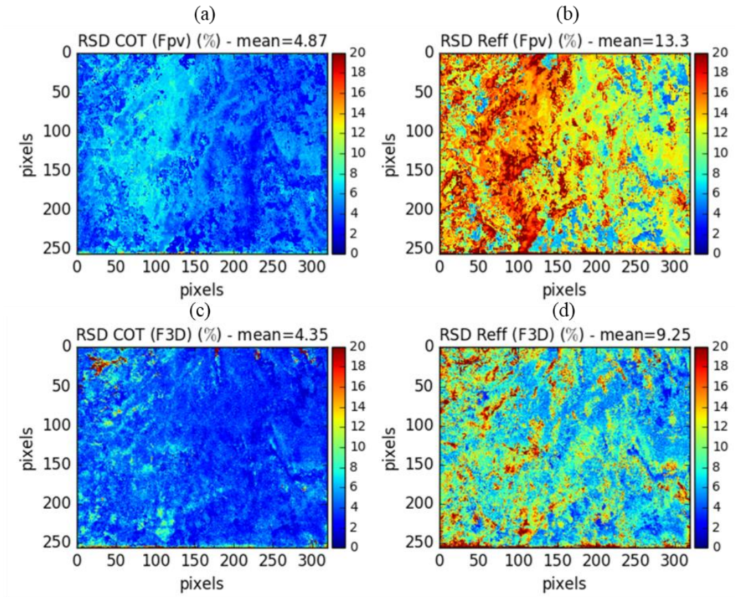
Figure 7: The uncertainties (%) on COT and R_{eff} originating from the assumptions in the forward model when not considering the heterogeneous vertical profile (a and b) and the 3D radiative transfer (c and d).
