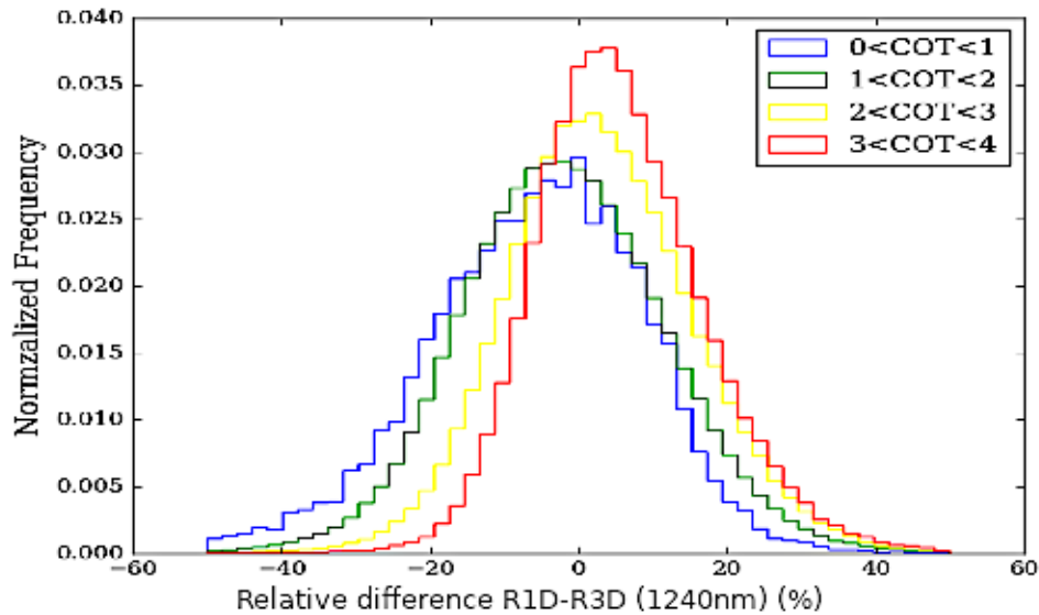
Figure 9: Histograms of the relative difference between the reflectances computed in 1D and 3D at 1240 nm for the central image. Each histogram corresponds to a domain of COT.
