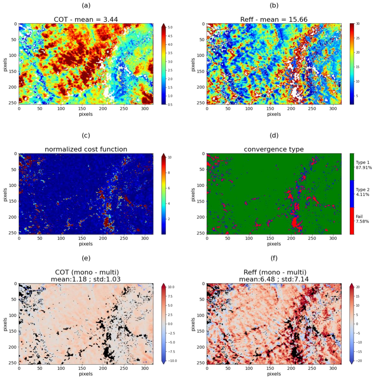
625 Figure 10: COT (a) and R_{\text{eff}} (b) retrieved using the mono-angular bispectral method for the CALIOSIRIS liquid cloud case study on 30 June 2014 at 11:02 (local time). Pixels associated with failed retrievals are represented by white pixels. (c) Normalized cost function. (d) Convergence type (Eq. 6 for Type 1 and Eq. 7 for Type 2) and failed retrieval. Differences between mono-angular and multi-angular retrieval for retrieved optical thickness (e) and retrieved effective radius (f).
