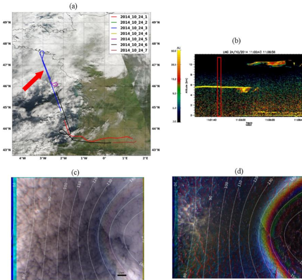
Figure 2: Studied case on 24 October 2014 at 10:02 UTC (11:02 local time): (a) In blue, airplane trajectory for this day above a MODIS/AQUA true color image. The red arrow corresponds to the studied segment (b) Quicklook of the backscattered signal provided by the LIDAR-LNG around the observed scene. The red rectangle corresponds to the studied scene (c) OSIRIS RGB composite image, obtained from the total radiances at channels 490, 670, and 865 nm. The blue bars on the left-hand side of the images are due to the motion of the airborne between the image acquisitions of the different filters (d) OSIRIS RGB composite image, obtained from the polarized radiances at channels 490, 670, and 865 nm. The white iso-contours in (c) and (d) represent the scattering iso-angles in a 10^\circ step.
