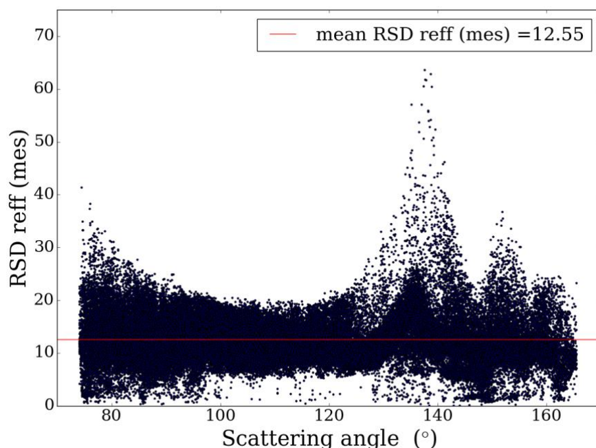
Figure 11: Uncertainties on the effective radius originating from the measurement errors, RSD R_{\text{eff}} (mes) as a function of the scattering angle for the mono-angular retrieval. The red line represents the mean RSD R_{\text{eff}} (mes) = 12.55\% .
