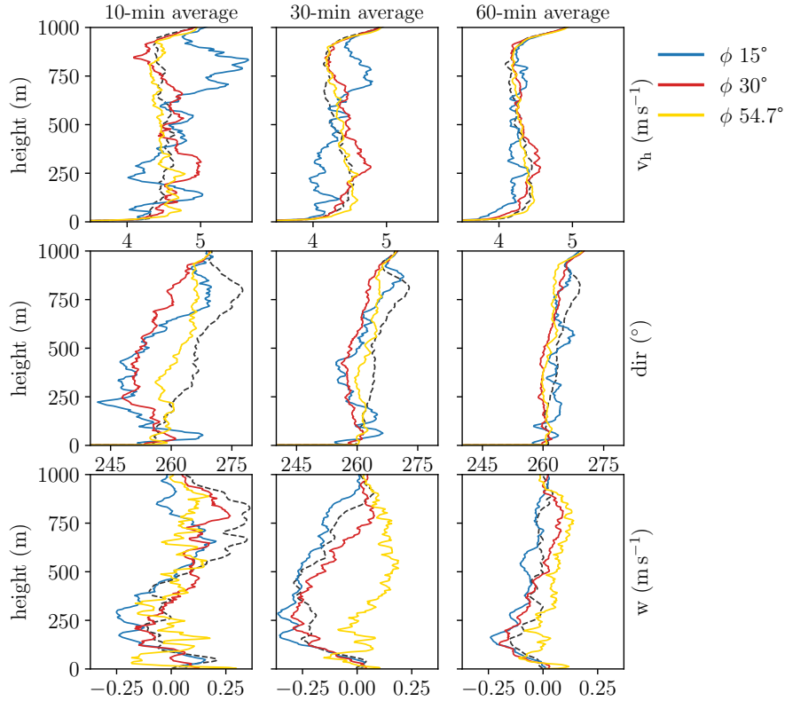
Figure 3. Simulation case 1: Time averaged vertical wind -profiles of the three-dimensional wind vector of lidar scans with the VAD 24 technique using different zenith angle configurations ( \phi ). Displayed are horizontal wind speed (upper panels), wind direction (center panels) and vertical wind (lower panels). Different colors indicate different zenith angle configurations. Reference profiles (true LES values) along the vertical column directly above the lidar location are shown in black (dashed lines).
