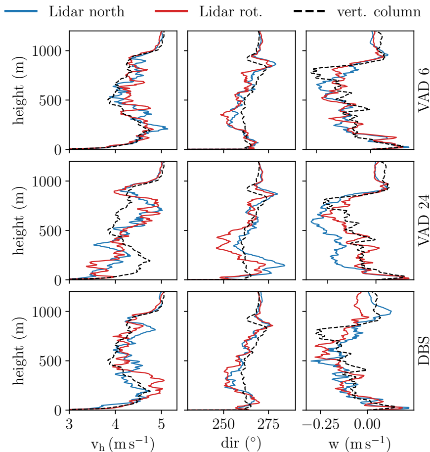
Figure 5. Simulation Case 1: Virtual lidar profiles obtained over a one exemplary 10-min period with a zenith angle configuration of 15^\circ using different scan schemes. Blue lines indicate profiles of north-oriented lidars and red lines indicate profiles of rotated lidars. For the VAD scans, lidars were rotated 30^\circ to the east, while for the DBS scan, the lidar was rotated 45^\circ to the east. Truth Reference profiles (LES values) along the vertical column directly above the lidar location (black dashed lines) are shown for reference.
