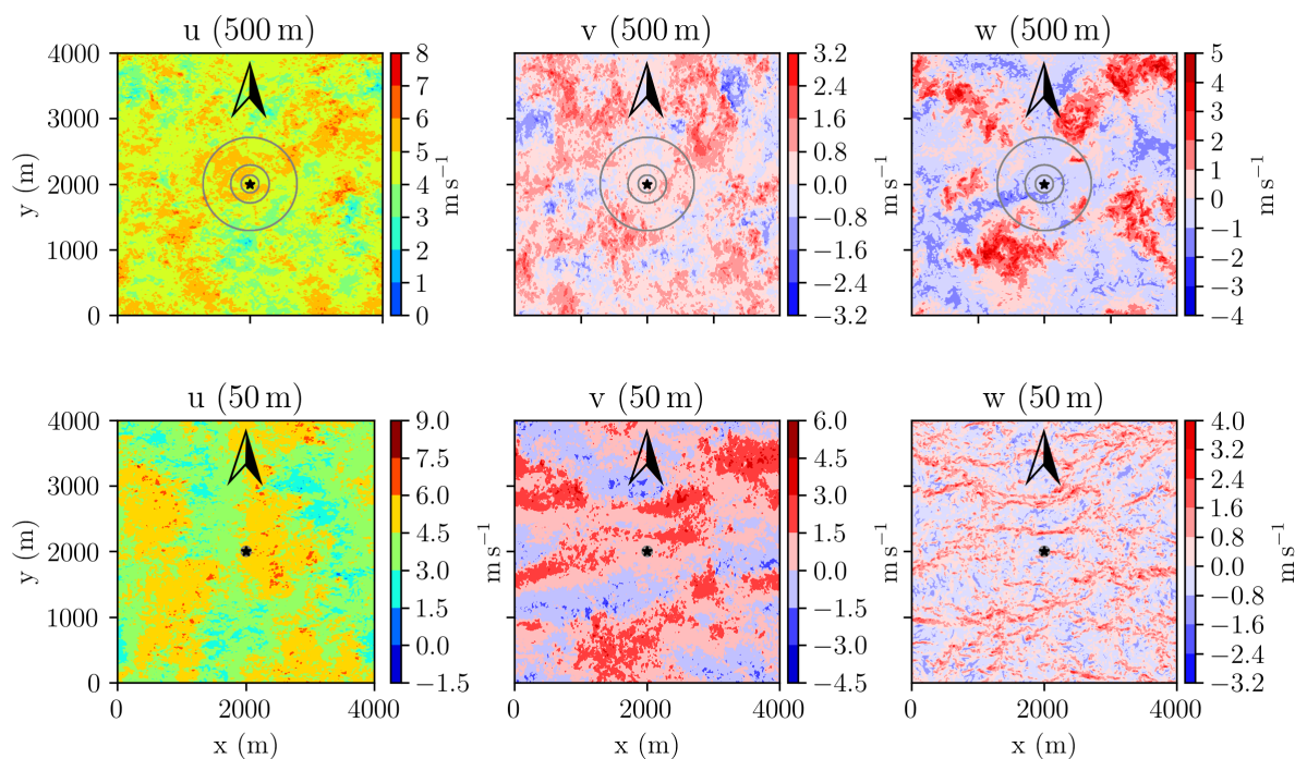
Figure 2. Simulation case 1: Horizontal cross sections of instantaneous flow field components (u, v, w) at 2 h simulation time, at 50 m and at 500 m height. The black star marks the location of the three virtual lidars, placed in the center of the domain. Each of the lidars is configured with a different zenith angle ( 15^\circ , 30^\circ , 54.7^\circ ). Gray circles indicate the corresponding scanning circles at the respective height level. Arrows are pointing north.
