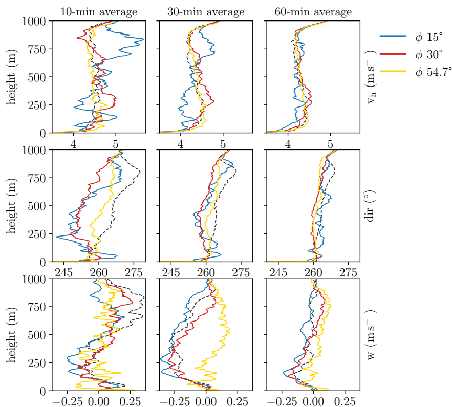
Figure 3. Simulation case 1: Time averaged vertical wind profiles of lidar scans with the VAD 24 technique using different zenith angle configurations ( \phi ). Displayed are horizontal wind speed (upper panels), wind direction (center panels) and vertical wind (lower panels). Different colors indicate different zenith angle configurations. Reference profiles (true LES values) along the vertical column directly above the lidar location are shown in black (dashed lines).
