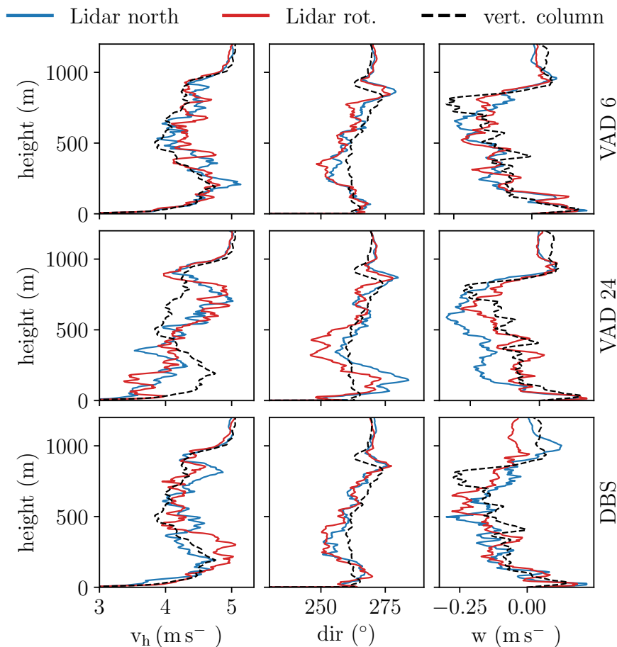
Figure 5. Simulation Case 1: Virtual lidar profiles obtained over a 10-min period with a zenith angle configuration of 15^\circ using different scan schemes. Blue lines indicate profiles of north-oriented lidars and red lines indicate profiles of rotated lidars. For the VAD scans, lidars were rotated 30^\circ to the east, while for the DBS scan, the lidar was rotated 45^\circ to the east. 'Truth' profiles (LES values) along the vertical column directly above the lidar location (black dashed lines) are shown for reference.
