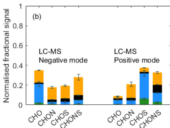
1165 Figure 2. (a) Elemental grouping from CIMS gas phase measurement, CIMS particle-phase measurement, LC-Orbitrap MS in the \alpha -pinene system. The signal of each compound is normalized to all compounds. (b) Elemental grouping for LC-Orbitrap MS inconclusive compounds. The signal of each compound is normalized to the total inconclusive compounds. The colors correspond to the ones in (a). Standard deviations ( n=2 for CIMS and n=3 for LC-Orbitrap MS) are indicated by error bars
