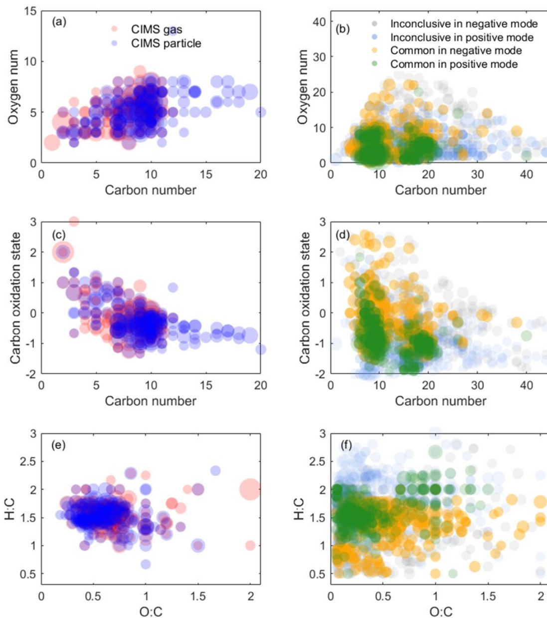
1170 Figure 3. Oxidation products distribution from the representative experiment detected by the CIMS measurement and LC-Orbitrap MS negative and positive mode. (a), (c) and (e) are for the CIMS measurements. (b), (d) and (f) are for LC-orbitrap MS measurement. The symbol size is proportional to the square root of the ion's signal intensity.
