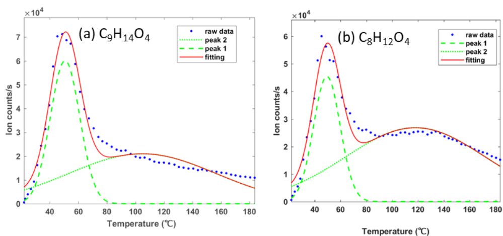
1155 Figure 1. Two examples of an ion with more than a single desorption peak in the FIGAERO-CIMS. Here the peaks at the lower desorption temperature were assigned to monomer C_9H_{14}O_4 (a) and C_8H_{12}O_4 (b) generated from \alpha -pinene directly and the broader higher temperature peaks being a fragment of another ion at the same mass.
