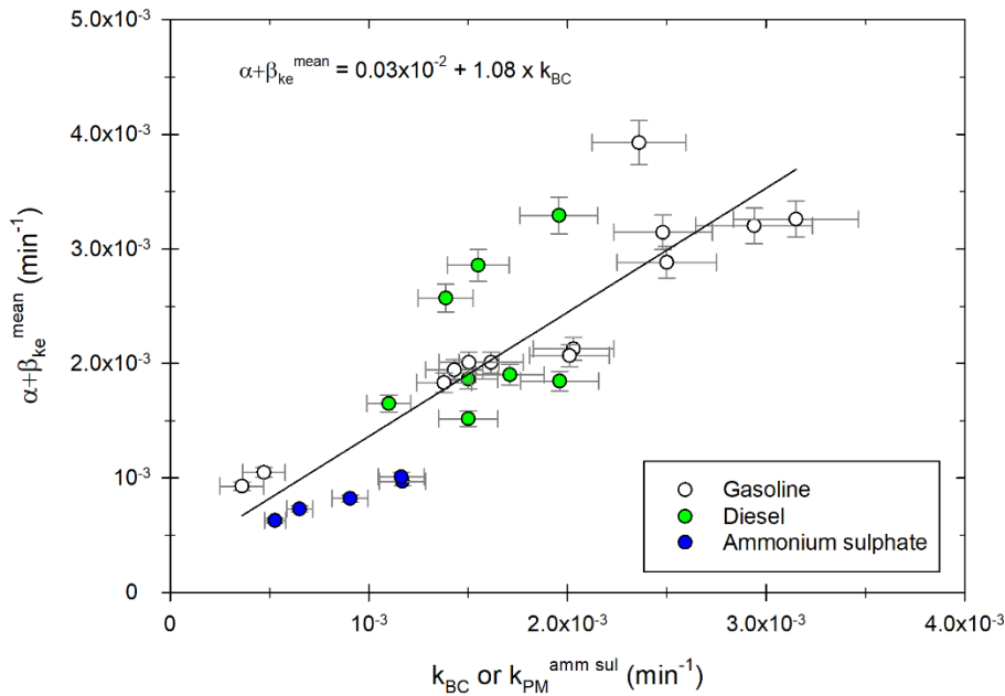
Figure 5 : Mean loss coefficient \alpha + \beta_{ke}^{\text{mean}} as a function of the decay coefficient k_{BC} or k_{PM}^{\text{amm sul}} obtained for the “neutralized walls” chamber experiments performed with particles from diesel (green) and gasoline (white) engines or ammonium sulphate particles (blue). A linear fit of the data is shown (black line).
