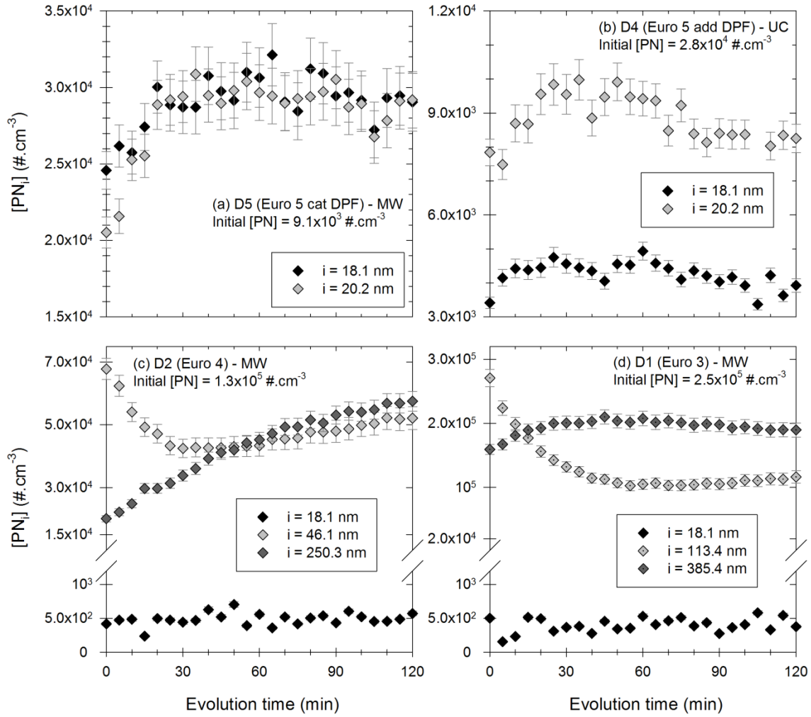
Figure 10: Evolution with time of the particles [PN] in certain diameter bins during 2 hours. Figures (a) and (b) show particles in the bins 18.1 nm (black) and 20.2 nm (light grey), for experiments with the vehicle D5 in MW conditions with an initial [PN] of 9.1 \times 10^3 \text{ \#.cm}^{-3} and with the vehicle D4 in UC conditions with an initial [PN] of 2.8 \times 10^4 \text{ \#.cm}^{-3} , respectively. Figure (c) shows particles in the bins 18.1 nm (black), 46.1 nm (light grey) and 250.3 nm (dark grey) with the vehicle D2 in MW conditions with an initial [PN] of 1.3 \times 10^5 \text{ \#.cm}^{-3} . Figure (d) shows particles in the bins 18.1 nm (black), 113.4 nm (light grey) and 385.4 nm (dark grey) with the vehicle D1 in MW conditions with an initial [PN] of 2.5 \times 10^5 \text{ \#.cm}^{-3} .
