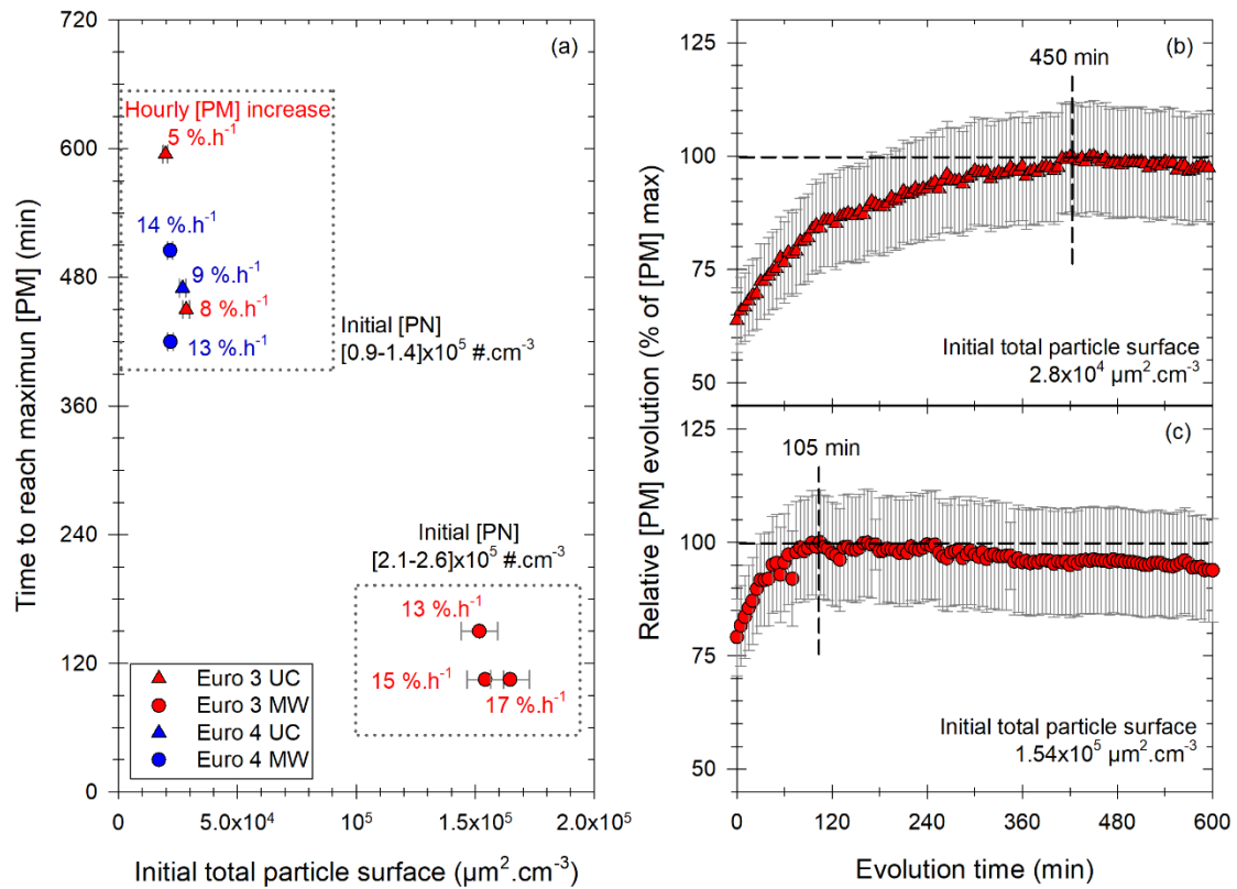
Figure 9: Results of the study of the [PM] evolution in the chamber for experiments showing a significant increase with the Euro 3 (red) and the Euro 4 (blue) vehicles, in UC (triangles) or MW (circles) conditions. Figure (a) gives the time to reach the maximum of [PM] as a function of initial total particle surface. Each point has a label giving the hourly [PM] increase in % of initial [PM] per hour. Two groups are found: the first one (top) for initial [PN] between 0.9 and 1.4 \times 10^5 \text{ \#}.\text{cm}^{-3} ; the second one (bottom) for initial [PN] between 2.1 and 2.6 \times 10^5 \text{ \#}.\text{cm}^{-3} . Figures (b) and (c) give 2 examples of those [PM] evolutions with time, plotted as relative evolution of the maximum [PM]. Examples are taken: (b) from the first group of figure (a) with initial surface of 2.8 \times 10^4 \mu\text{m}^2.\text{cm}^{-3} and a maximum [PM] reached in 450 min; and (c) from the second group of figure (a) with initial surface of 1.54 \times 10^5 \mu\text{m}^2.\text{cm}^{-3} and a maximum [PM] reached in 105 min.
