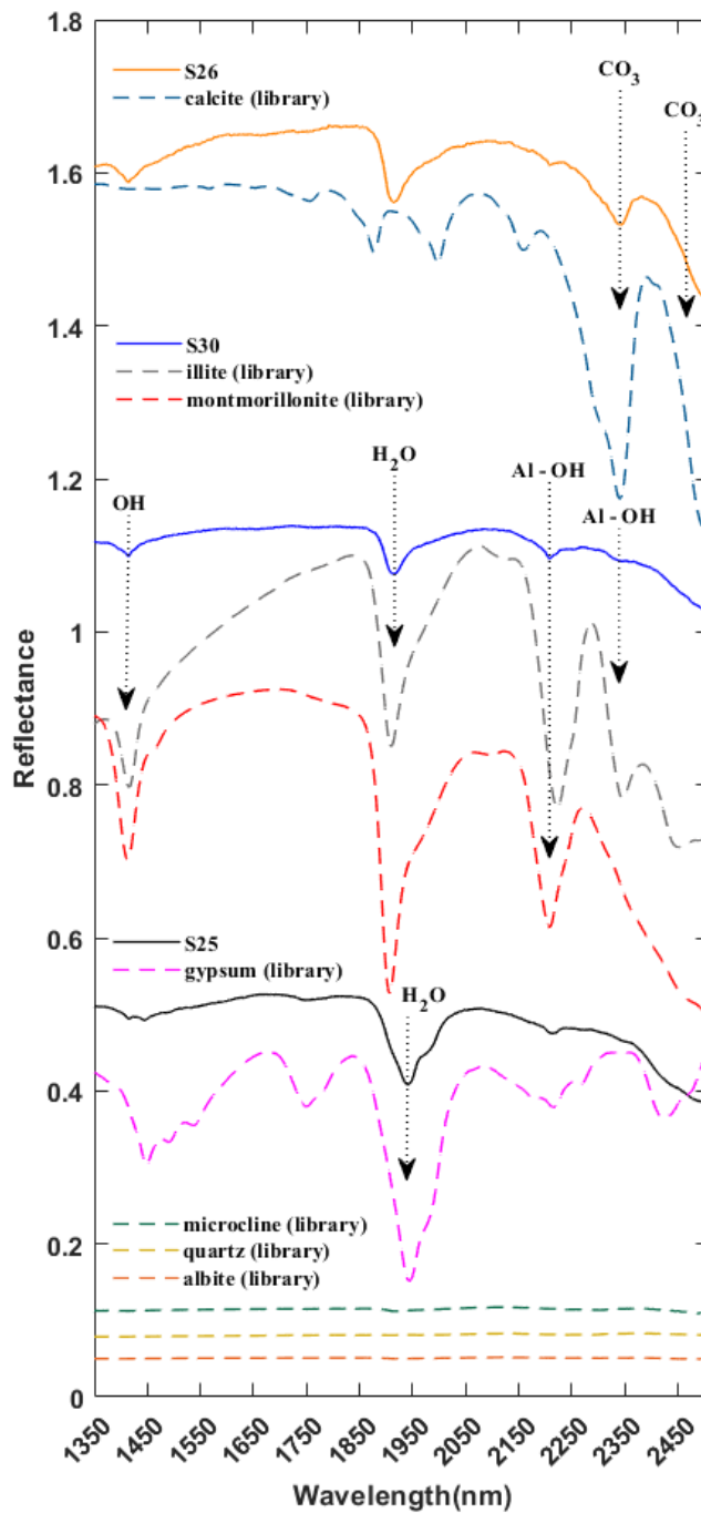
160 Figure 3. SWIR spectra for three representative samples (S25, S26, S30) and library spectra of pure minerals showing diagnostic features for calcite, montmorillonite, illite, and gypsum. All spectra are offset for clarity. Arrows near 1400, 1900, 2200, and 2345 nm call out features arising from OH, water, and Al-OH in mineral structures, common to many clay minerals such as montmorillonite and illite. Arrows targeting 2340 and 2480 nm show the wavelengths of dominant absorption features in calcite. Arrow at 1945 nm represents the unique spectral signature attributed to water in sulfates such as gypsum.
