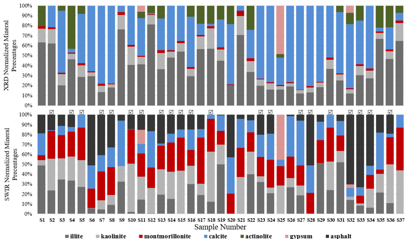
320 Figure 10. Bar charts show XRD (top) and SWIR (bottom) normalized abundances after removing the transparent minerals. Those samples with check marks had relatively well-modelled spectral fit (e.g., Figs. 6a and 6b) as described in the text, and are used for subsequent comparison as described in Sect. 3.3.
