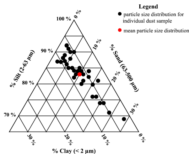
Figure 5. Ternary diagram showing volume distributions for 37 dust samples analysed with Malvern Mastersizer 3000. Silt is the most prevalent size class in the samples with a minimum \sim 69\% and maximum \sim 93\% .
