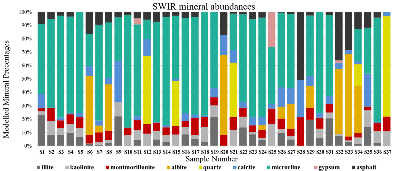
305 Figure 9. Bar charts shows the relative mass fraction (%) calculated from a linear combination of SSA of minerals and asphalt. The unrealistically large proportions of microcline, quartz, and albite is discussed in the text.
