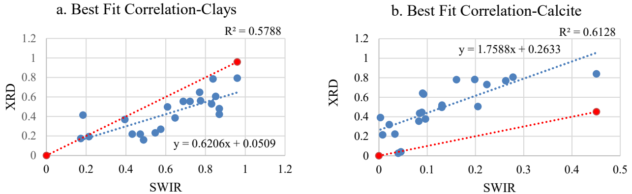
340 Figure 11. Plots display the difference between abundance values in wt. % derived from XRD and SWIR. Data and the best fit line are in blue, a 1:1 correspondence is shown in red. In (a) clay abundances obtained from SWIR demonstrate a relatively higher value suggesting underestimation by the XRD. In (b) the SWIR derived abundances strongly underestimate the amount of calcite compared to XRD.
