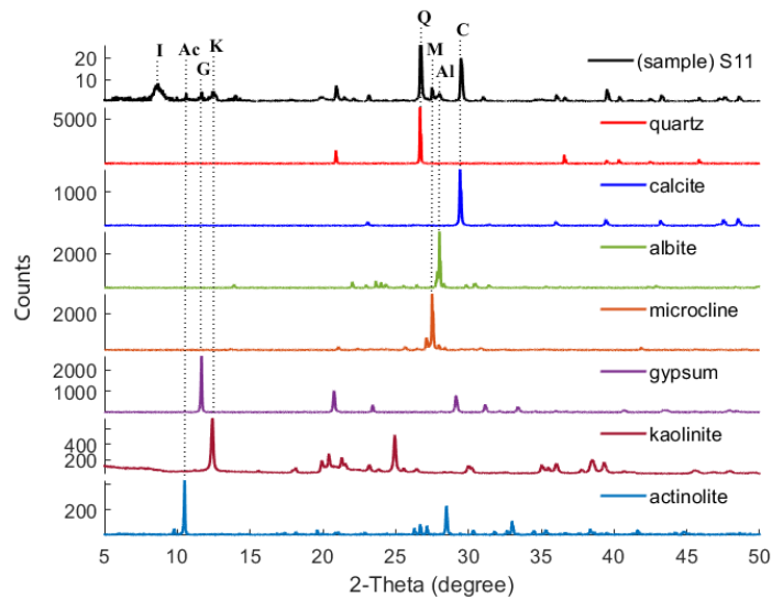
130 Figure 2. XRD pattern of sample S11 is compared with those of standard reference minerals from AMCS. Dotted lines connect the diagnostic XRD peak in quartz (Q), calcite (C), albite (Al), microcline (M), gypsum (G), kaolinite (K), and actinolite (Ac) to the corresponding XRD patterns in S11 confirming the presence of these minerals in this particular dust sample. Illite (I) was identified as described in the text.
