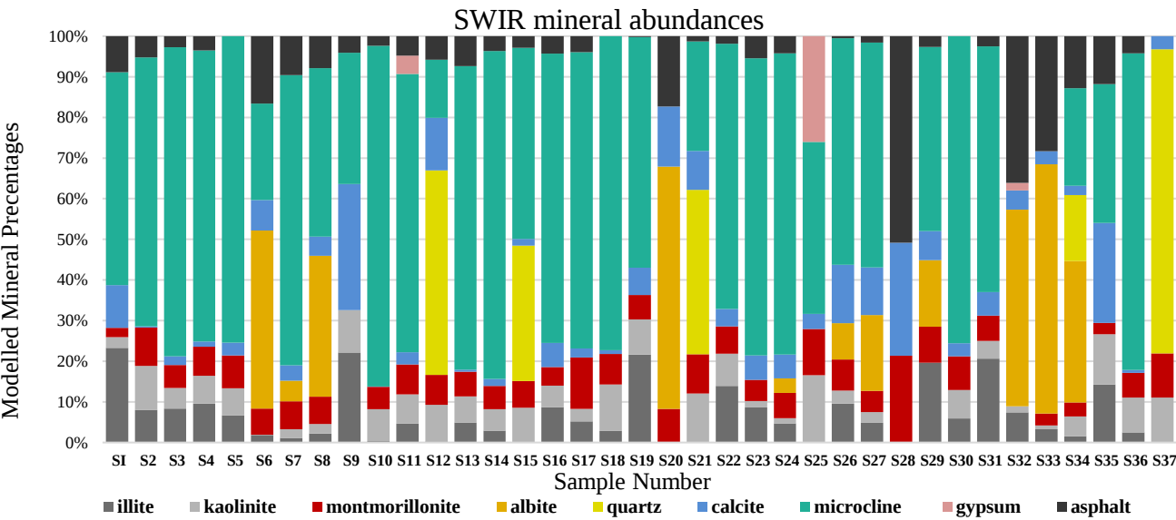
Figure 9. Bar charts show the relative mass fraction (%) calculated from a linear combination of SSA of minerals and asphalt. The unrealistically large proportions of microcline, quartz, and albite is discussed in the text.
