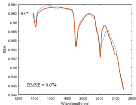
500 Figure C1. Spectral model fit (red line) and RMSE are shown for all 37 dust samples SSA spectra (blue line). Check marks represent the relatively well model fits based on visual inspection and relatively low RMSE.
