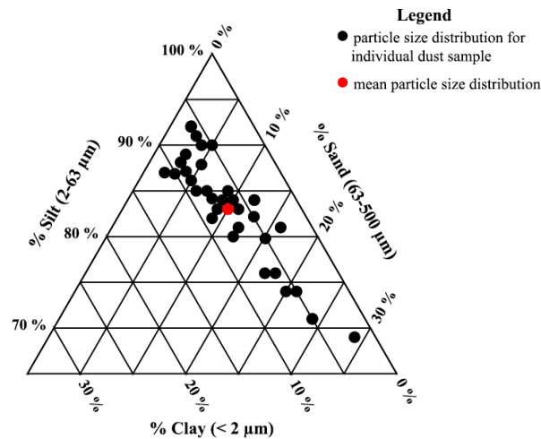
195 Figure 5. Ternary diagram showing volume distributions for 37 dust samples analysed with Malvern Mastersizer 3000. Silt is the most prevalent size class in the samples with a minimum ~ 69 % and maximum ~ 93 %.
