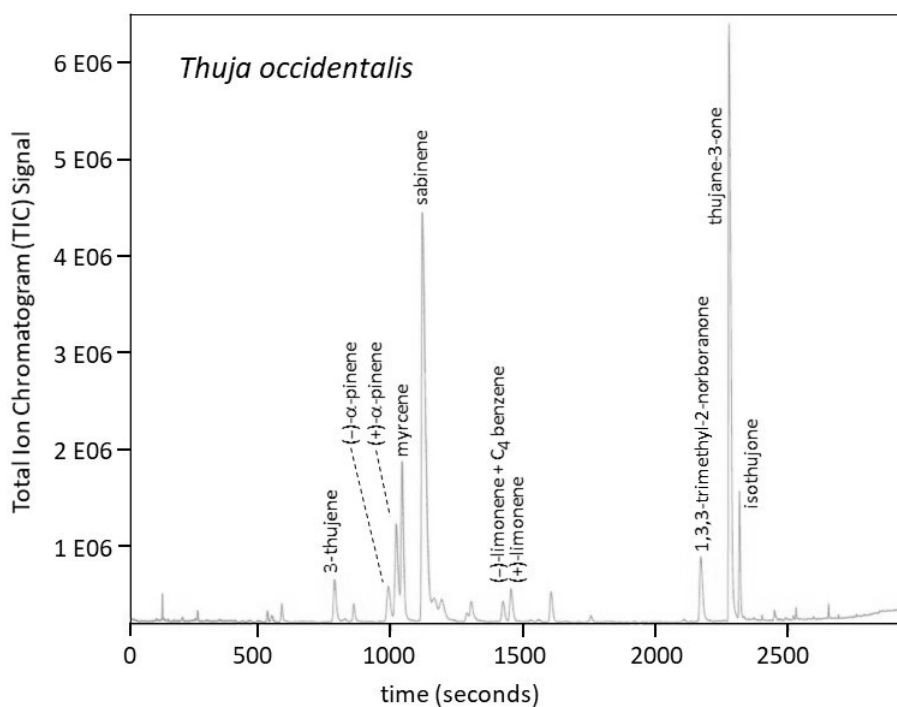
361 Figure 1. Total ion chromatogram (TIC) by GC/MS (gas chromatography/mass spectrometry) 362 using a Supelco Beta DEX™ 120 chiral capillary column (0.25 \mu m film thickness, 0.25 mm 363 i.d., and 30 m long; Supelco Inc., Bellefonte, PA) for a T. occidentalis sample. The peak 364 marked for (-)-limone contains a contribution from an unidentified C 4 -benzene. The two \alpha - 365 pinene enantiomers and the two limonene enantiomers were quantitated using the ion m/z = 93 .
