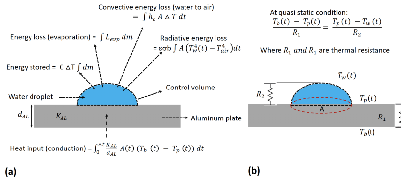
Figure 2. Schematic of energy conservation of control volume across hydrometeor. (a) Distribution of heat gain and loss from the hydrometeor. (b) Schematic of heat flow between the series combination the hotplate and water droplet at quasi static condition.
