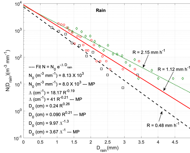
Figure 14. Size distributions of raindrops for different fall rates measured in Red Butte Canyon. Approximately 2000 raindrops were considered in each case binned in increments of \approx 0.2 mm. Distribution of raindrops (points) on a plot of log number vs diameter of raindrops ( D_{rain} ), fitted using N(D_{rain}) = N_0 e^{-\Lambda D_{rain}} (lines). R is SWE rate of rainfall ( SWE ) and D_0 is median of diameter of raindrops. Fitted results are compared with Marshall and Palmer (1948), abbreviated as MP.
