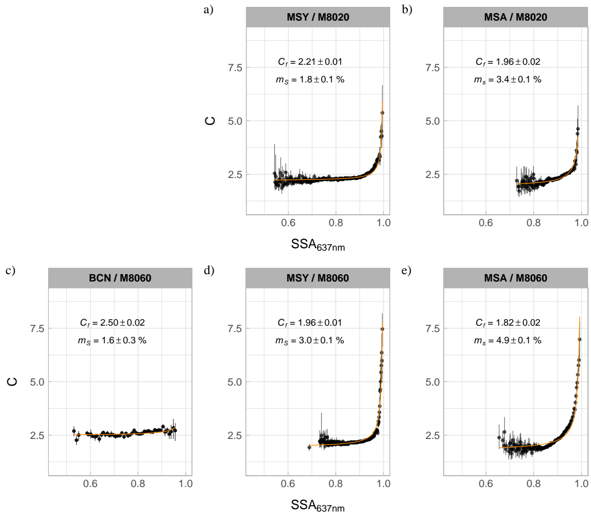
Figure 1. Cross-sensitivity to scattering analysis for TFE-coated glass tape (also known as M8020, upper panel) and M8060 filter tape (lower panel) for BCN (c), MSY (a,d) and MSA (b,e) stations obtained by attenuation coefficients from the AE33, absorption coefficients from the MAAP photometer and scattering coefficients from the integrating nephelometer. Each data point represents the mean, and the vertical bars the first and third quartile for each bin. Multiple scattering constant, C_f and cross-sensitivity to scattering, m_s , are determined by fitting eq. (9) to the binned data.
