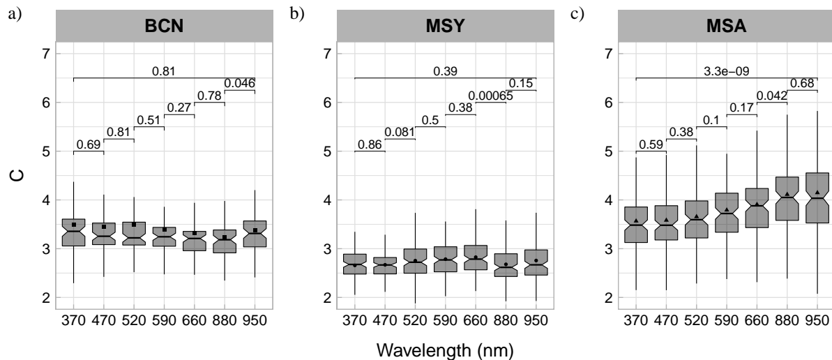
Figure 4. Wavelength dependence of C at BCN, MSY and MSA comparing b_{atn} from the AE33 measured at each wavelength and b_{abs} inter/extrapolated to the same wavelength from the PP_UniMI. Box plots have been obtained as in Fig. 3 with the addition of the mean value of the distribution for each wavelength represented by a marker. The values above the box plots between adjacent wavelengths and between 370 and 950 nm wavelength box plots show the obtained p-values, with p < 0.05 meaning a statistically significance difference.
