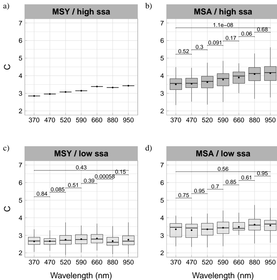
Figure 5. Wavelength dependence of C at MSY (a,c) and MSA (b,d) obtained comparing b_{atn} from the AE33 measured at each wavelength and b_{abs} inter/extrapolated to the same wavelength from the PP_UniMI. Box plots have been obtained as in Fig. 3 and separated into two categories depending whether the SSA was above (high ssa, upper panel) or below (low ssa, lower panel) the threshold at which C sharply increases. As in Fig. 3, the values above the box plots between adjacent wavelengths and between 370 and 950 nm wavelength box plots show the obtained p-values, with p < 0.05 meaning a statistically significance difference.
