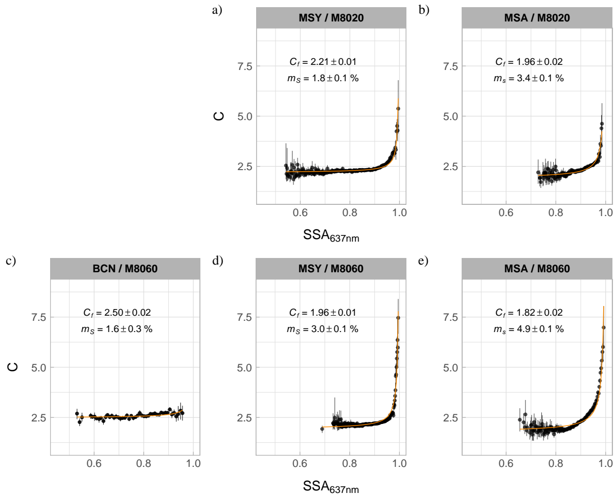
Figure 1. Cross-sensitivity to scattering analysis for TFE-coated glass tape (also known as M8020, upper panel) and M8060 filter tape (lower panel) for BCN (c), MSY (a,d) and MSA (b,e) stations obtained by attenuation coefficients from the AE33, absorption coefficients from the MAAP photometer and scattering coefficients from the integrating nephelometer. Each data point represents the mean, and the vertical bars the first and third quartile for each bin. Multiple scattering constant, C_f and cross-sensitivity to scattering, m_s , are determined by fitting eq. (9) to the binned data.
