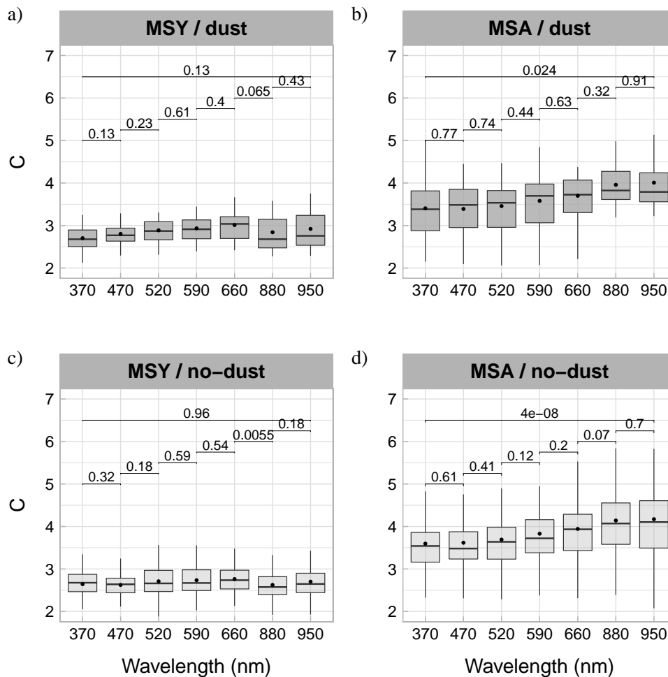
Figure 6. Wavelength dependence of C at MSY (a,c) and MSA (b,d) obtained comparing b_{atn} from the AE33 measured at each wavelength and b_{abs} inter/extrapolated to the same wavelength from the PP_UniMI. Box plots have been obtained as in Fig. 3 and separated into two categories depending whether Saharan dust outbreaks took place (dust) or not (no-dust). As in Fig. 3, the values above the box plots between adjacent wavelengths and between 370 and 950 nm wavelength box plots show the obtained p-values, with p < 0.05 meaning a statistically significance difference.
