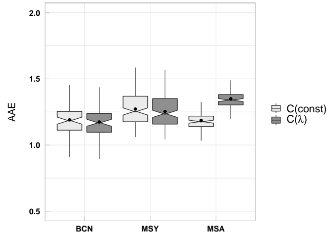
Figure 7. The absorption Ångström exponent (AAE) calculated with a constant C(\text{const}) and the wavelength-dependent C(\lambda) for all stations. Box plots have been obtained as in Figs. 3 and 4, with the markers indicating the mean AAE values.
