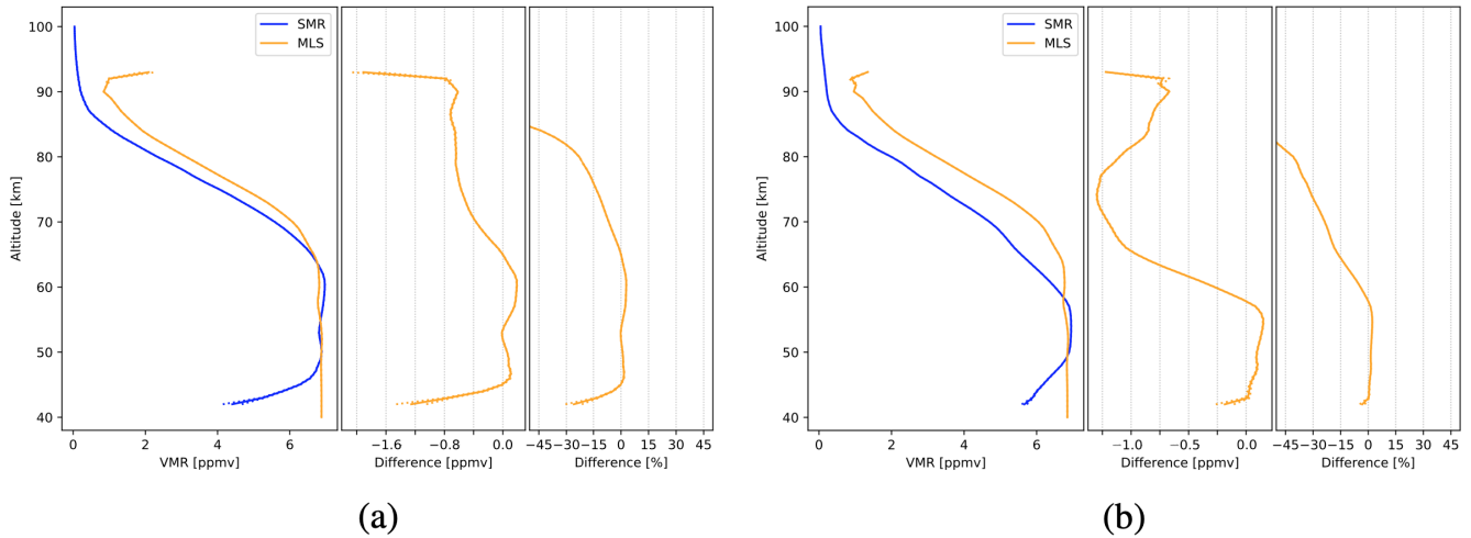
Figure 11. Comparison of SMR \text{H}_2\text{O} concentrations profiles, from FM13 (a) and FM19 (b), with the ones those from MLS retrievals. The data plotted are global averages over the whole time period between July 2004 and April 2019. Figures characteristics are the same as in Figure 6.
