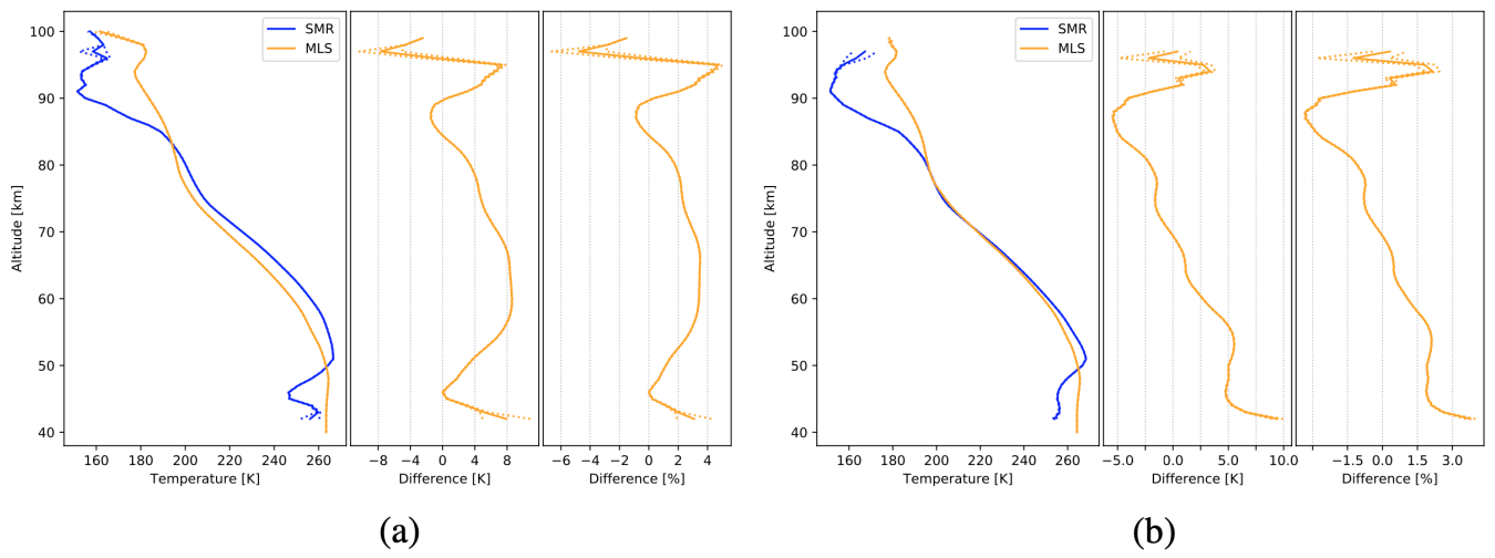
Figure A29. Comparison of SMR temperatures, from FM13 (a) and FM19 (b), with the ones those from MLS retrievals. The data plotted are global averages over the time period between July 2004 and April 2019. Figures characteristics are the same as in Figure 6.
