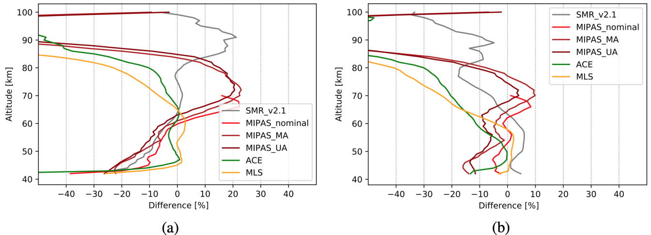
Figure 12. Summary of relative differences of SMR v3.0 \text{H}_2\text{O} concentrations with respect to those from SMR v2.1 ones , as well as those retrieved from measurements by all other instruments considered in this study. For the sake of clarity, errors are not shown. Panel a: FM13 comparison. Panel b: FM19 comparison.
