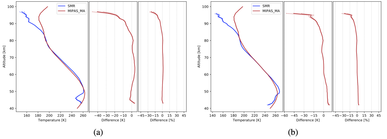
Figure A20. Comparison of SMR temperatures, from FM13 (a) and FM19 (b), with the ones those from MIPAS Middle Atmosphere Mode retrievals. The data plotted are global averages over the whole time periods indicated in Table 2. Figures characteristics are the same as in Figure 6.
