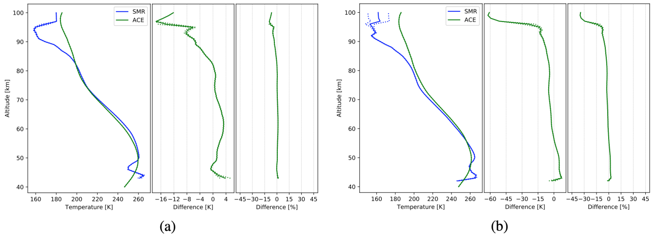
Figure A26. Comparison of SMR temperatures, from FM13 (a) and FM19 (b), with the ones those from ACE-FTS retrievals. The data plotted are global averages over the time period between February 2004 and April 2019. Figures characteristics are the same as in Figure 6.
