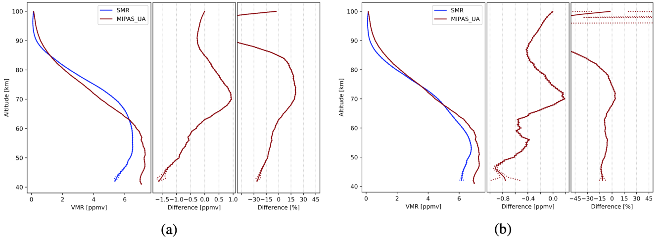
Figure 9. Comparison of SMR \text{H}_2\text{O} concentrations profiles, from FM13 (a) and FM19 (b), with the ones those from MIPAS Upper Atmosphere Mode retrievals. The data plotted are global averages over the whole-time periods indicated in Table 2. Figures characteristics are the same as in Figure 6.
