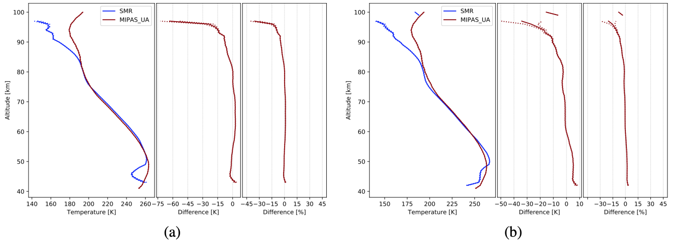
Figure A23. Comparison of SMR temperatures, from FM13 (a) and FM19 (b), with the ones those from MIPAS Upper Atmosphere Mode retrievals. The data plotted are global averages over the whole time periods indicated in Table 2. Figures characteristics are the same as in Figure 6.
