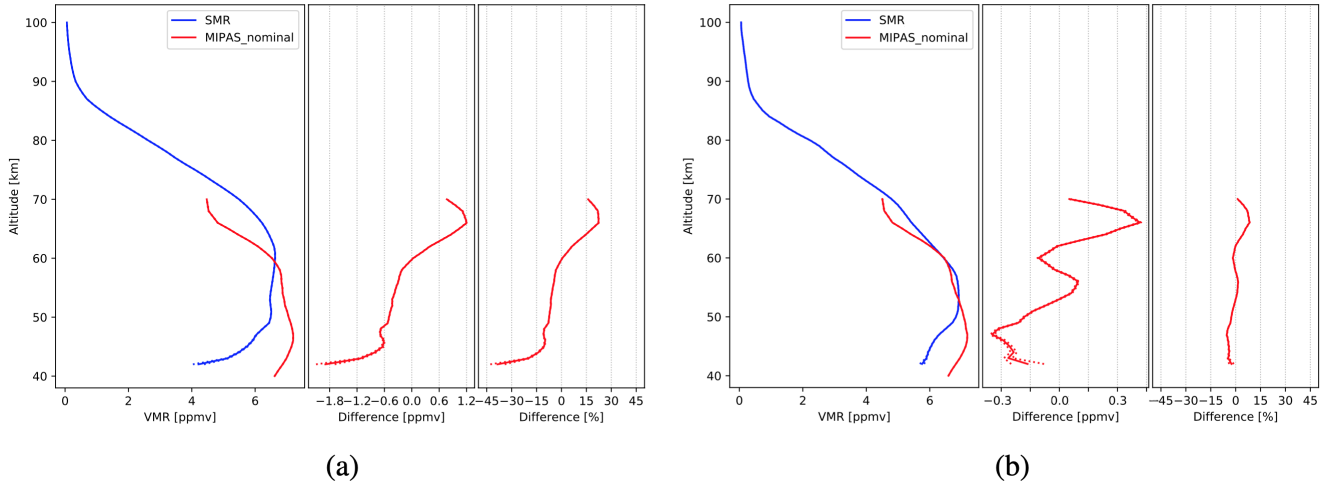
Figure 7. Comparison of SMR H 2 O concentrations profiles , from FM13 (a) and FM19 (b), with the ones those from MIPAS Nominal Mode retrievals. The data plotted are global averages over the whole time between periods indicated in Table 2. Figures characteristics are the same as in Figure 6.
