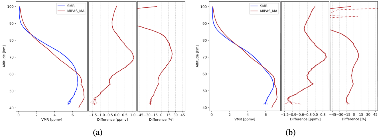
Figure 8. Comparison of SMR \text{H}_2\text{O} concentrations profiles, from FM13 (a) and FM19 (b), with the ones those from MIPAS Middle Atmosphere Mode retrievals. The data plotted are global averages over the whole-time periods indicated in Table 2. Figures characteristics are the same as in Figure 6.
