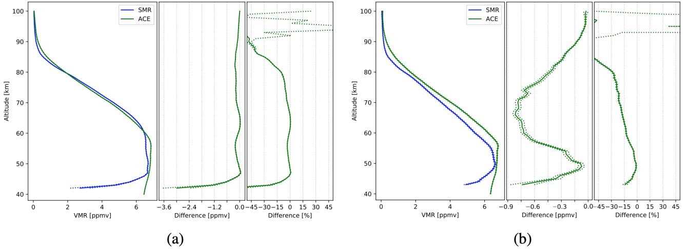
Figure 10. Comparison of SMR \text{H}_2\text{O} concentrations profiles, from FM13 (a) and FM19 (b), with the ones those from ACE-FTS retrievals. The data plotted are global averages over the whole time period between February 2004 and April 2019. Figures characteristics are the same as in Figure 6.
