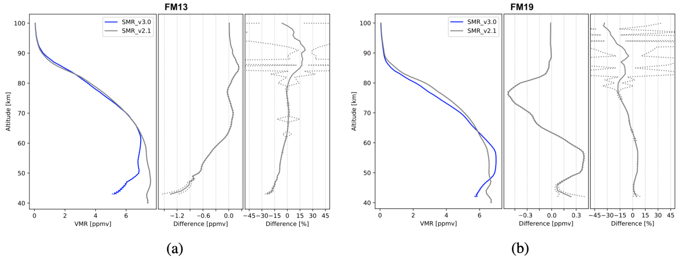
Figure 6. Comparison of SMR v3.0 with respect to v2.1 \text{H}_2\text{O} concentrations profiles, from FM13 (a) and FM19 (b). The data plotted are global averages over the whole-time period between February 2001 and April 2019. Each subfigure consists of three panels. Left panels: volume mixing ratios, expressed in ppmv. Center panels: absolute differences, expressed in ppmv. Right panels: relative differences, expressed in percentage. The differences shown are calculated as medians of the single profiles differences. The dashed lines represent the standard deviation of the median which, in some cases, is smaller than the thickness of the profile line, causing the dashed line not to be distinguishable.
