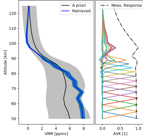
Figure 2. Example retrieval referring to from ScanID 230753751 from FM 19. Left: Retrieved concentration profile and error due measurement thermal noise (Rodgers, 2000) (in blue and shaded, respectively) and a priori including uncertainties (in black and shaded, respectively). Right: Averaging kernels plotted in a different colour for each altitude (not indicated) and measurement response (dashed-dotted black line).
