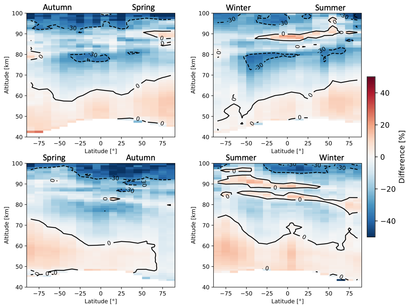
Figure A6. Seasonal zonal means of H 2 O FM19 SMR v3.0–v2.1 relative differences averaged over the whole time period between February 2001 and April 2019. The seasons are intended as astronomical seasons, i.e. starting each at the respective solstice or equinox.
