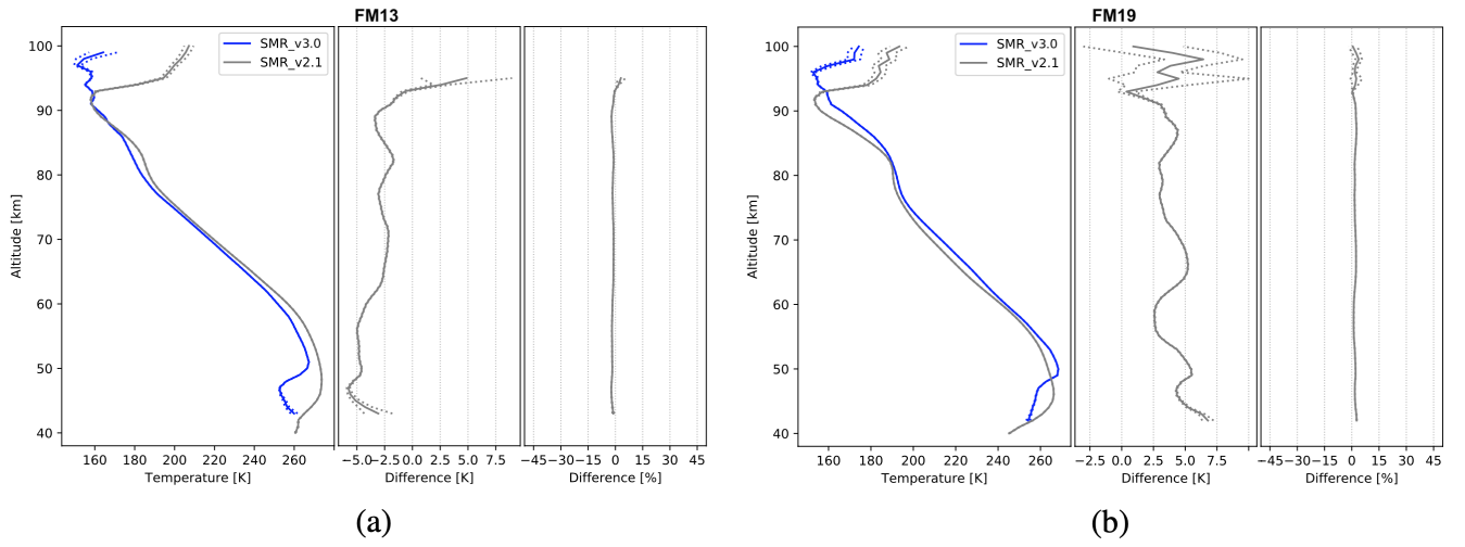
Figure A7. Comparison of SMR v3.0 and v2.1 temperatures from FM13 (a) and FM19 (b). The data plotted are global averages over the whole time period between February 2001 and April 2019. Figures characteristics are the same as in Figure 6.
