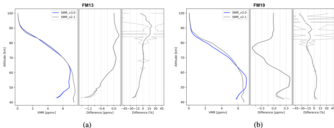
Figure 6. Comparison of SMR v3.0 with respect to v2.1 \text{H}_2\text{O} concentrations, from FM13 (a) and FM19 (b). The data plotted are global averages over the whole time period between February 2001 and April 2019. Each subfigure consists of three panels. Left panels: volume mixing ratios, expressed in ppmv. Center panels: absolute differences, expressed in ppmv. Right panels: relative differences, expressed in percentage. The differences shown are calculated as medians of the single profiles differences. The dashed lines represent the standard deviation of the median which, in some cases, is smaller than the thickness of the profile line, causing the dashed line not to be distinguishable.
