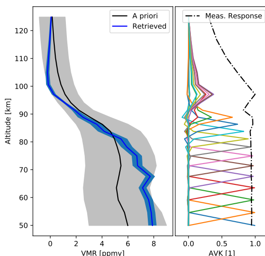
Figure 2. Example retrieval referring to ScanID 230753751 from FM 19. Left: Retrieved concentration profile and error due to measurement thermal noise (Rodgers, 2000) (in blue and shaded, respectively) and a priori including uncertainties (in black and shaded, respectively). Right: Averaging kernels plotted in a different colour for each altitude (not indicated) and measurement response (dashed-dotted black line).
