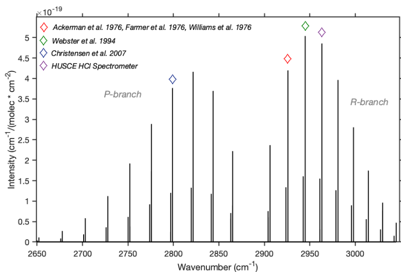
Figure 1: Line intensities of fundamental transition of HCl. The relatively smaller line that accompanies each larger line represents transition of H 37 Cl. The purple diamond indicates the transition that the current instrument uses to measure HCl. The red, green, and blue diamonds indicate transitions utilized by past measurements of stratospheric HCl.
