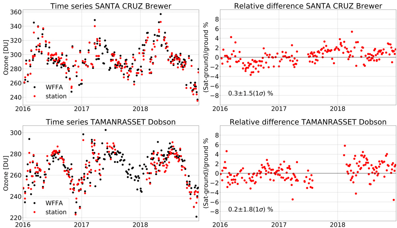
Figure 6. Left panels: Examples of daily mean total ozone time series from ground-based measurements (red) and co-located WFFA TOC (black) from 2016 to 2018, in Santa Cruz (28.42° N, 16.26° W) and Tamanraset (22.80° N, 5.52° E). Right panels: Percentage differences between WFFA and ground-based data. Mean relative difference and its standard deviation are indicated.
