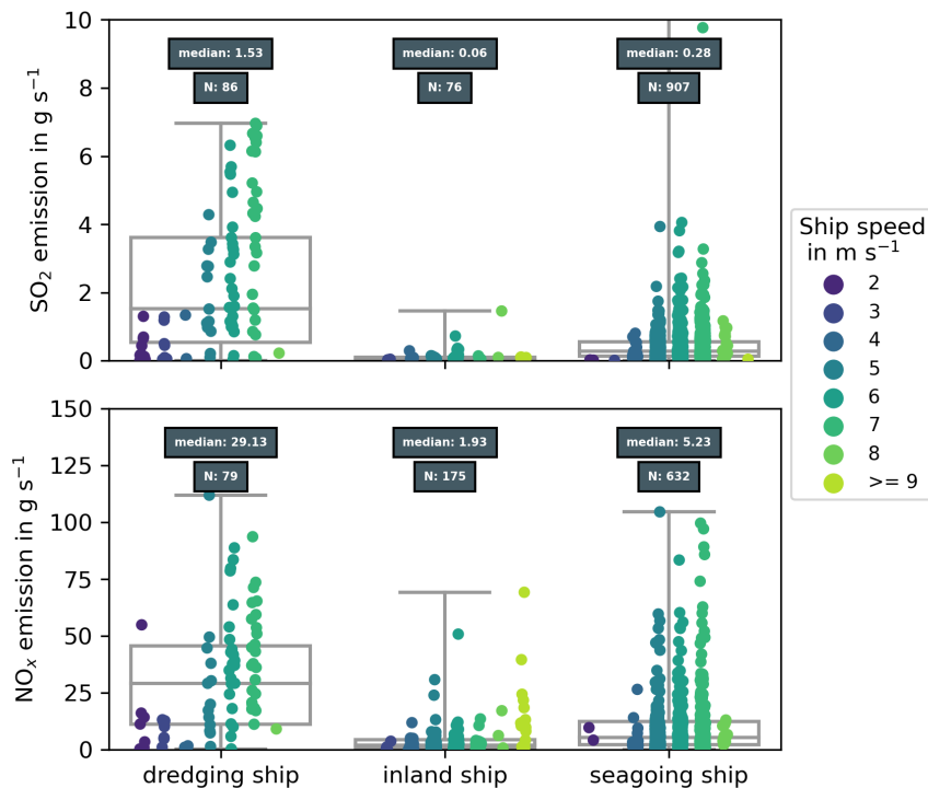
Figure 6. Box plot of SO 2 and NO x emission rates in g s -1 for different ship types. Boxes indicate the 25% and 75% percentile, the line in the middle is the median and the bars show minimum and maximum values. Dots show individual measurements and are colour coded by corresponding ship speed. Dark grey boxes show the median emission rate and total number of observations for each ship type.
