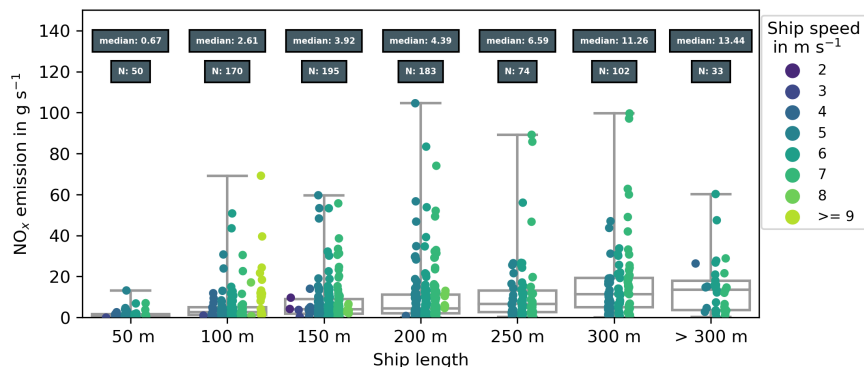
Figure 7. Box plot of NO x emission rates in g s -1 for different ship lengths. Boxes indicate the 25% and 75% percentile, the line in the middle is the median and the bars show minimum and maximum values. Dots show individual measurements and are colour coded to corresponding ship speed. Dark grey boxes show the median emission rate and total number of observations for this length class. Data of dredging ships has been excluded.
