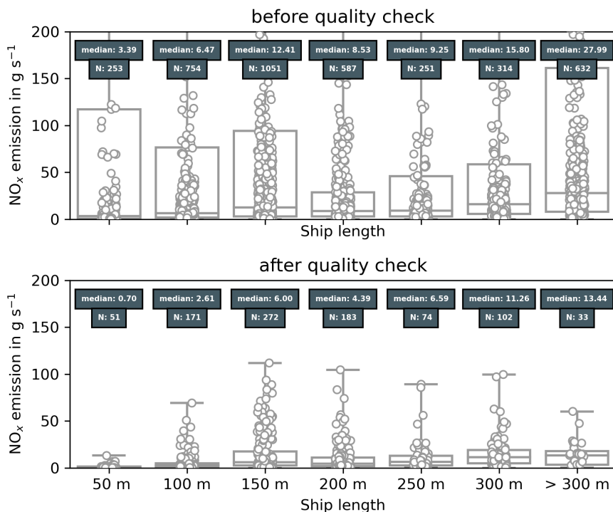
Figure 4. Box plot of \text{NO}_x emission rates in \text{g s}^{-1} for different ship sizes. Boxes indicate the 25% and 75% percentile, the line in the middle is the median and the bars show minimum and maximum values. Dots show individual measurements. Dark grey boxes show the median emission rate and total number of observations for this length class.
