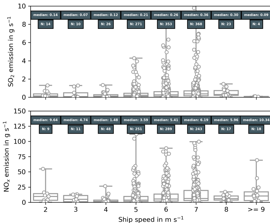
Figure 8. Box plot of SO 2 and NO x emission rates in g s -1 for different ship speeds. Boxes indicate the 25% and 75% percentile, the line in the middle is the median and the bars show minimum and maximum values. Dots show individual measurements. Boxes show the median emission rate and total number of observations for each ship speed.
