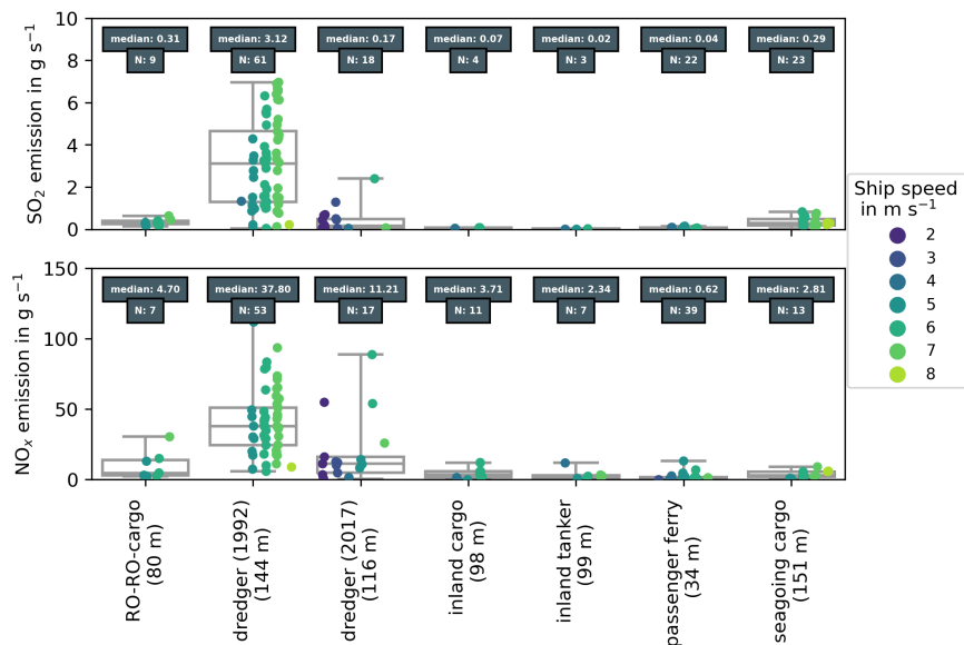
Figure 5. Box plot of SO 2 and NO x emission rates in g s -1 for individual ships, their respective length is given in brackets. Boxes indicate the 25% and 75% percentile, the line in the middle is the median and the bars show minimum and maximum values. Dots show individual measurements and are colour coded by corresponding ship speed. Dark grey boxes show the median emission rate and total number of observations for this ship.
