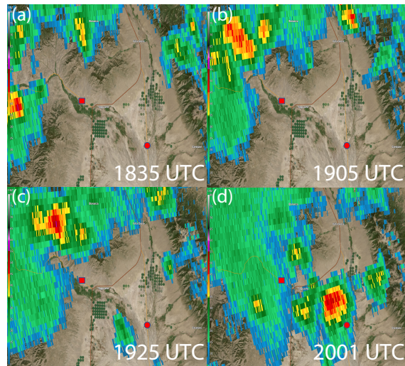
Figure 7. 0.5° level reflectivity (dBZ) from the KPUX radar in Pueblo, CO over the SLV on 15 July 2018. Red square indicates the K04V site and red circle indicates MOFF. a) 1835 UTC (1235 MDT) b) 1905 UTC (1305 MDT) c) 1925 UTC (1325 MDT) d) 2001 UTC (1401 MDT)
