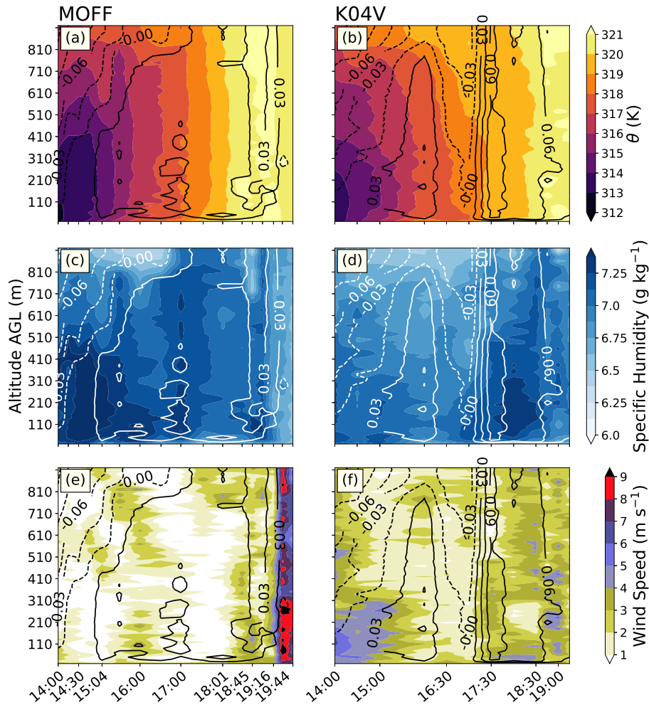
Figure 8. Same as Fig. 3 but on 15 July 2018 and (a,c,e) are at the MOFF site and (b,d,f) are at the K04V site.
