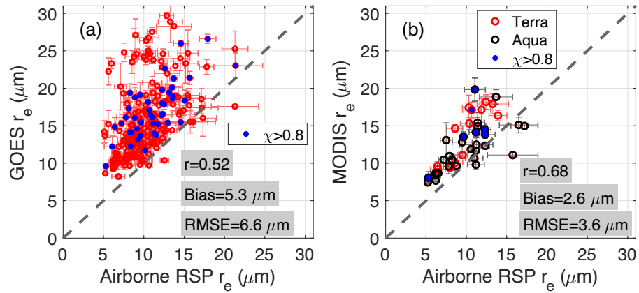
630 Figure 5: Relationship between airborne RSP r_e and (a) GOES-13 and (b) MODIS. Statistics for MODIS combine data from Aqua and Terra. Error bars denote the spatial standard deviation. Blue circles denote retrievals derived over highly heterogeneous cloud scenes.
