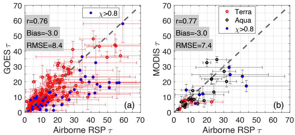
Figure 6: As Figure 5, but for the comparison between airborne RSP \tau and (a) GOES-13 and (b) MODIS.
