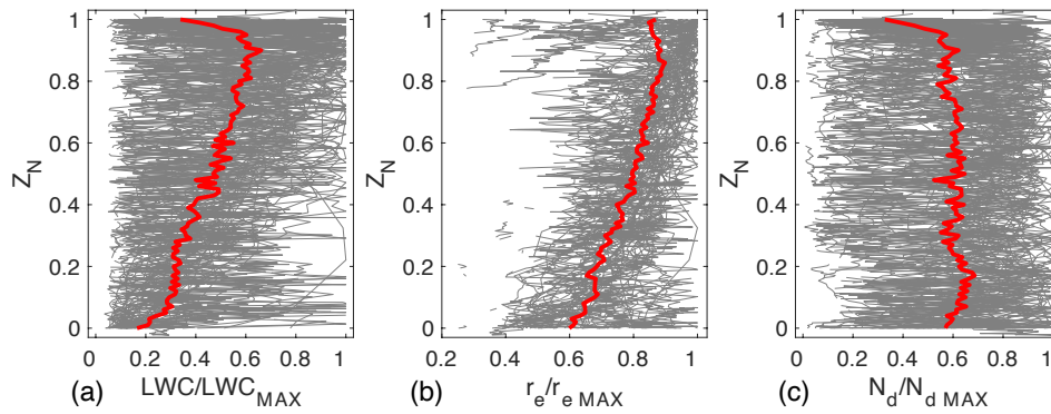
610 Figure 3: CDP profiles normalized by their maximum value from the three NAAMES campaign: a) of liquid water content, (b), r_e , and c) cloud droplet number concentration N_{dMAX} . Normalized height ( Z_N ) corresponds to 0.0 for cloud base and 1.0 for cloud top height. Individual and mean profiles are depicted in gray and red, respectively.
