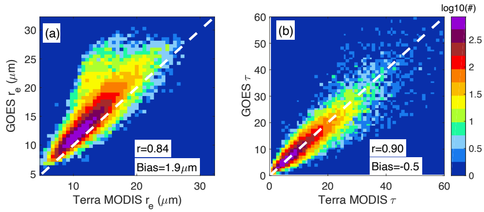
Figure 7: Bivariate histogram between Terra MODIS and GOES-13 a) r_e and b) \tau . 1-to-1 line is denoted by the white dashed lines. Bias represents the mean difference between GOES-13 and MODIS.
