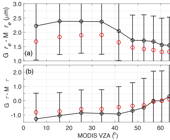
670 Figure 9: Mean differences between GOES and Aqua/Terra MODIS retrievals binned in MODIS VZA 675 deciles: a) cloud effective radius, and b) cloud optical depth. Error bars denote the standard deviation, and median values are represented by red circles.
