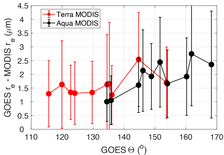
680 Figure 10: r_e differences between GOES-13 and Terra MODIS (red) and Aqua MODIS (black) binned in deciles of GOES-13 scattering angle ( \Theta ). Error bars represent the root mean square difference for each bin.
