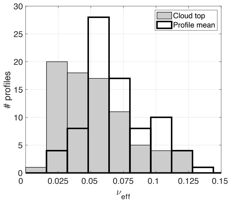
690 Figure 12: Histogram of computed effective variance ( \nu_{\text{eff}} ) assuming a modified gamma distribution, for CDP values sampled near the cloud top (filled gray) and averaged throughout the cloud profile (black).
