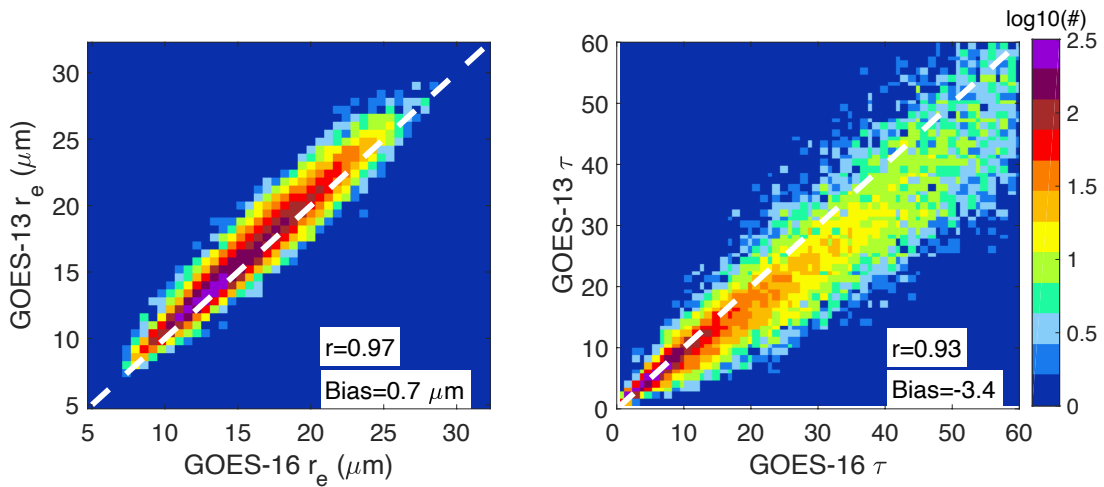
685 Figure 11: Relationship between 30-min GOES-16 ABI and GOES-13 cloud retrievals for 5 days of December 2017 (20, 22, 24, 26, 28) over the North Atlantic for solar zenith angle <75^\circ : a) cloud effective radius and b) cloud optical depth. The bias is defined as the mean difference between GOES-13 and GOES-16 retrievals.
