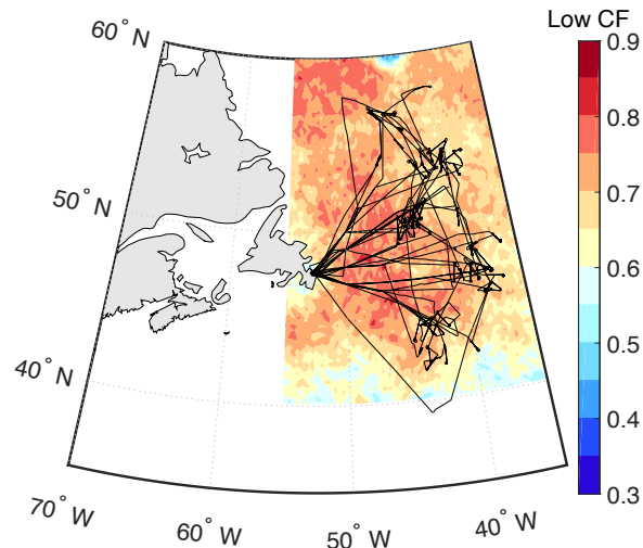
595 Figure 1: Mean Aqua-MODIS low-cloud cover and aircraft tracks (black lines) during the three NAAMES campaigns in November 2015, May 2016, and September 2017.
