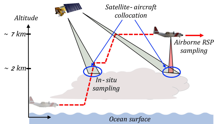
600 Figure 2: Collocation method between satellite and airborne in-situ (CDP probe) and RSP observations. Satellite pixels are paired with in-situ samples collected during profiling maneuver, whereas satellite and RPS data are collocated for high altitude aircraft transects (~ 7 km)
