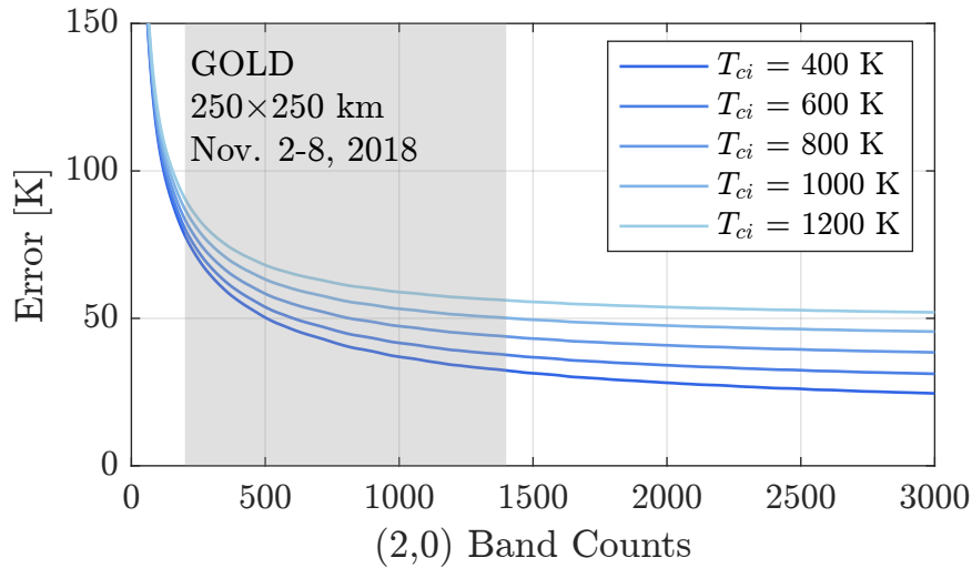
550 Figure 4: Total T_{ci} random measurement error (not including particle noise) and representativeness error for the (2,0) band. The range of (2,0) band counts for GOLD data (250 \times 250 km resolution at nadir) used in the case study in Section 4 is highlighted by the grey box.
