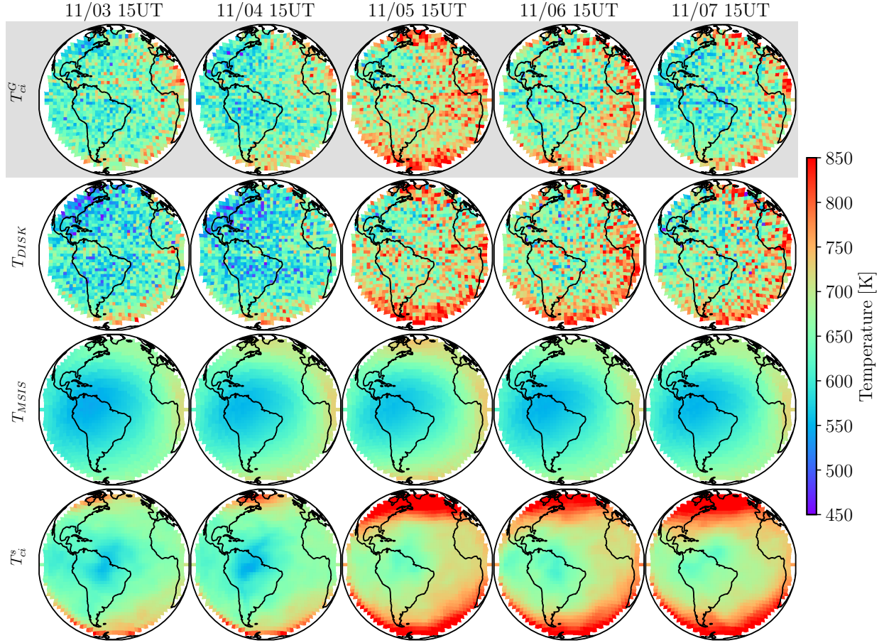
Figure 7: Comparison of T_{ci}^G with T_{DISK} , T_{MSIS} , and T_{ci}^s over Earth's disk viewed by GOLD for a five-day window from 3–7 November 2018 at about 15 UT, noon LT at the center of the disk (47.5°W, 0°N). A small geomagnetic storm has commenced the evening of 4 November and lasted through 5 November.
