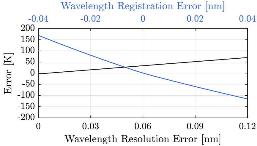
545 Figure 3: Expected bias errors in T_{ci} as a function of the two dominant known sources systematic measurement errors: the instrument's wavelength registration (blue) and variations in the wavelength resolution (black).
