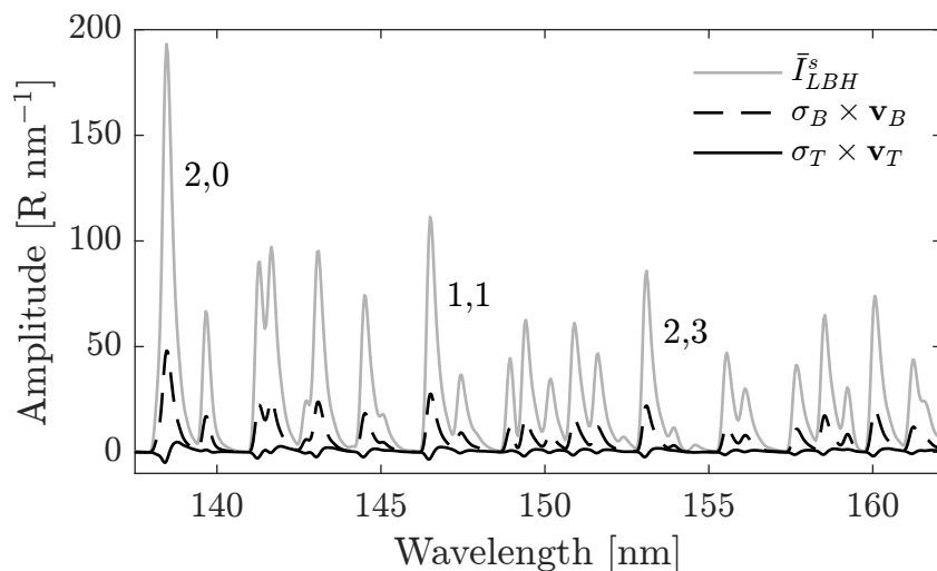
Figure 1: Simulated top-of-atmosphere mean LBH emissions (gray), \overline{I_{LBH}^s} , and the principal components associated with overall brightening of emissions (dashed black), v_B , and the temperature signal (solid black), v_T , scaled by their respective eigenvalues, \sigma_B and \sigma_T . These two principal components account for 99.9% of the variability about the mean for the period of 2–8 November 2018.
