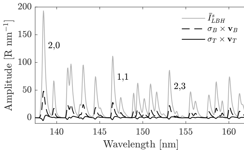
Figure 1: Simulated top-of-atmosphere mean LBH emissions (gray), \overline{I_{LBH}^S} , and the principal components associated with overall brightening of emissions (dashed black), \sigma_B \times \mathbf{v}_B , and the temperature signal (solid black),
