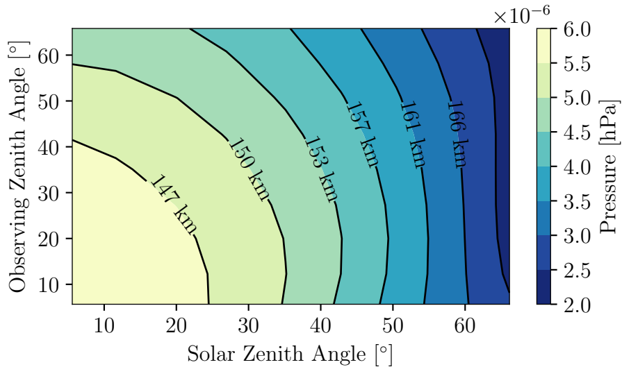
555 Figure 5: Pressure at the peak of the LBH contribution function, p_{\tau=1} , as a function of SZA and OZA determined from forward modeling WAM simulations for the period of 2-8 November 2018 considering realistic forcing conditions. LBH emissions are on constant pressure level surfaces given the solar and observing zenith angles. Approximate corresponding altitudes in the WAM simulations are also provided but note that these altitudes will vary depending on the forcing conditions.
