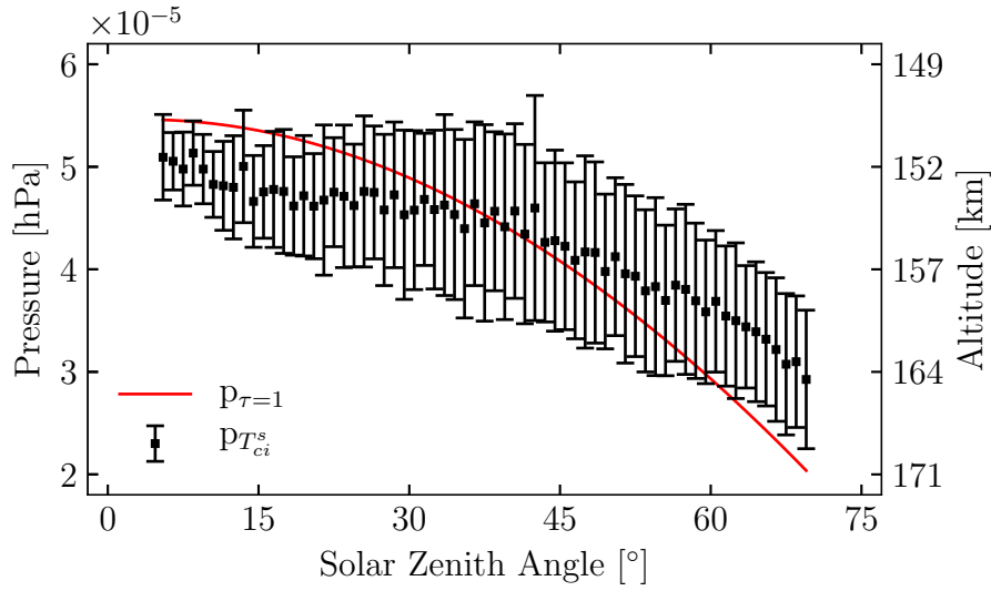
Figure 6: The mean and standard deviation of the pressure for the simulated WAM temperature that is closest to T_{ci}^s , p_{\tau=1} , as a function of SZA averaged over all OZA for the simulation period of 2–8 November 2018 (black). The peak of the LBH contribution function, p_{\tau=1} , is shown as a function of SZA based on forward modeling of LBH disk emissions using the same WAM simulation (red). This peak is constant with respect to pressure level for a given SZA and OZA.
