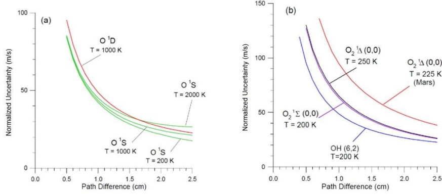
Figure 2. Normalized uncertainty plotted against D (0 to 2.5cm) for several emissions. The O I S emission is shown in green for three temperatures in (a).
