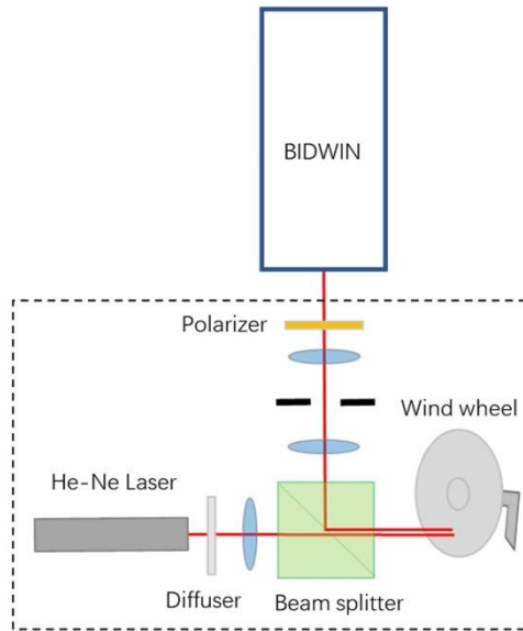
Figure 9. Schematic of the system used to produce a predicable gradient in the LOS wind field within the field of view of the instrument in the lab.
