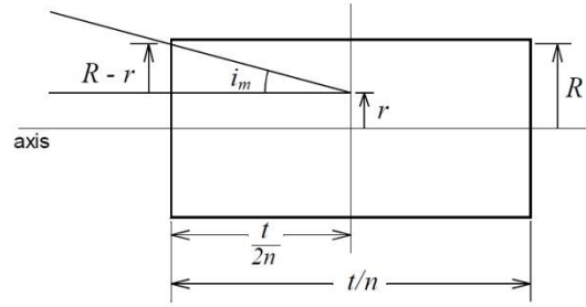
290 Figure 4. The rectangle represents the interferometer, of thickness t . A ray enters near the edge at incident angle i_m and reaches midway at distance r above the axis. R is the available radius at both ends of the interferometer. The thickness is shown as air equivalent, t/n , where n is the refractive index.
