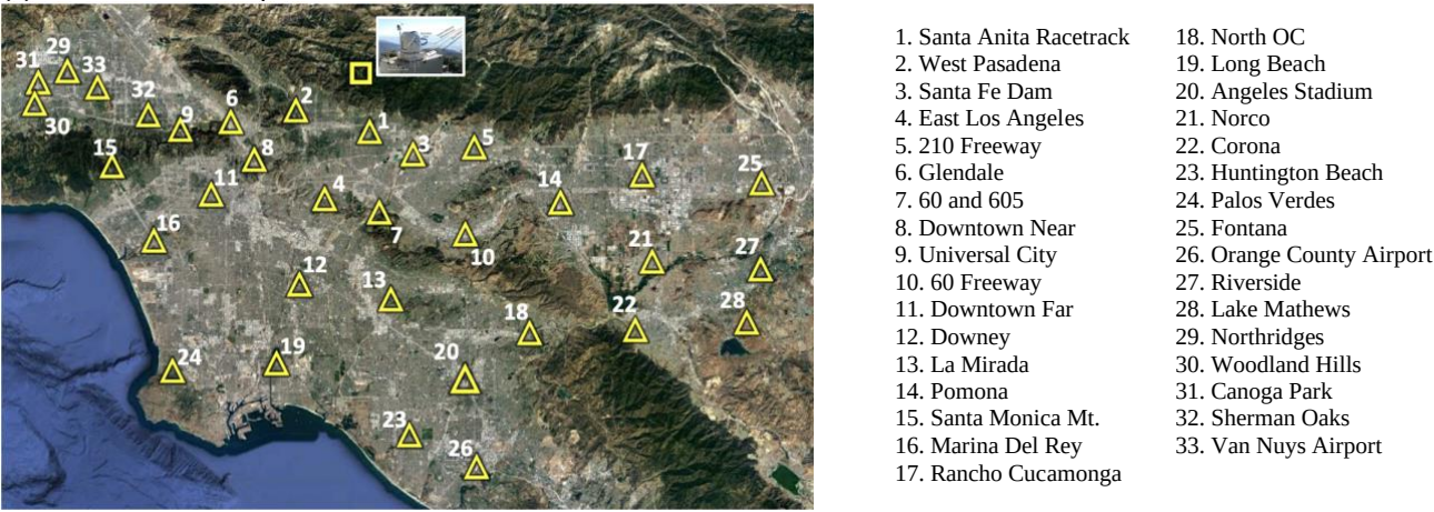
(c) Surface reflection points
