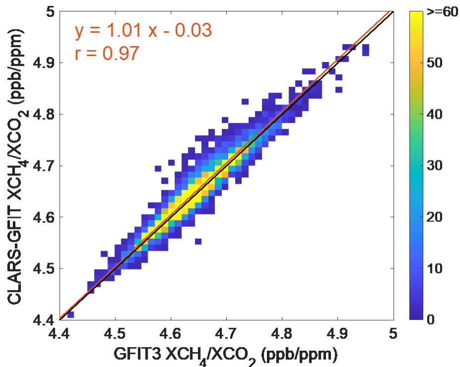
Figure 17. Scatter plot of the \text{XCH}_4/\text{XCO}_2 ratio from GFIT3 and CLARS-GFIT. The 1:1 line is shown in black. The red line denotes the best fit using type II linear regression to fit the data. The equation for the regression fit is also shown.
