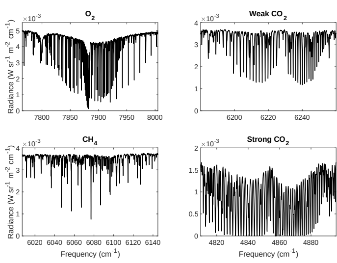
(b) Observed radiance
