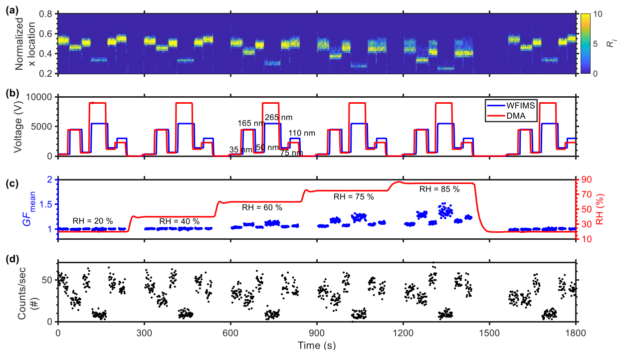
145 Figure 2. Example of the hygroscopic growth measurement sequence of ambient aerosols with six dry sizes (35, 50, 75, 110, 165, and 265 nm) under five RHs (20, 40, 60, 75, and 85%). (a) The number of particles ( R_i ) detected by WFIMS as a function of normalized x -locations within the viewing window and time. (b) The DMA classifying voltage (red line) and WFIMS separator voltage (blue line). (c) RH inside the WFIMS separator and mean growth factor measured by HFIMS as a function of time. (d) Actual particle count rate of HFIMS as a function of time. 150 The particle residence time inside the DMA and the time required for particles to travel from the DMA outlet to the WFIMS separator leads to “dead time” following changes in classified particle size. Given the parabolic flow profile in the tubing, particles travel with a range of velocities inside the HFIMS. As a result, following a change in the DMA classifying voltage, it takes some time for the vast majority of the particles classified at the previous size to exit the system. During this transition 155 concentration at the new size is much lower. Such transition time is common in measurements of size-resolved aerosol hygroscopicity. For example, in DASH-SP, it requires a maximum transition time of 17 s to switch between different DMA-selected sizes (Sorooshian et al., 2008). For traditional HTDMA, a transition time on the order of 20 s is negligible when compared to the long measurement time (i.e., several minutes). However, such transition time rivals the measurement time of HFIMS at each particle size and is one of the main obstacles for fast measurements at multiple sizes. Here the transition time 160 is minimized by optimizing the size sequence as 35 -> 165 -> 50 -> 265 -> 75 -> 110 nm. At an RH of 85% or lower, the maximum range of growth factor (i.e., the ratio of humidified particle diameter to that of dry particles) for atmospheric aerosols is 0.8-2.0 (Gysel et al., 2007). For example, for dry particles of 35 nm, the diameter of humidified particles ranges from 28 to 105 nm. For the next dry size of 165 nm in the sequence, the possible size range of humidified particles is
