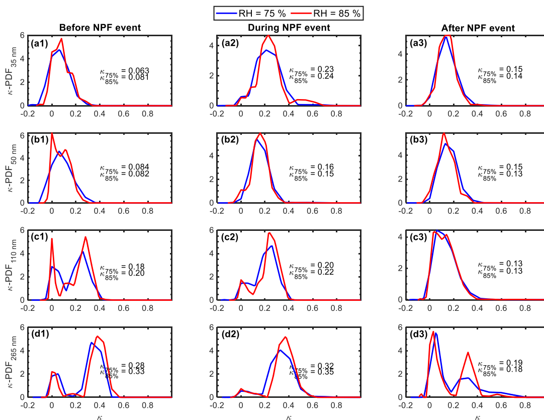
260 Figure 6. Probability density function of hygroscopicity parameter ( \kappa -PDF) before (a1-d1), during (a2-d2) and after (a3-d3) the NPF event period (06:53 am, 09:57 am, and 23:53 pm, respectively) on March 2 nd , 2021. The mean \kappa value derived from each \kappa -PDF is also given in the plots.
