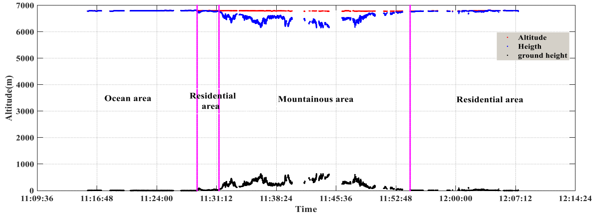
525 Figure 3: Aircraft flight height and corresponding surface elevation on 14 March 2019. The red dots are the altitude of the aircraft measured by the onboard GPS system. The blue scatter points are the distance between the plane and ground measured by lidar. The black scattered points are the difference between the altitude measured by the GPS and the distance measured by the lidar, and also represent the surface elevation. The purple-red vertical line is the dividing line for different surface types.
