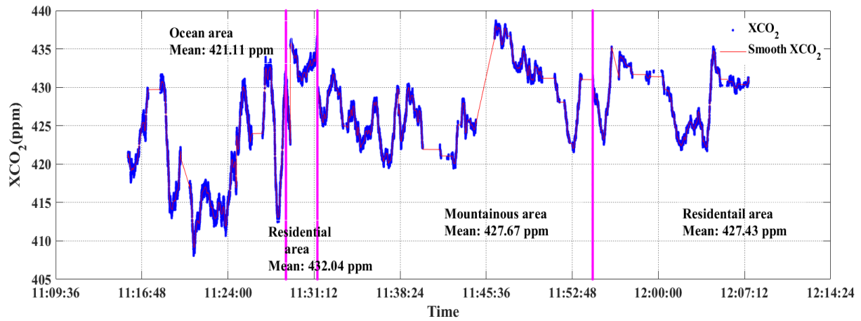
Figure 12: XCO 2 results over ocean, urban residential and mountainous areas on 14 March 2019. The purplish red vertical line represents the boundary of different surface types.
