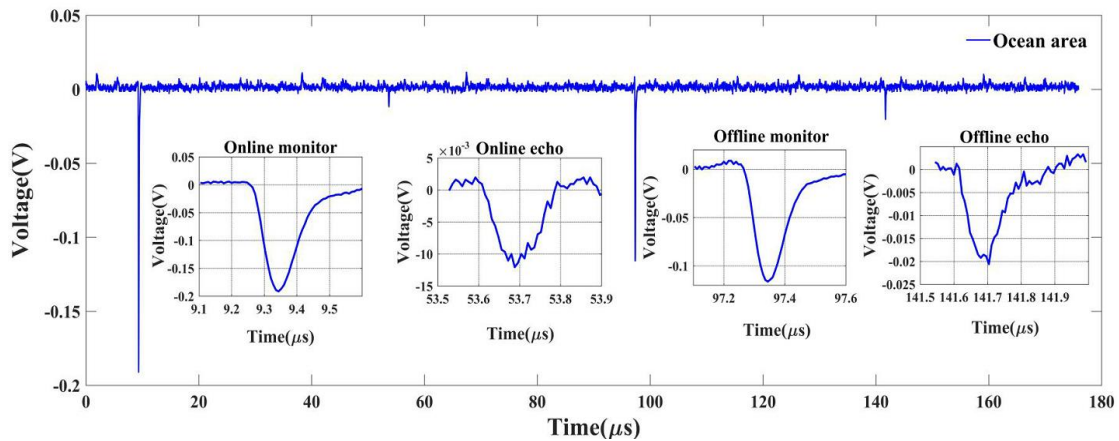
530 Figure 4: Original echo signal of ocean area (total signal and pulse amplification signal). The amplification signals from left to right are online monitor signal, online echo signal, offline monitor signal and offline echo signal.
