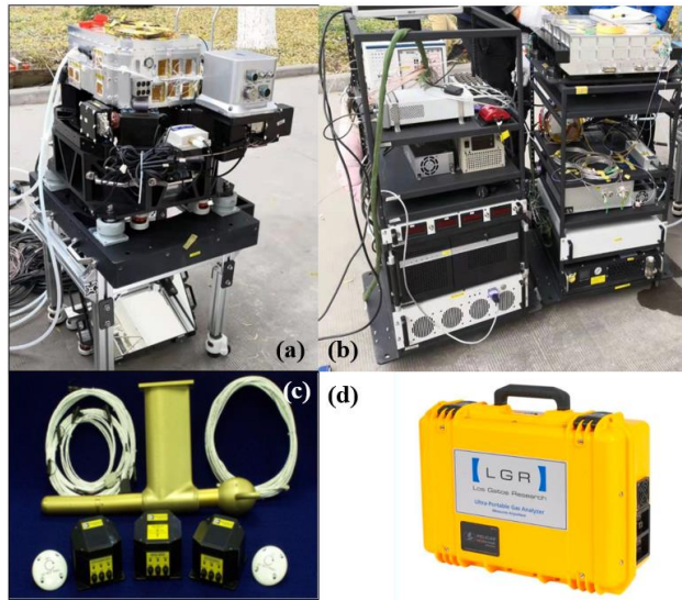
Figure 1: The physical picture of IPDA lidar system. (a) It is the transceiver system, installed in the pod outside the aircraft. (b) It is the control system and data acquisition system of some equipment, which is installed in the sealed cabin of the aircraft. (c) It is the Aircraft Integrated Meteorological Measurement System (AIMMS). (d) It is a commercial instrument Ultraporeable Greenhouse Gas Analyzer, that was installed in an unsealed cabin of the aircraft.
