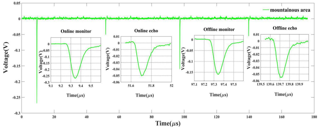
Figure 6: Original echo signal of mountain area (total signal and pulse amplification signal). The amplification signals from left to right are online monitor signal, online echo signal, offline monitor signal and offline echo signal.
