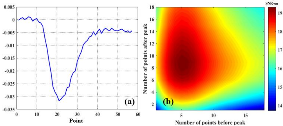
Figure 8: (a) Online wavelength echo pulse signal in land area. (b) The change of the SNR of the echo pulse signal in the land area with the number of selected pulse points.
