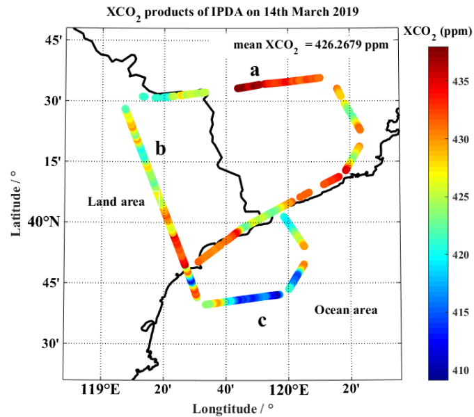
Figure 12: XCO 2 results over ocean, urban residential and mountainous areas on 14 March 2019. The purplish red vertical line represents the boundary of different surface types.
