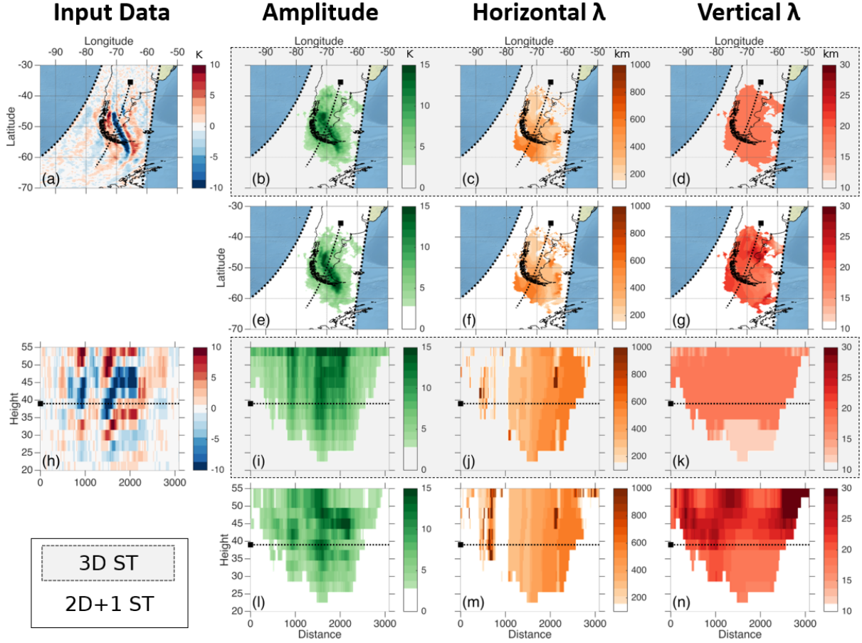
Figure 6. Comparison of 3D ST and 2D+1 ST estimates of GW parameters for a large orographic gravity wave observed in May 2008 over South America. (a) and (h) show original temperature perturbation data, as a map at 39 km altitude and a vertical cut along the instrument track respectively; dotted lines show the location of the other set of panels, with a black square indicating zero-distance on the lower panel. (b-d,i-k) 3DST estimates, (e-g,l-n) 2D+1 ST estimates of (b,e,i,l) wave amplitude, (c,f,j,m) \lambda_h and (d,g,k,n) \lambda_z . Units for each panel are shown above the colourbar at the top of each row. Data have been boxcar-smoothed by 5 voxels in each direction in the horizontal plane before plotting to reduce visible noise. Regions with smoothed output amplitudes below 2.7 K have been removed from all panels except (a) and (h) to focus on wave features only.
