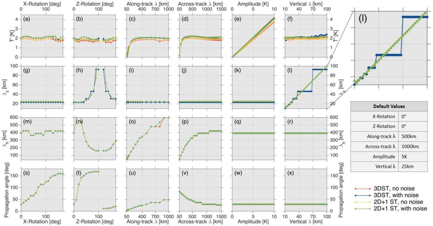
Figure 4. Systematic comparison of the 3DST and 2D+1 ST for a wide range of input artificial waves. Each panel shows recovered (a-f) wave amplitude, (g-l) \lambda_z , (m-r) \lambda_h and (s-x) propagation angle, for the four different analyses indicated at bottom right. For each panel, the parameter named at the top and bottom of the column is varied systematically, with all other parameters set to the default values shown in the table at top right. Note that, in many cases the results for each method are identical, and for these only the last-plotted (2D+1 ST with noise) analysis is visible. (l) is the only test to exhibit significantly different results between the 3DST and 2D+1 ST, and is shown enlarged at top right.
