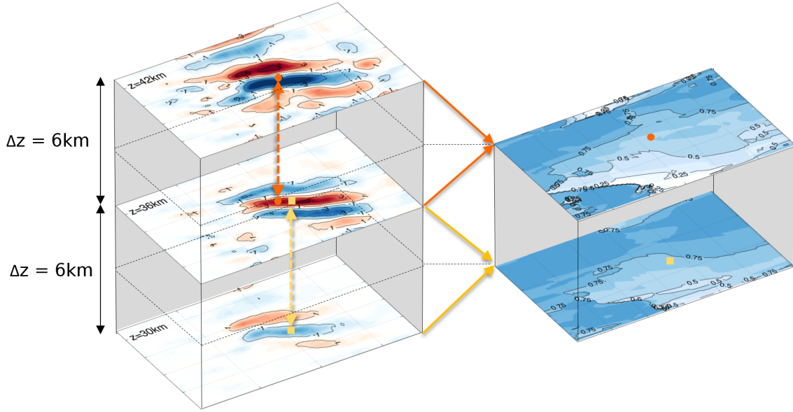
Figure 2. Diagram illustrating the underlying concept of our method. The left column show three horizontal cuts through a large-vertical-scale gravity wave, with a vertical spacing between levels of 6 km. Values shown at each level are the magnitude of a gravity wave signal, with red indicating a positive magnitude and blue a negative magnitude. All units except for height are arbitrary. The right column shows cospectral phase differences between the wave structures at each height, on the same horizontal domain; these are derived from a 2D S-Transform analysis, with contours showing phase difference in units of \pi radians. Yellow and orange arrows and markers indicate examples of how \lambda_z is computed in our analysis, and are explained in the main text.
