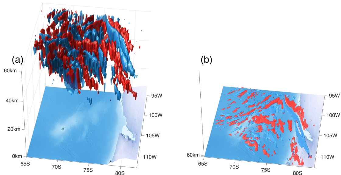
Figure 1. 3D sketches of temperature perturbations associated with a gravity wave observed on the 28th of June 2010 over the Southern Ocean, shown (a) with the vertical axis stretched to highlight wave structure and (b) to true vertical scale. Red/blue isosurfaces enclose the \pm 3.5 K 3D contours respectively. Viewing angle and plotted isosurface magnitudes are identical for both panels.
