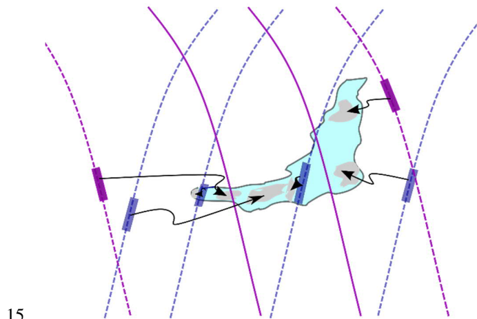
Figure 1. Concept sketch of the use of many CALIOP swaths to determine the height of an SO 2 cloud. Vertical profiles from the daytime CALIOP swaths retrieved simultaneously as the AIRS swaths (purple) is used together with data from CALIOP night-time swaths (blue dashed lines) and daytime CALIOP swaths from other instances (purple dashed lines). Since the volcanic SO 2 cloud is subject to transport, the height information from the non-concurrent swaths is transported using FLEXPART (black arrows) to give a more complete picture of the altitude of the SO 2 cloud (grey areas). 20
