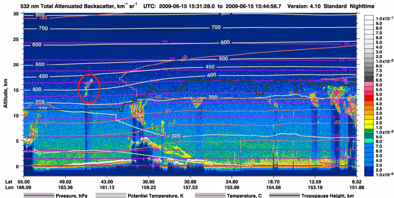
Figure 3: A CALIOP swath containing volcanic aerosol at latitude 46°N and altitudes between 13 and 17 km (red circle). This CALIOP swath is also used in Fig. 5. This figure is part of the CALIOP browse images from NASA.
