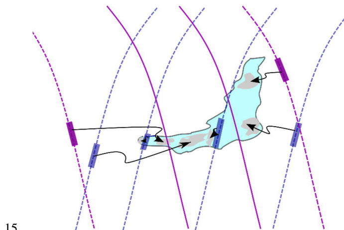
Figure 1. Concept sketch of the use of many CALIOP swaths to determine the height of an SO 2 cloud (shown in light blue). Vertical profiles from the daytime CALIOP orbital tracks retrieved simultaneously as the AIRS swaths (purple) is used together with data from CALIOP night-time orbital tracks (blue dashed lines) and daytime CALIOP orbital tracks from other instances (purple dashed lines). The thick blocks segments on the orbital tracks are the segments where volcanic aerosol is detected. Since the volcanic SO 2 cloud is subject to transport, the height information from the non-concurrent swaths is transported using FLEXPART (black arrows) to give a more complete picture of the altitude of the SO 2 cloud. The grey areas are where FLEXPART trajectories contribute with SO 2 cloud altitude information. 20
