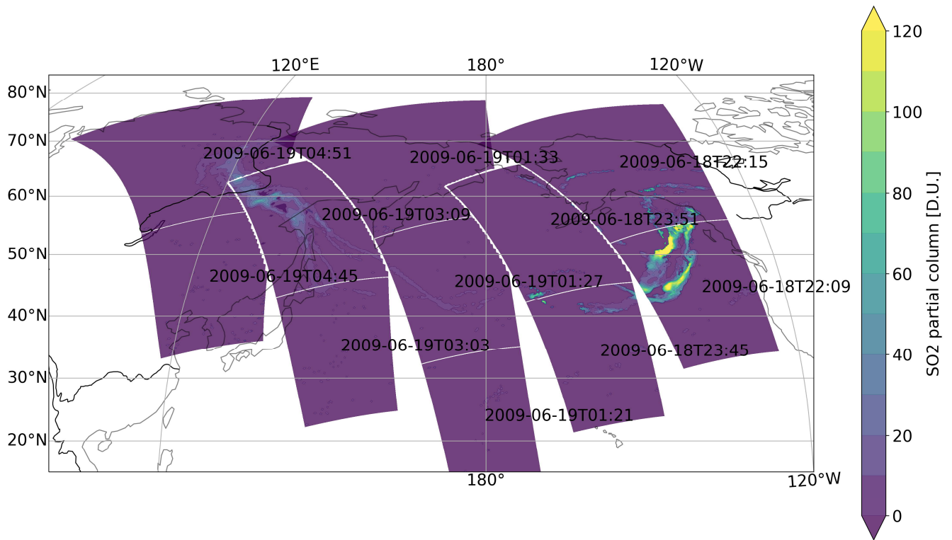
Figure 2: SO 2 partial column densities from AIRS swaths on the 18 th and 19 th of June. The total SO 2 mass is 1.09 Tg with no location counted more than once.
