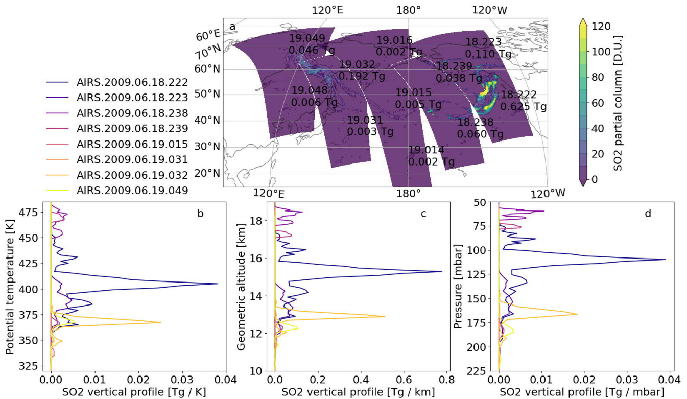
15 Figure 7: a) A collection of AIRS SO 2 swaths spanning the entire volcanic cloud. The SO 2 mass in the wedge of missing coverage between swaths 18.222, 18.238, 18.239 is estimated to be 0.036 Tg (3 % of the total mass). b-d) Height profiles for the AIRS swaths in the collection shown in a), in potential temperature (b), geometric altitude (c), and pressure (d). The number of CALIOP swaths that had air tracers transported into the SO 2 -swaths were: 18.222 (34 CALIOP swaths), 18.223 (34), 18.238 (17), 18.239 (25), 19.014
