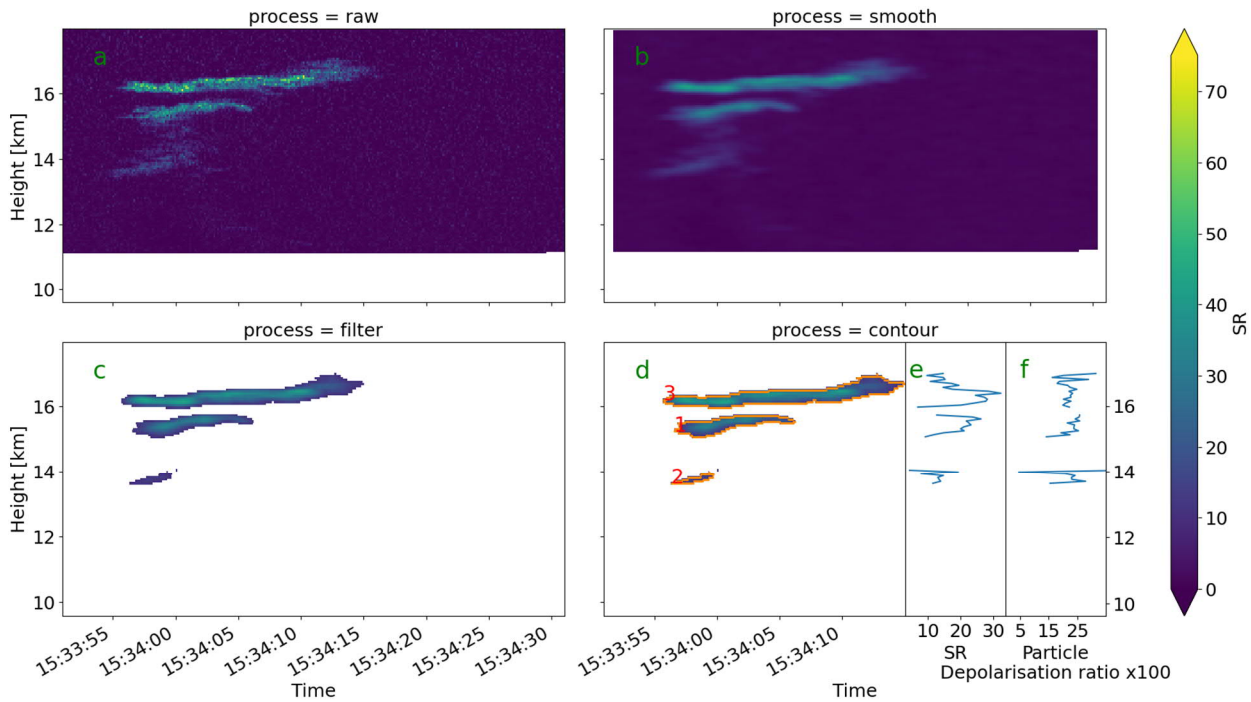
Figure 5: Example of how a volcanic cloud is located in a CALIOP swath and how it is prepped for RELEASES, a) the calculated scattering ratio from a level 1 CALIOP swath with pixels below the tropopause filtered away (white), b) the scattering ratio after smoothing has been applied, c) the smoothed scattering ratio after the scattering ratio threshold has been applied, d) sub-clouds 20
