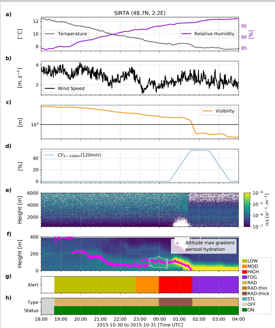
Figure 6: Time series presenting measurements and the corresponding retrieved alerts level outputs from PARAFOG-v2 during a thick radiation fog formation on 30-31 October 2015 at SIRTa. a) Temperature and relative humidity, b) wind speed, c) visibility, d) the Cloud Fraction (CF) between 0 and 1000 m over the last 2 hours, e) ALC-attenuated backscatter between 400 and 6000 m, f) ALC-attenuated backscatter between 0 and 400 m (color contours) together with the altitude of the maximum gradient (fuchsia points) and the aerosol hydration (gray contours), g) alert levels retrieved from PFG2, and h) fog type and PFG2 status.
