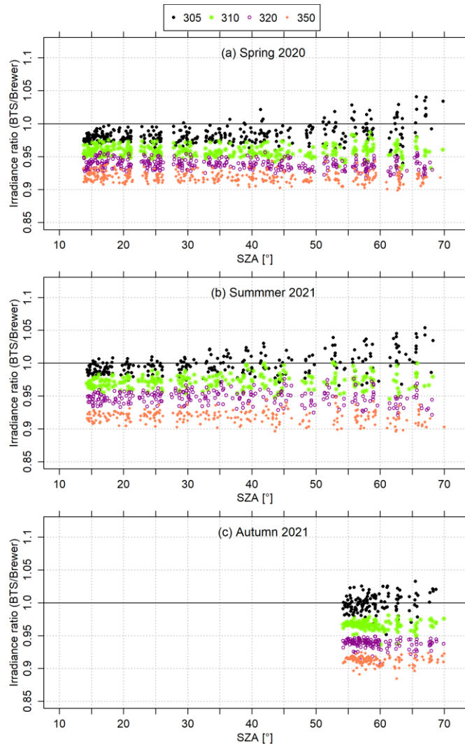
Figure 3: The ratios of global UV spectral irradiance at selected wavelengths between the BTS and the Brewer #150. The measurements were obtained from cloud-free conditions and SZAs below 70^\circ during (a) spring 2020, (b) summer 2021 and (c) autumn 2021. Each data point is calculated from the average over a \pm 2.5 nm wavelength band.
