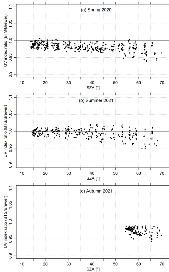
Figure 4: The ratio of UV indices between the BTS and the Brewer #150, as a function of solar zenith angle. The measurements were obtained from cloud-free conditions and SZAs lower than 70° during (a) spring 2020, (b) summer 2021 and (c) autumn 2021.
