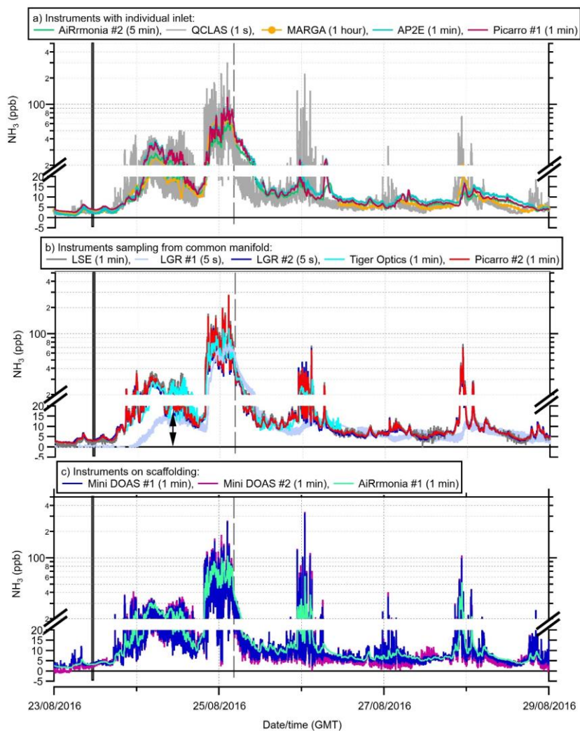
Figure 3. Summary of the reported concentrations from the instruments divided into categories a) instruments with individual inlet set-up b) instruments subsampling from the manifold and c) instruments on scaffolding. Number in brackets is the reporting time resolution of each instrument. The thick black line is the fertilisation of both fields, the grey dashed line indicates the change in wind direction at 04:00 on the 25/08 and the black arrow indicates the point at which the laser position was changed on the LGR #1. Note: The scale changes at 20 ppb to a log scale. (Supplementary Figures plotting the data on linear scale can be found in Figure S1).
