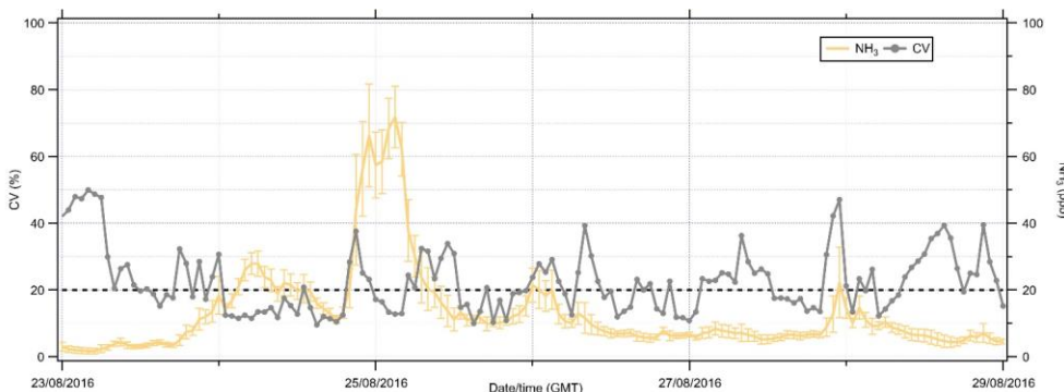
Figure 6. Time series hourly averages of the coefficient of variance (CV) and the average reported NH 3 concentration (ppb), where error bars are \pm \sigma_A . The black dotted line is a CV limit of 20%.
