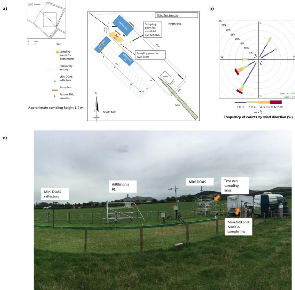
Figure 1. a) Layout of field site b) wind rose of wind direction and wind speed for the period 23 rd August to 29 th August ( Generated using OpenAir package in R (Carslaw and Ropkins, 2012) and c) photo of setup instruments (photo credit: M.
