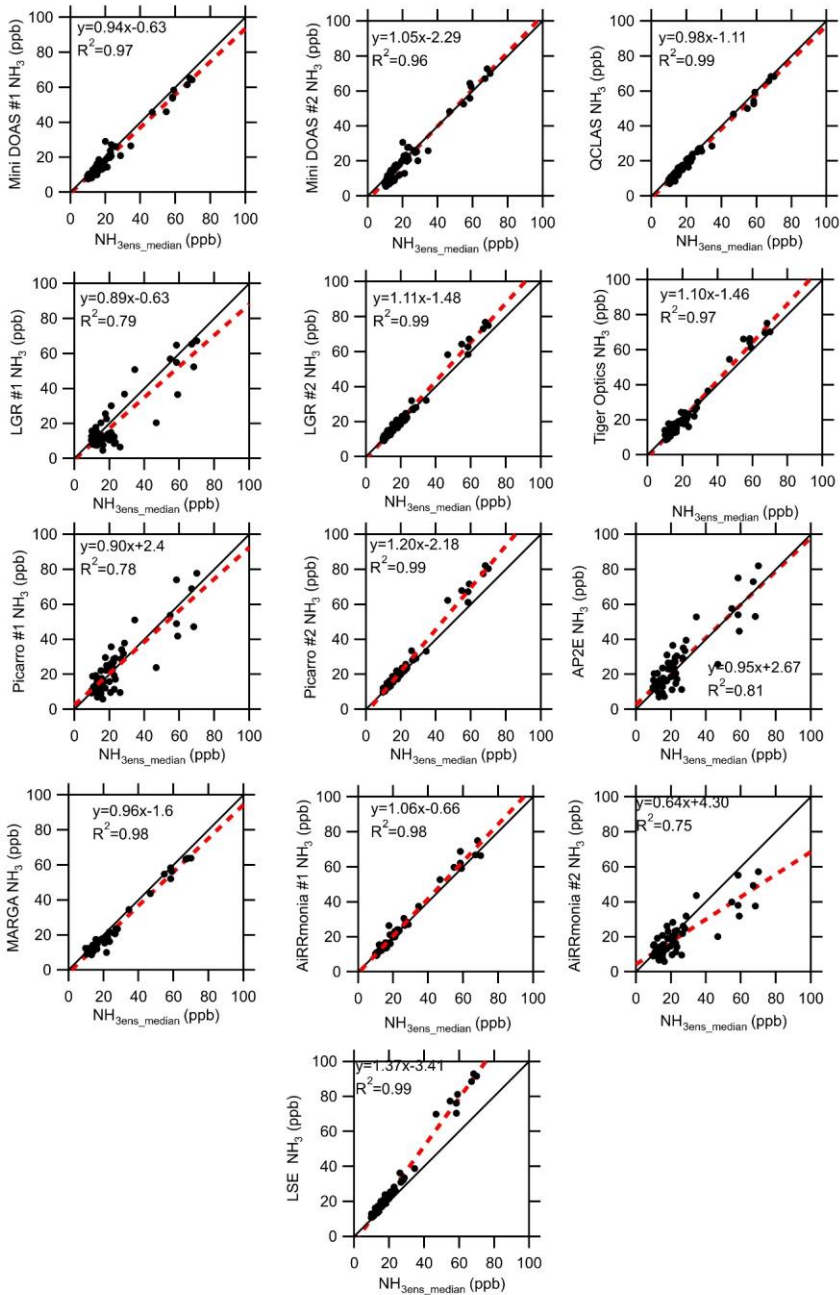
Figure 9. Intercomparison of instruments (hourly) averages from 22/08/2016 to 29/08/2016 to the ensemble median (excluding LGR #1 and Tiger Optics) when the median is equal or greater to 10 ppb \text{NH}_3 . Data were filtered for low wind speed and stable/unstable conditions that could have led to inhomogeneity at the site. The solid black line is the 1:1 line and red dashed line is the fit.
